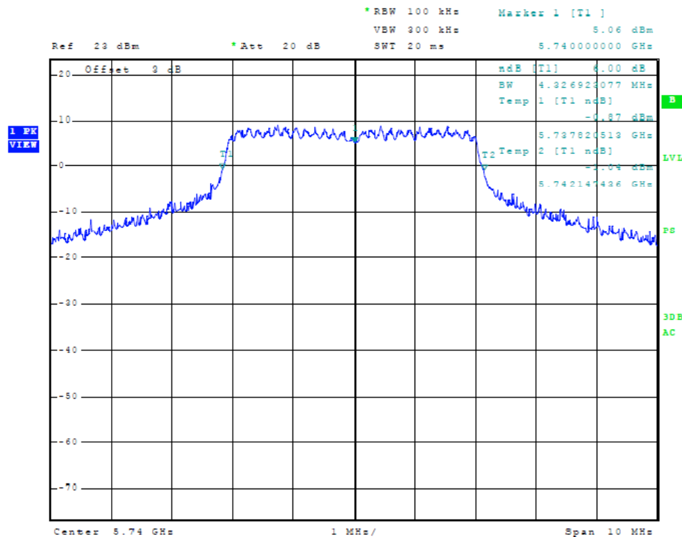
Figure Sixteen Plot of Plot of 6dB Band width (Chain 1, 5 MHz Mode, 5740 MHz)
