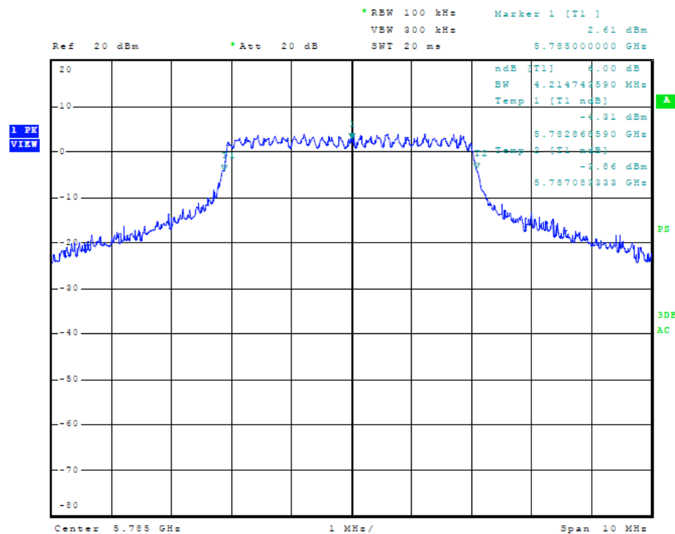
Figure Seventeen Plot of Plot of 6dB Band width (Chain 1, 5 MHz Mode, 5785 MHz)
