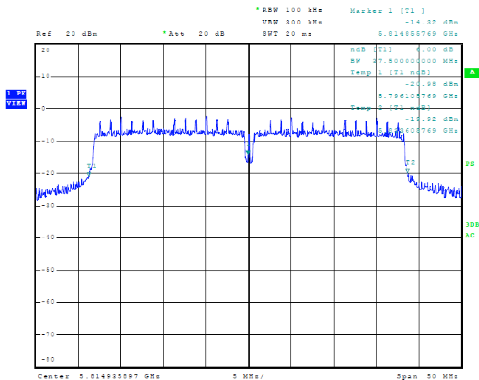
Figure Twenty-four Plot of 6dB Band width (Chain 1, 40 MHz Mode, 5815 MHz)
