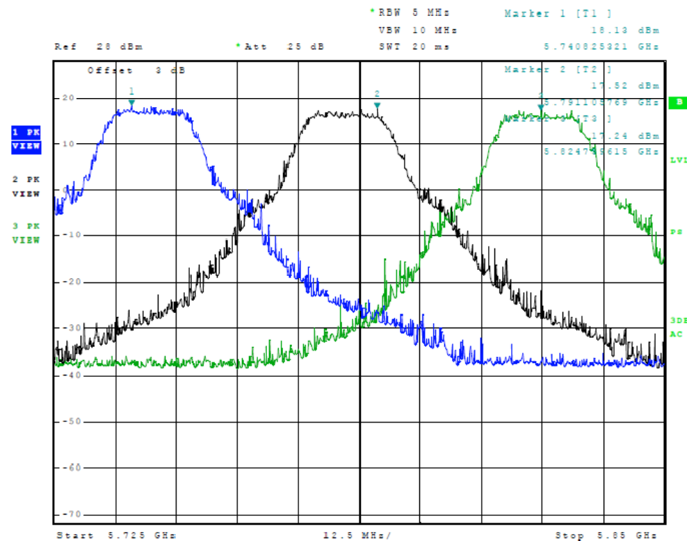
Figure Fourteen Plot of Radiated Emissions (Across Operational Band, 20MHz Mode)
