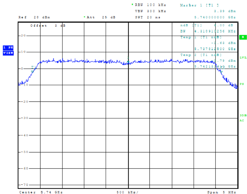
Figure Thirty-four Plot of Plot of 6dB Band width (Chain 2, 5 MHz Mode, 5740 MHz)
