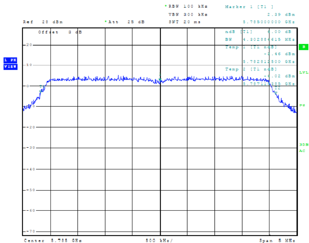
Figure Thirty-five Plot of Plot of 6dB Band width (Chain 2, 5 MHz Mode, 5785 MHz)
