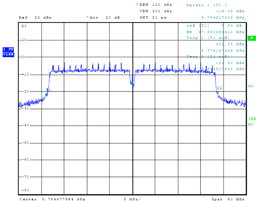
Figure Twenty-three Plot of 6dB Band width (Chain 1, 40 MHz Mode, 5795 MHz)
