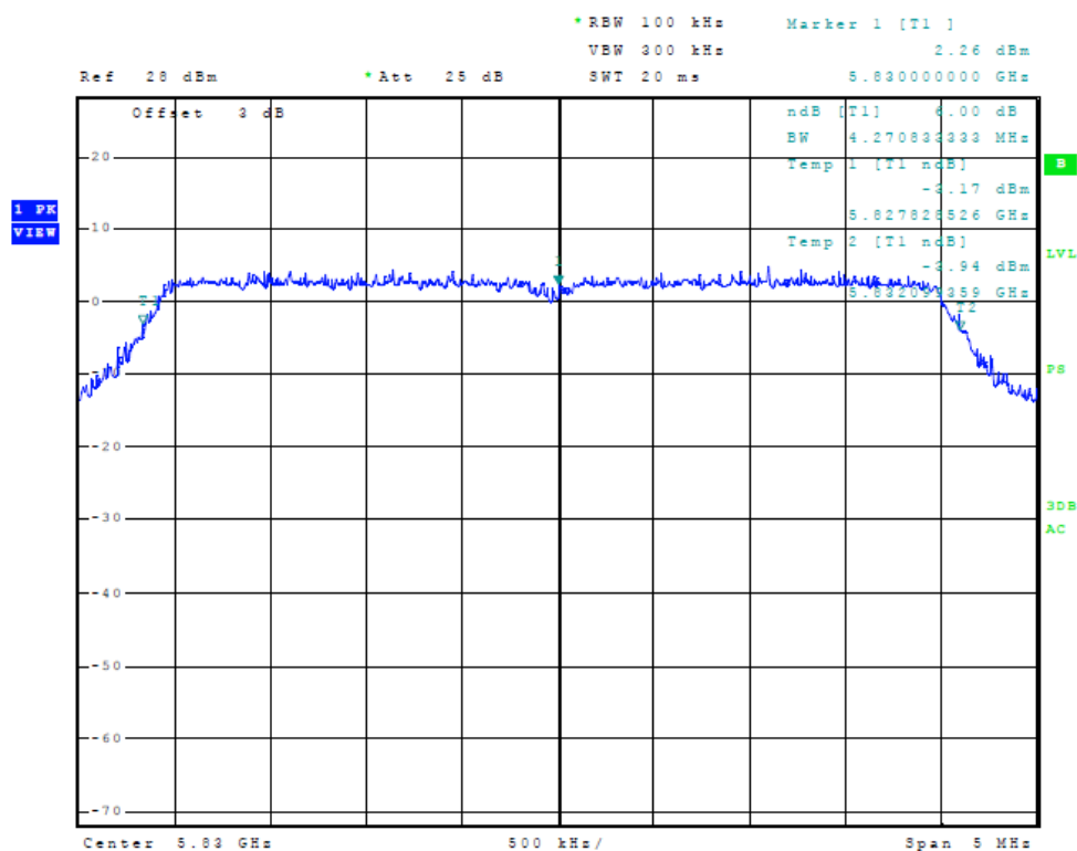
Figure Thirty-six Plot of Plot of 6dB Band width (Chain 2, 5 MHz Mode, 5830 MHz)
