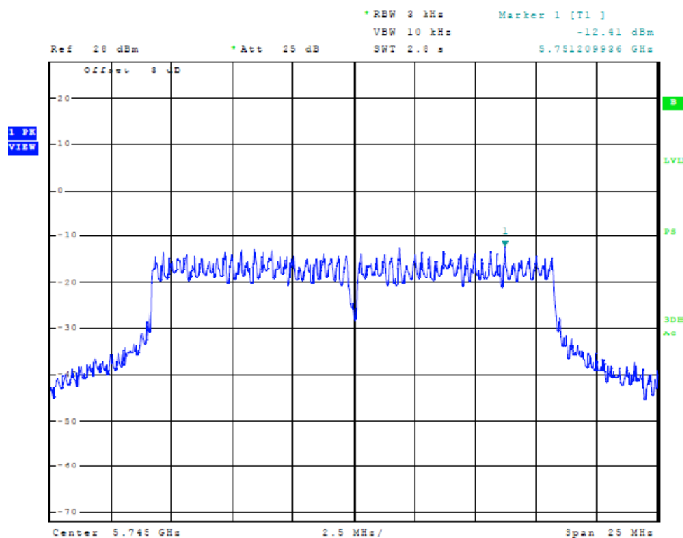
Figure Forty-six Plot of Power Spectral Density (Chain 2, 20 MHz Mode, 5745 MHz)
