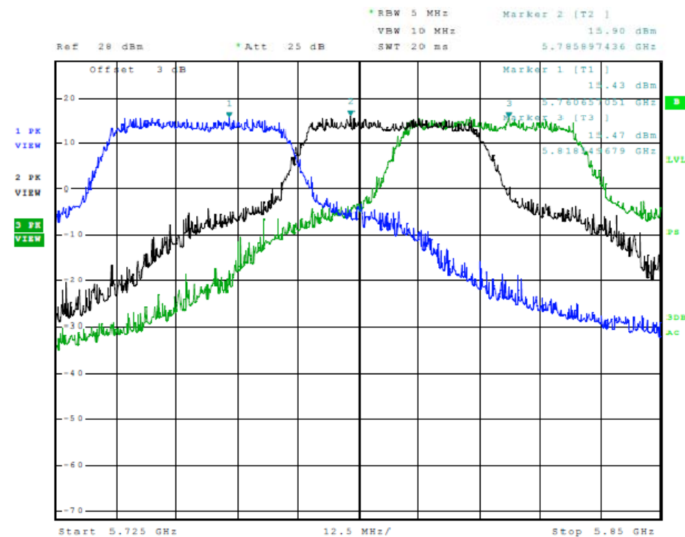
Figure Fifteen Plot of Radiated Emissions (Across Operational Band, 40MHz Mode)
