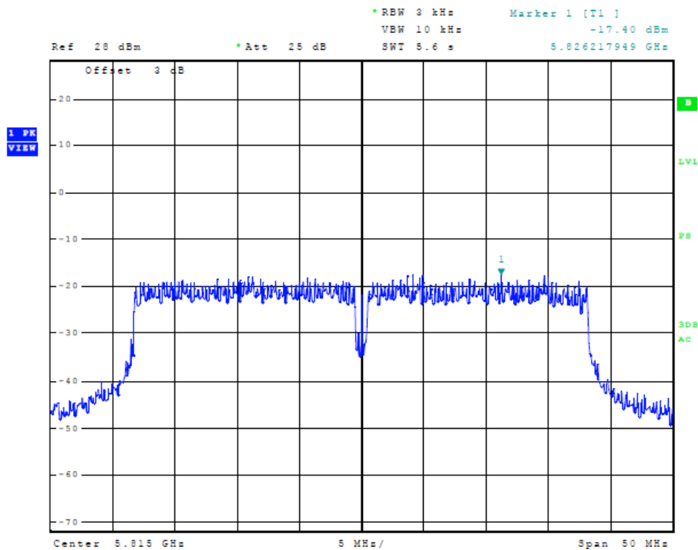
Figure Fifty-one Plot of Power Spectral Density (Chain 2, 40 MHz Mode, 5815 MHz)
