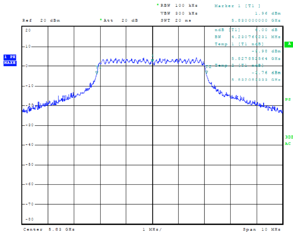
Figure Eighteen Plot of Plot of 6dB Band width (Chain 1, 5 MHz Mode, 5830 MHz)
