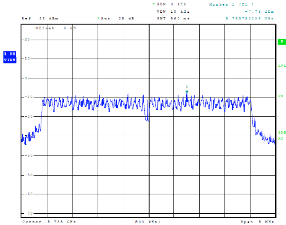
Figure Forty-four Plot of Power Spectral Density (Chain 2, 5 MHz Mode, 5785 MHz)
