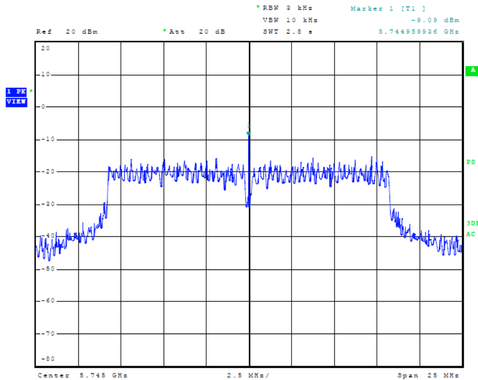
Figure Twenty-eight Plot of Power Spectral Density (Chain 1, 20 MHz Mode, 5745 MHz)
