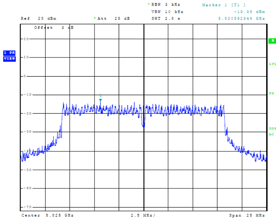
Figure Forty-eight Plot of Power Spectral Density (Chain 2, 20 MHz Mode, 5825 MHz)
