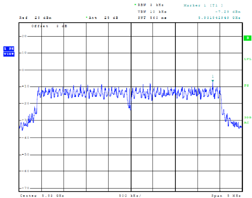
Figure Forty-five Plot of Power Spectral Density (Chain 2, 5 MHz Mode, 5830 MHz)
