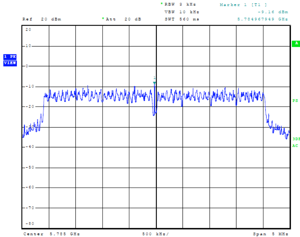
Figure Twenty-six Plot of Power Spectral Density (Chain 1, 5 MHz Mode, 5785 MHz)
