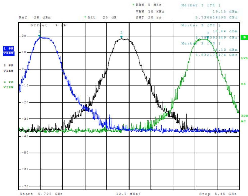
Figure Thirteen Plot of Radiated Emissions (Across Operational Band, 10MHz Mode)
