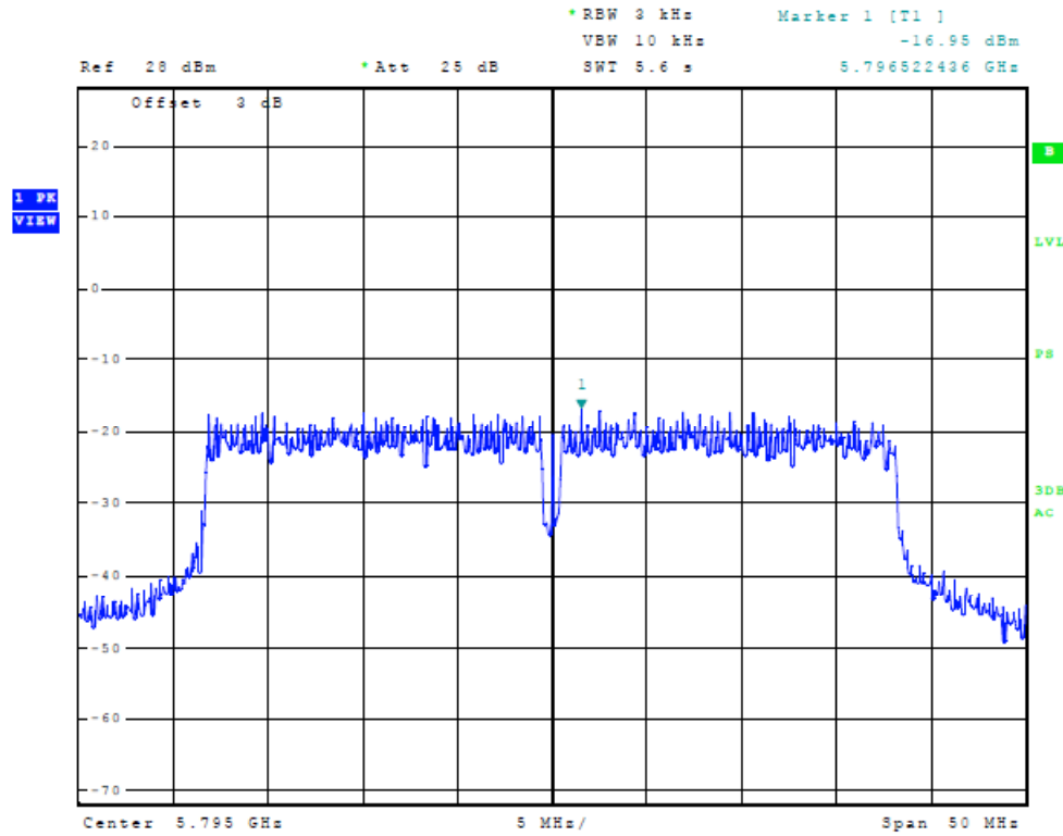
Figure Fifty Plot of Power Spectral Density (Chain 2, 40 MHz Mode, 5795 MHz)
