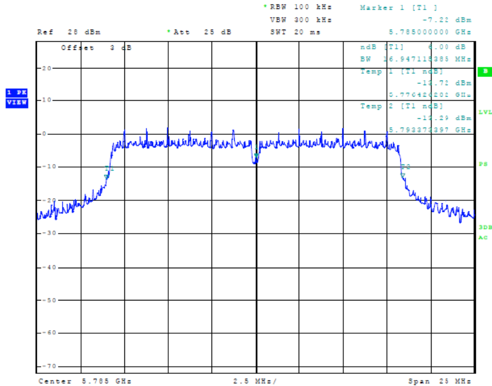
Figure Thirty-eight of 6dB Band width (Chain 2, 20 MHz Mode, 5785 MHz)
