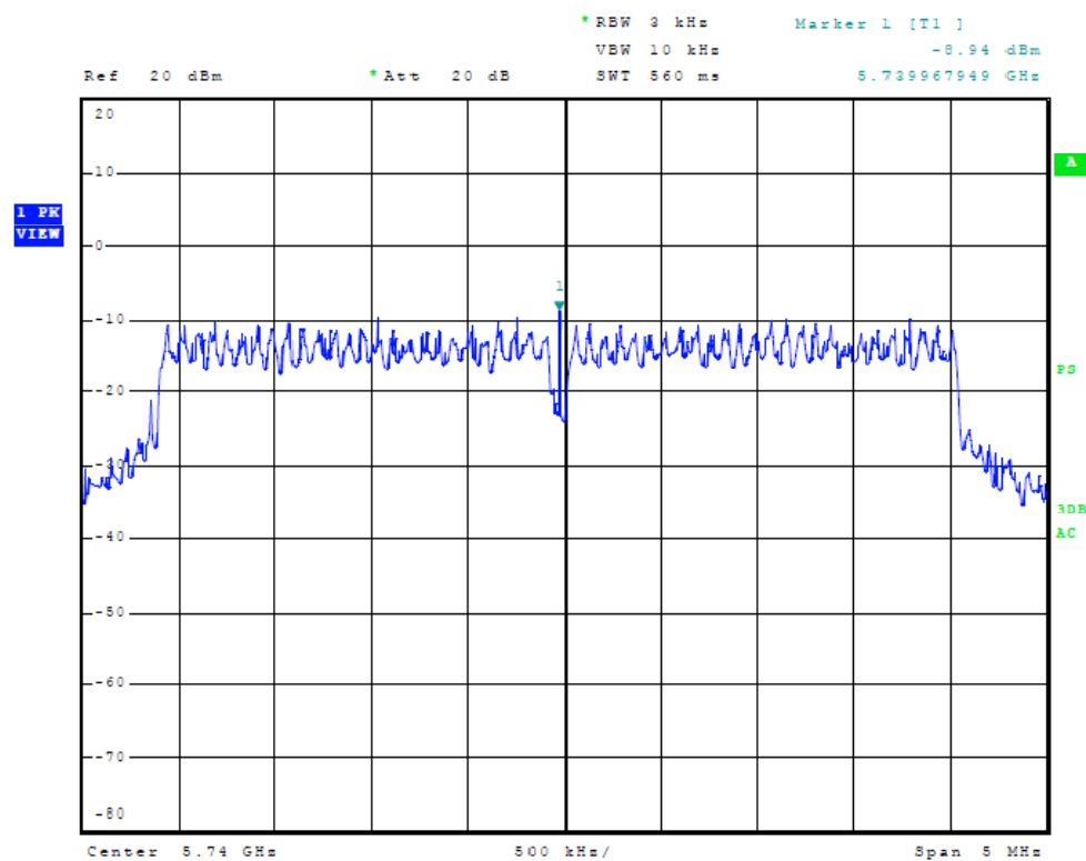
Figure Twenty-five Plot of Power Spectral Density (Chain 1, 5 MHz Mode, 5740 MHz)
