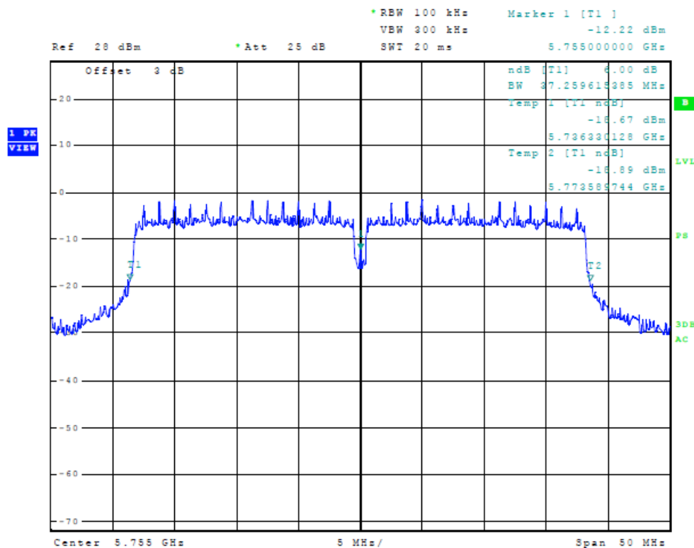
Figure Forty Plot of 6dB Band width (Chain 2, 40 MHz Mode, 5755 MHz)
