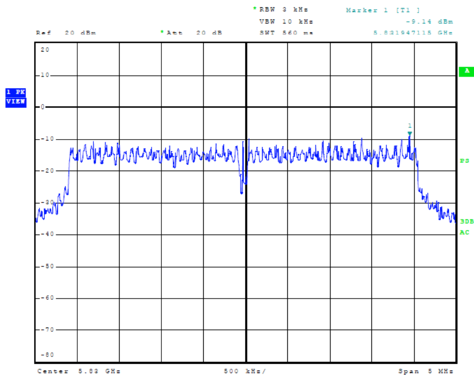
Figure Twenty-seven Plot of Power Spectral Density (Chain 1, 5 MHz Mode, 5830 MHz)
