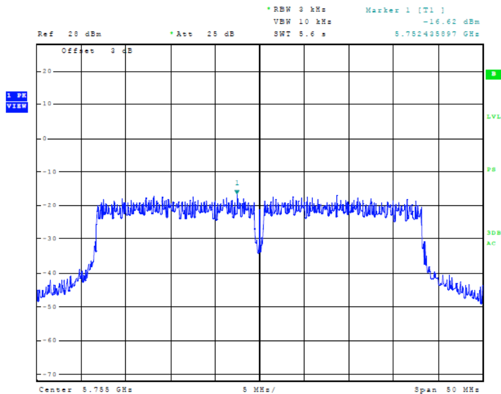
Figure Forty-nine Plot of Power Spectral Density (Chain 2, 40 MHz Mode, 5755 MHz)
