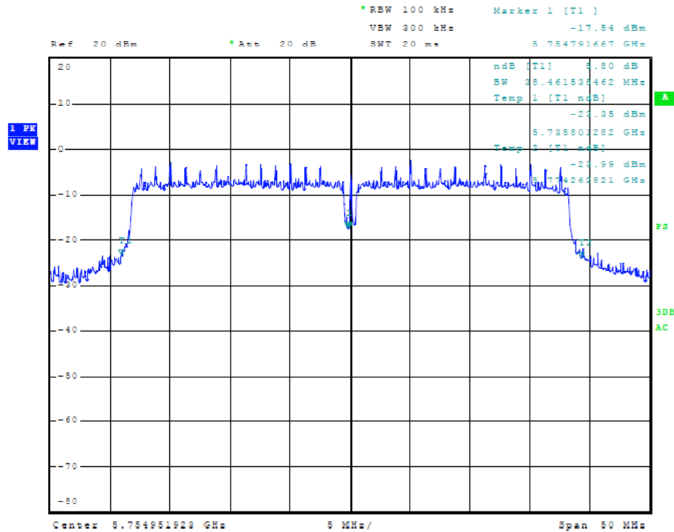
Figure Twenty-two Plot of 6dB Band width (Chain 1, 40 MHz Mode, 5755 MHz)
