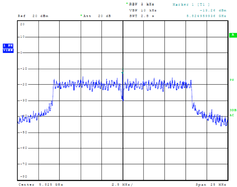
Figure Thirty Plot of Power Spectral Density (Chain 1, 20 MHz Mode, 5825 MHz)
