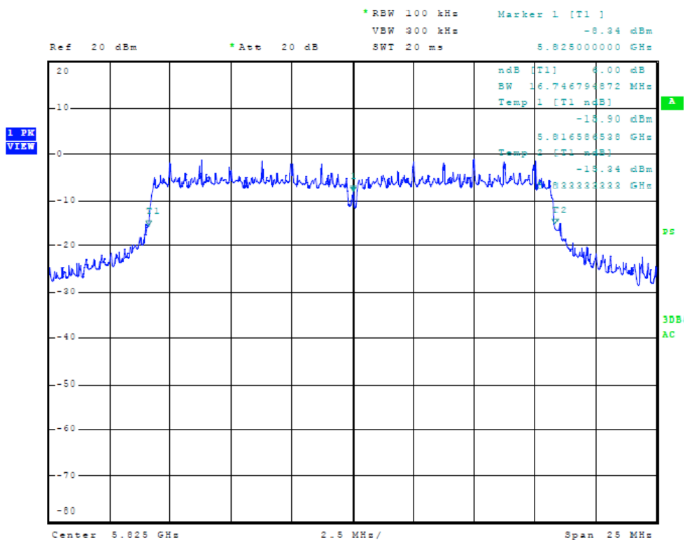
Figure Twenty-one Plot of 6dB Band width (Chain 1, 20 MHz Mode, 5825 MHz)
