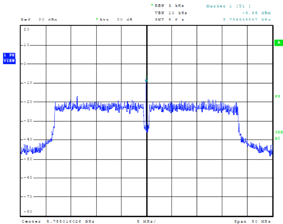
Figure Thirty-one Plot of Power Spectral Density (Chain 1, 40 MHz Mode, 5755 MHz)
