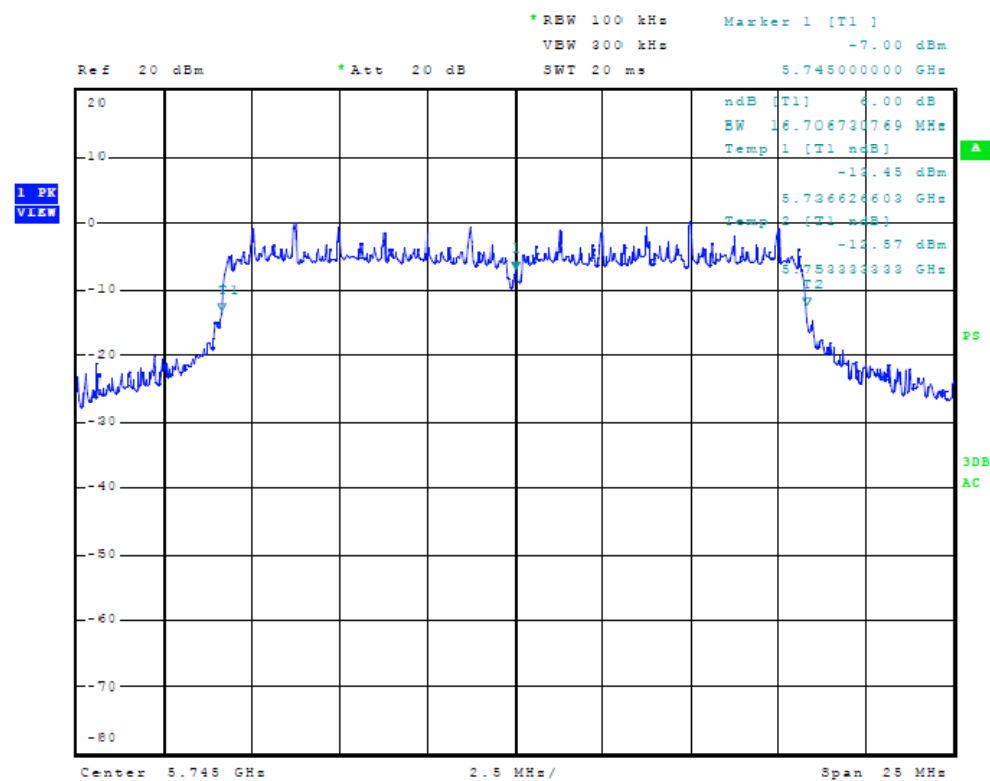
Figure Nineteen Plot of 6dB Band width (Chain 1, 20 MHz Mode, 5745 MHz)
