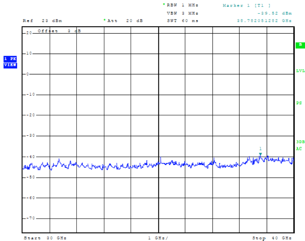
Figure Fifty-eight Plot of Antenna port conducted emissions
