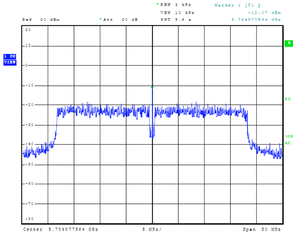
Figure Thirty-two Plot of Power Spectral Density (Chain 1, 40 MHz Mode, 5795 MHz)
