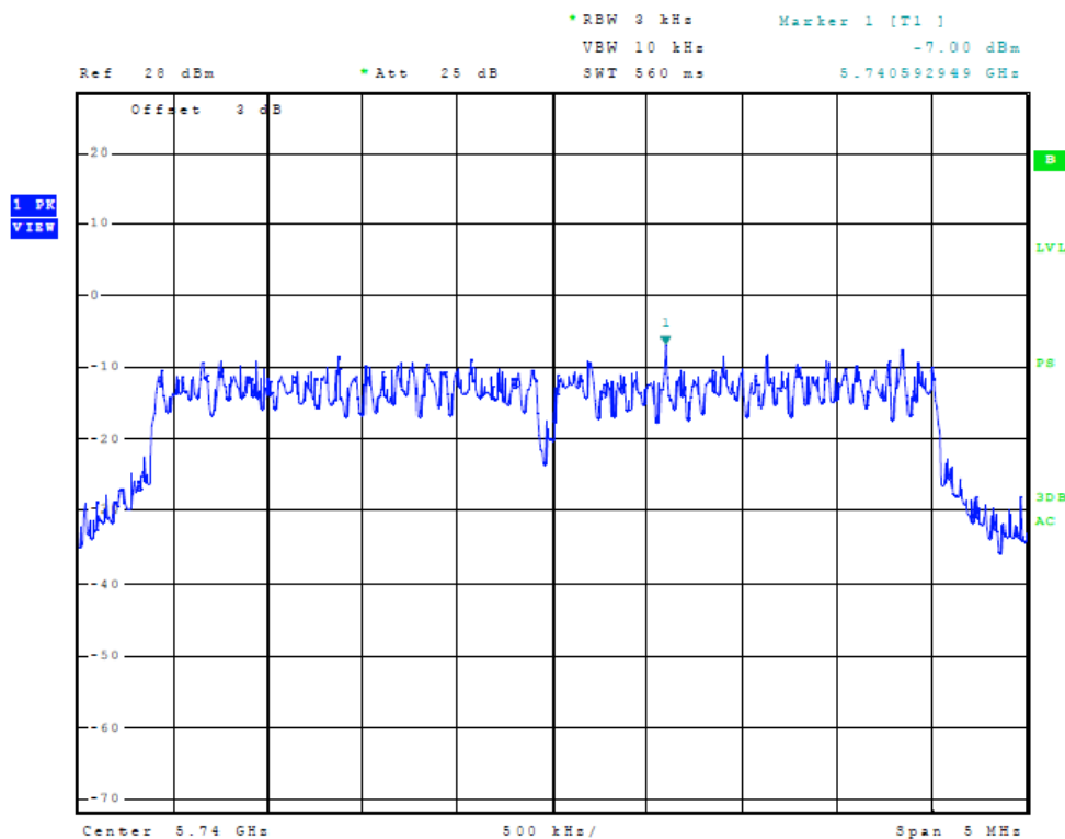
Figure Forty-three Plot of Power Spectral Density (Chain 2, 5 MHz Mode, 5740 MHz)
