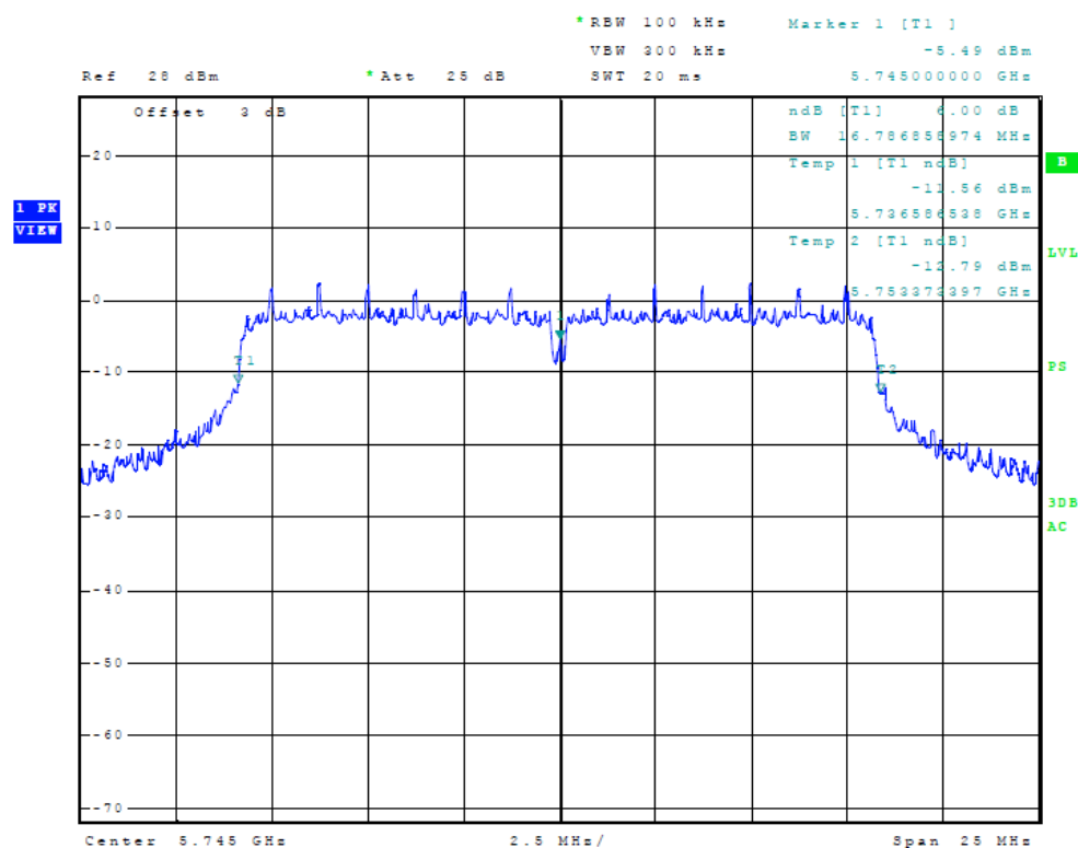
Figure Thirty-seven Plot of 6dB Band width (Chain 2, 20 MHz Mode, 5745 MHz)
