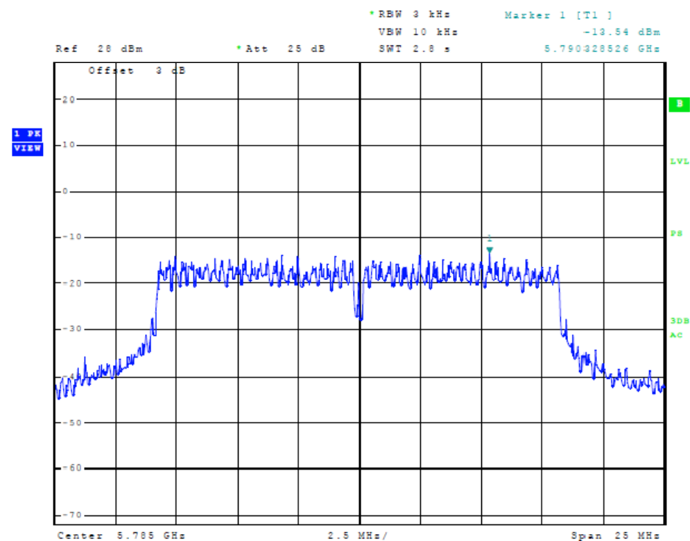
Figure Forty-seven Plot of Power Spectral Density (Chain 2, 20 MHz Mode, 5785 MHz)
