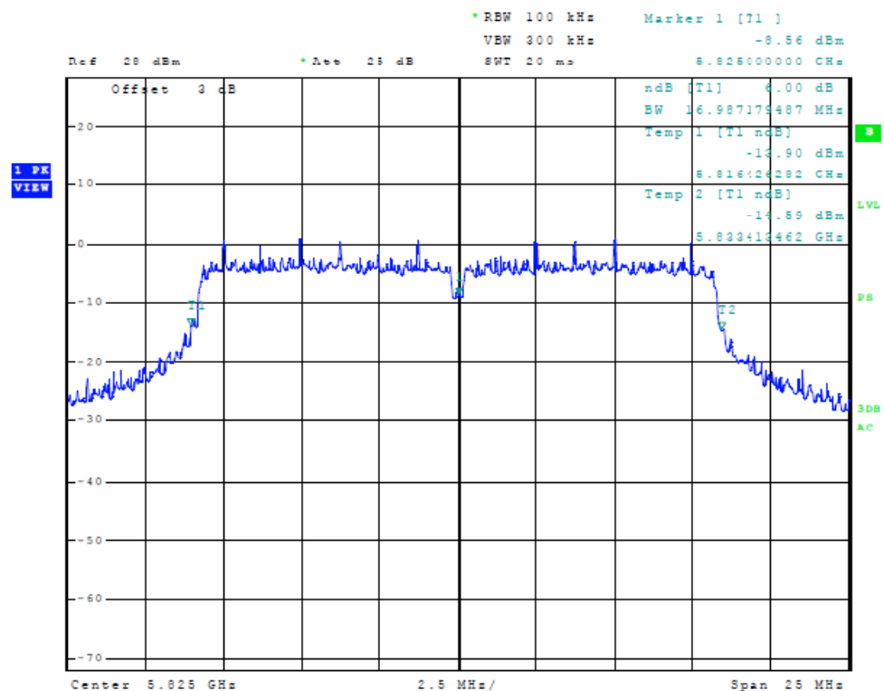
Figure Thirty-nine Plot of 6dB Band width (Chain 2, 20 MHz Mode, 5825 MHz)
