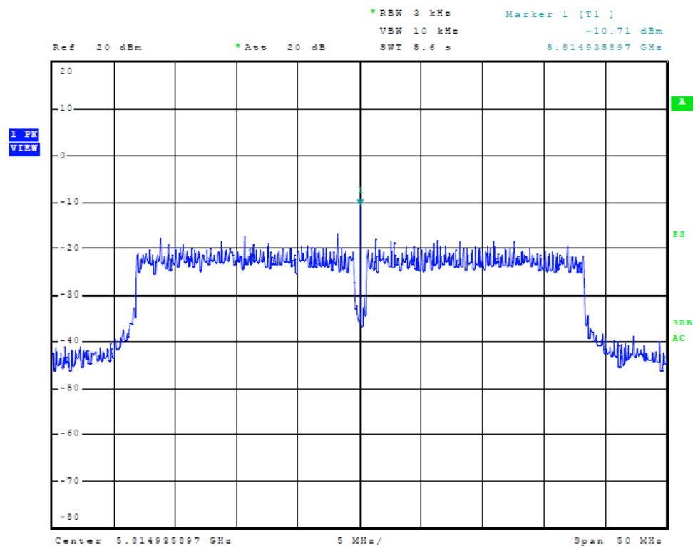
Figure Thirty-three Plot of Power Spectral Density (Chain 1, 40 MHz Mode, 5815 MHz)
