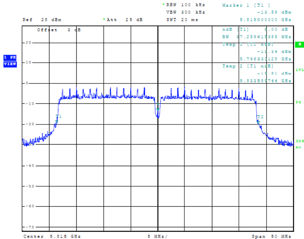
Figure Forty-two Plot of 6dB Band width (Chain 2, 40 MHz Mode, 5815 MHz)
