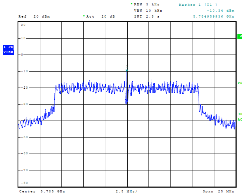
Figure Twenty-nine Plot of Power Spectral Density (Chain 1, 20 MHz Mode, 5785 MHz)
