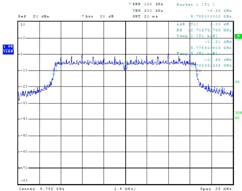
Figure Twenty of 6dB Band width (Chain 1, 20 MHz Mode, 5785 MHz)
