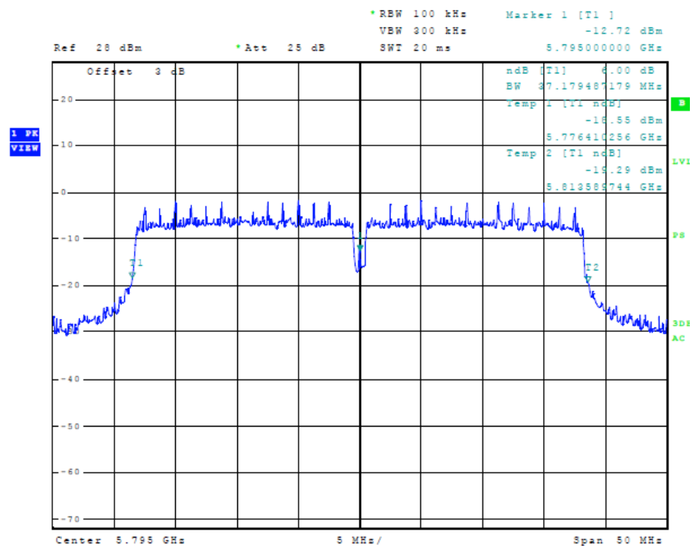
Figure Forty-one Plot of 6dB Band width (Chain 2, 40 MHz Mode, 5795 MHz)
