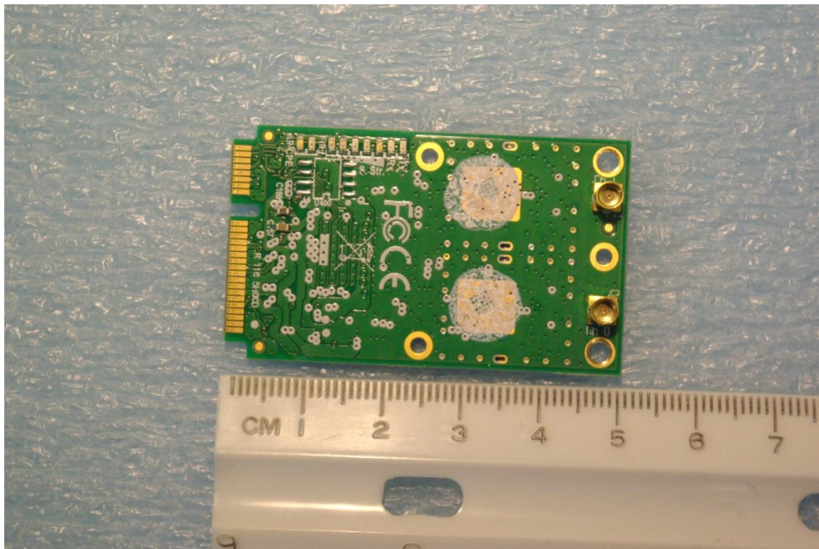
Back Side with heat sink removed
