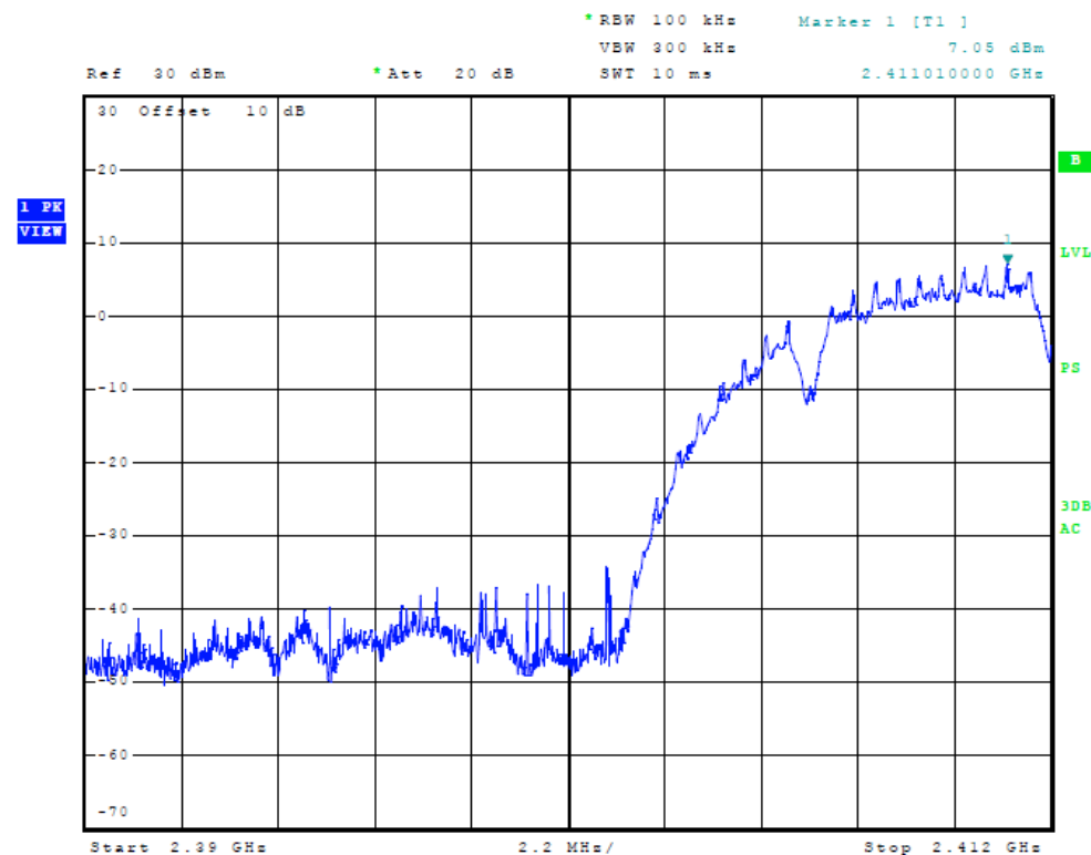
Figure Seven Plot of Low Band Edge (b/g/n Mode, chain 0)
