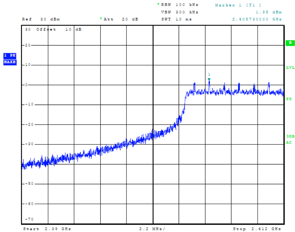
Figure Twelve Plot of Low Band Edge (n Mode, chain 1)
