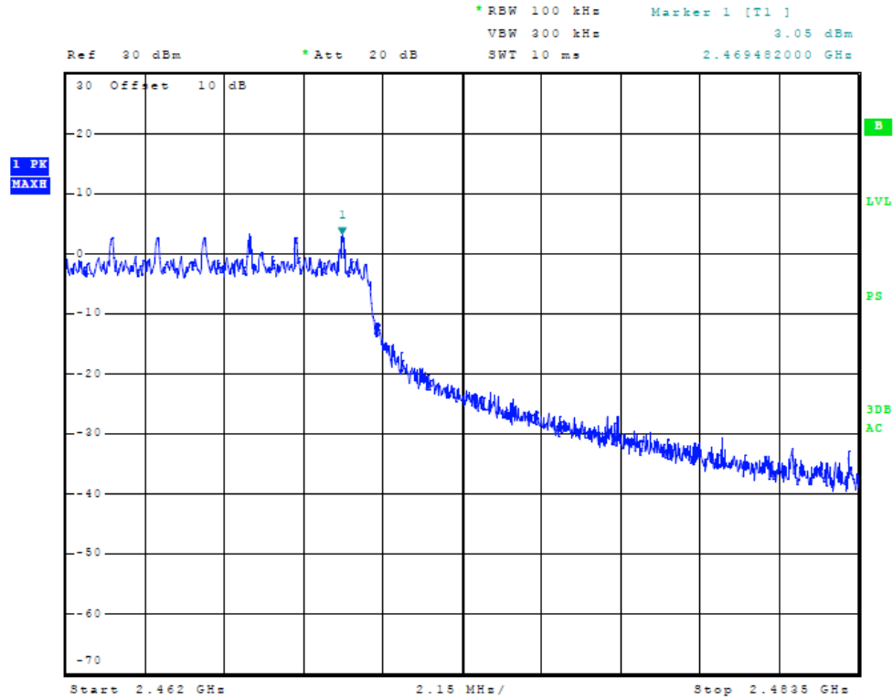
Figure Ten Plot of High Band Edge (n Mode, chain 0)
