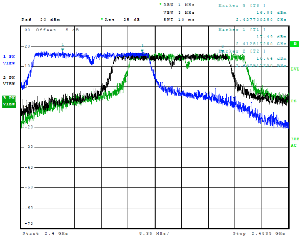
Figure Five Plot of Transmitter Emissions (Across Operational Band, n Mode, chain 0)
