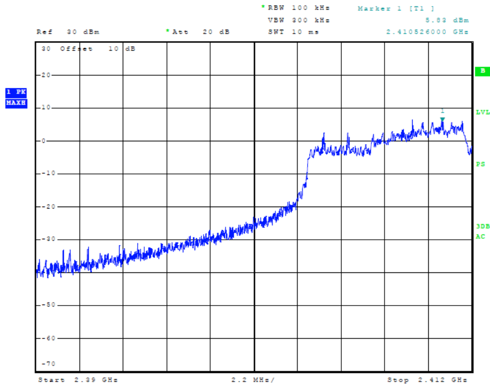
Figure Eight Plot of Low Band Edge (n Mode, chain 0)
