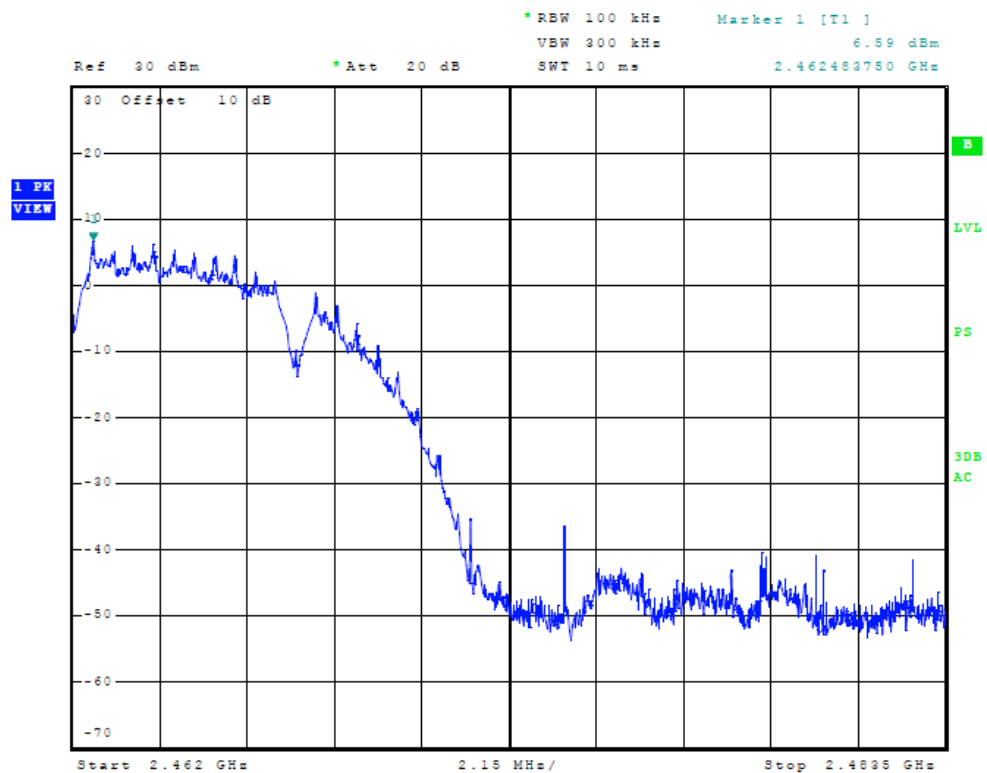
Figure Thirteen Plot of High Band Edge (b/g/n Mode, chain 1)
