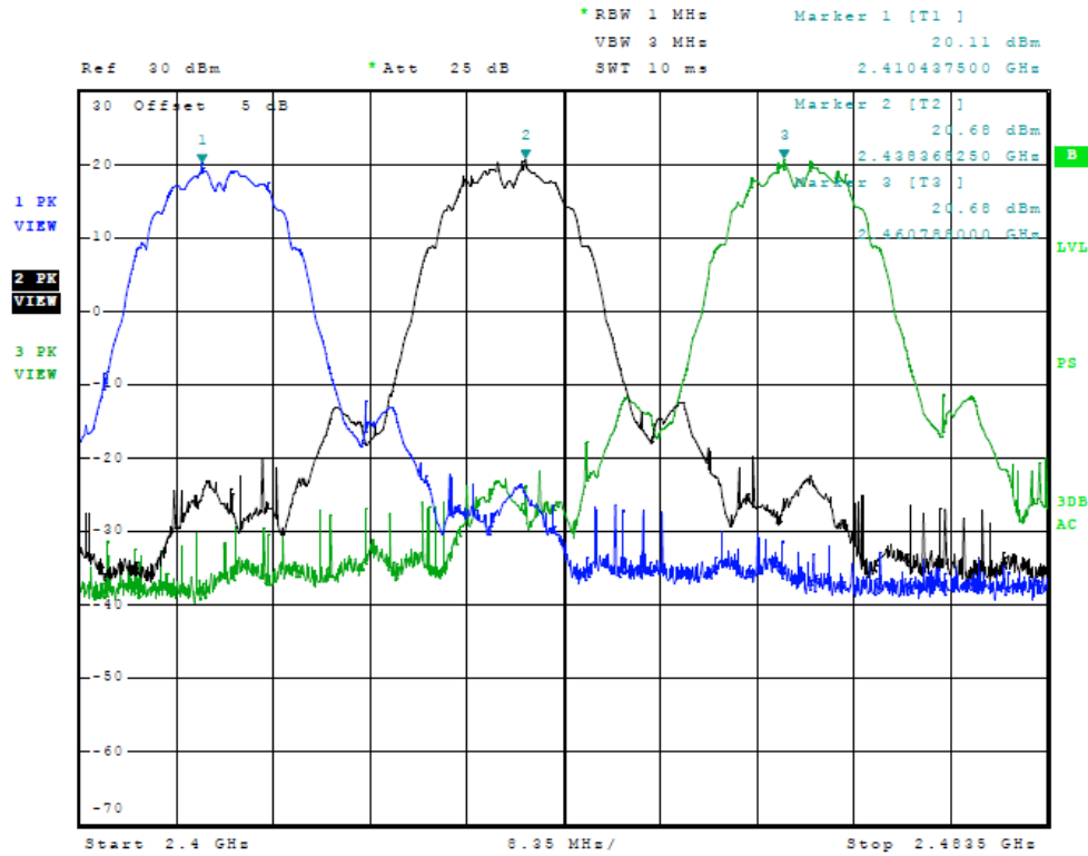
Figure Four Plot of Transmitter Emissions (Across Operational Band, b/g/n Mode, chain 1)
