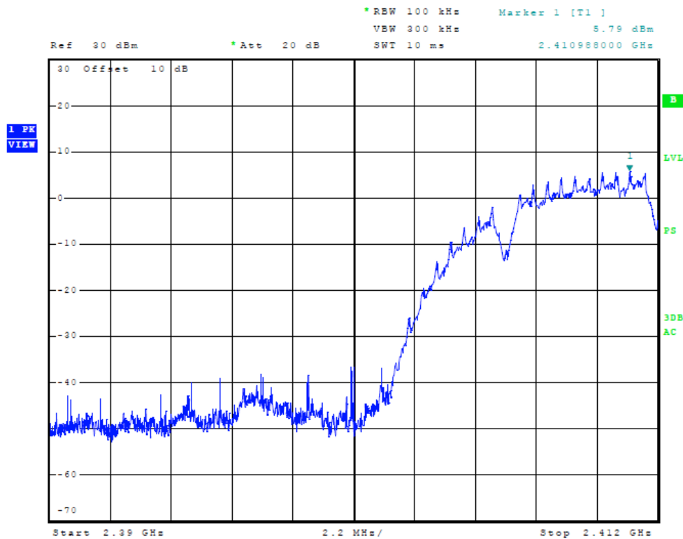
Figure Eleven Plot of Low Band Edge (b/g/n Mode, chain 1)
