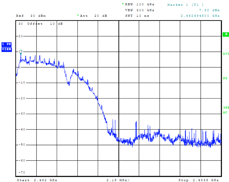
Figure Nine Plot of High Band Edge (b/g/n Mode, chain 0)
