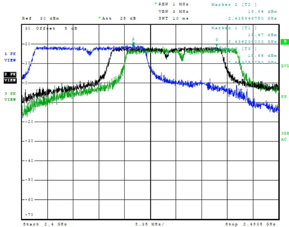
Figure Six Plot of Transmitter Emissions (Across Operational Band, n Mode, chain 1)
