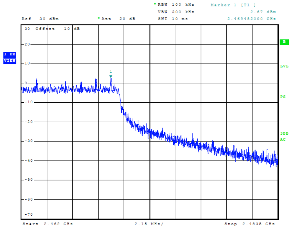
Figure Fourteen Plot of High Band Edge (n Mode, chain 1)
