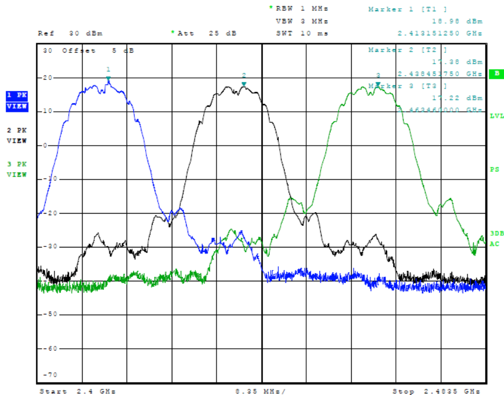
Figure Three Plot of Transmitter Emissions (Across Operational Band, b/g/n Mode, chain 0)
