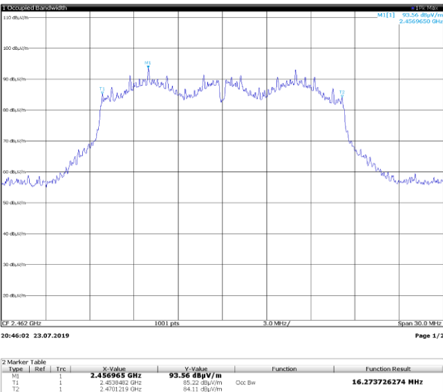
Figure 8.5-22: 99% bandwidth on 802.11g, sample plot
