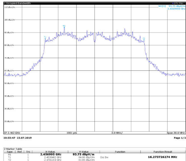
Figure 8.5-23: 99% bandwidth on 802.11n HT20, sample plot
