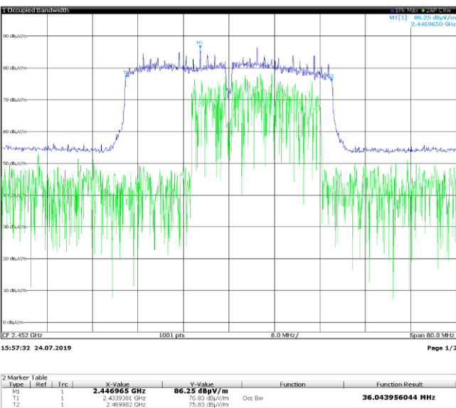
Figure 8.5-24: 99% bandwidth on 802.11n HT40, sample plot
