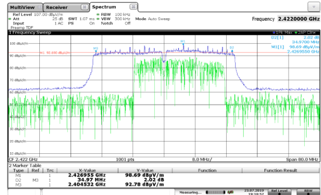
Figure 8.5-4: 6 dB bandwidth on 802.11n HT40, sample plot
