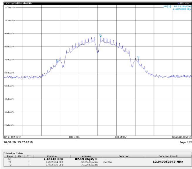
Figure 8.5-21: 99% bandwidth on 802.11b, sample plot
