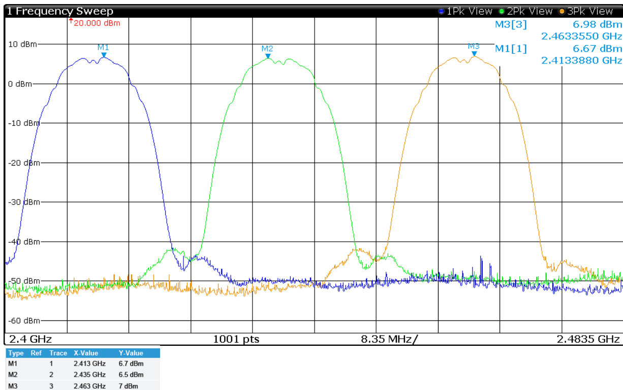
Figure 4 Plot of Transmitter Emissions (Across Operational Band 802.11b, Chain 1)
