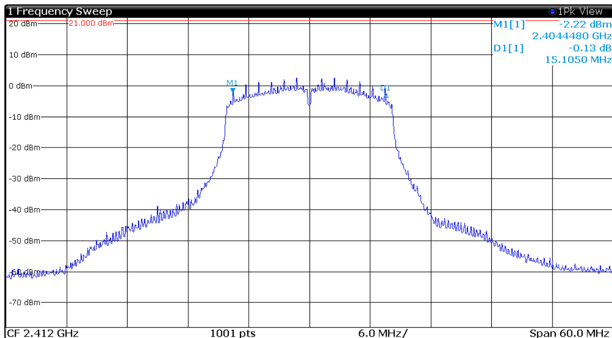
Figure 31 Plot of Transmitter 6-dB Occupied Band Width (802.11n (20), Chain 0)
