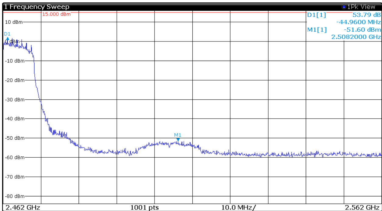
Figure 26 Plot of Transmitter High Band Edge (802.11n (40), Chain 1)
