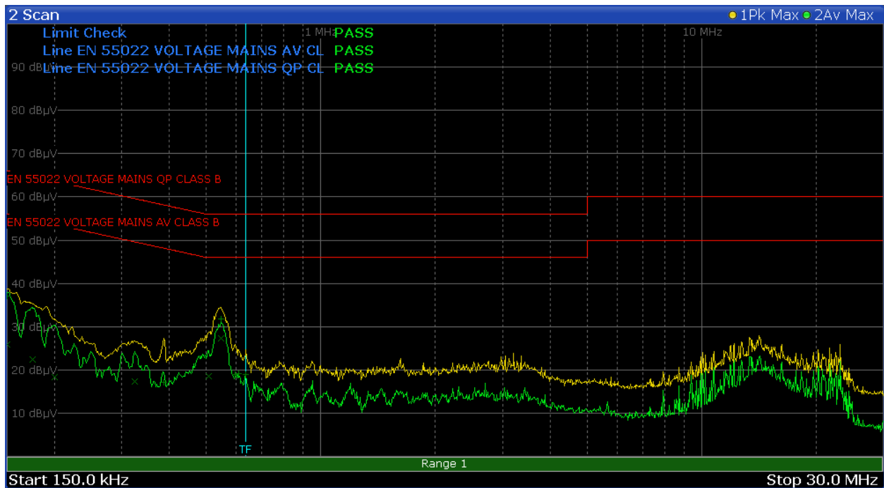
Figure 1 AC Line Conducted Emissions Line 1
