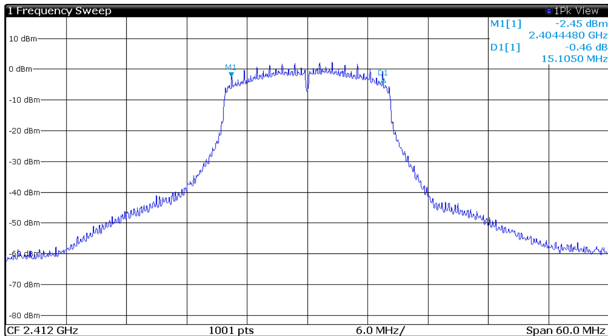
Figure 32 Plot of Transmitter 6-dB Occupied Band Width (802.11n (20), Chain 1)
