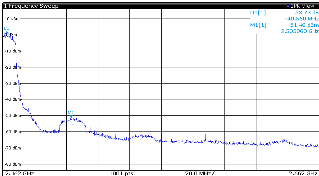
Figure 23 Plot of Transmitter High Band Edge (802.11n (20), Chain 0)
