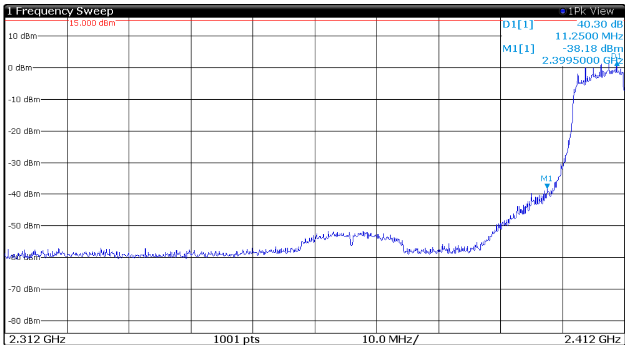
Figure 16 Plot of Transmitter Low Band Edge (802.11n (20), Chain 1)
