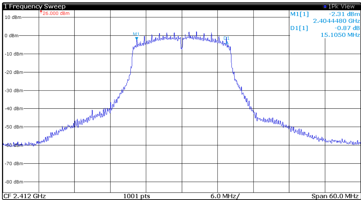
Figure 30 Plot of Transmitter 6-dB Occupied Band Width (802.11g, Chain 1)
