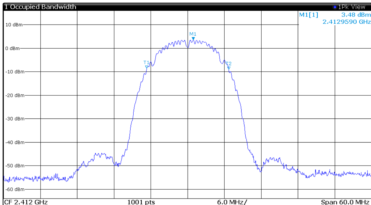
Figure 35 Plot of Transmitter 99% Occupied Band Width (802.11b, Chain 0)
