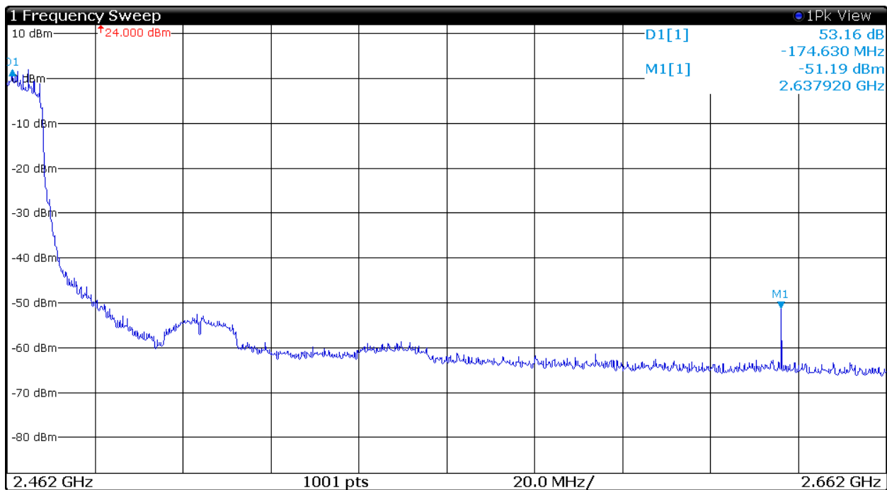
Figure 22 Plot of Transmitter High Band Edge (802.11g, Chain 1)
