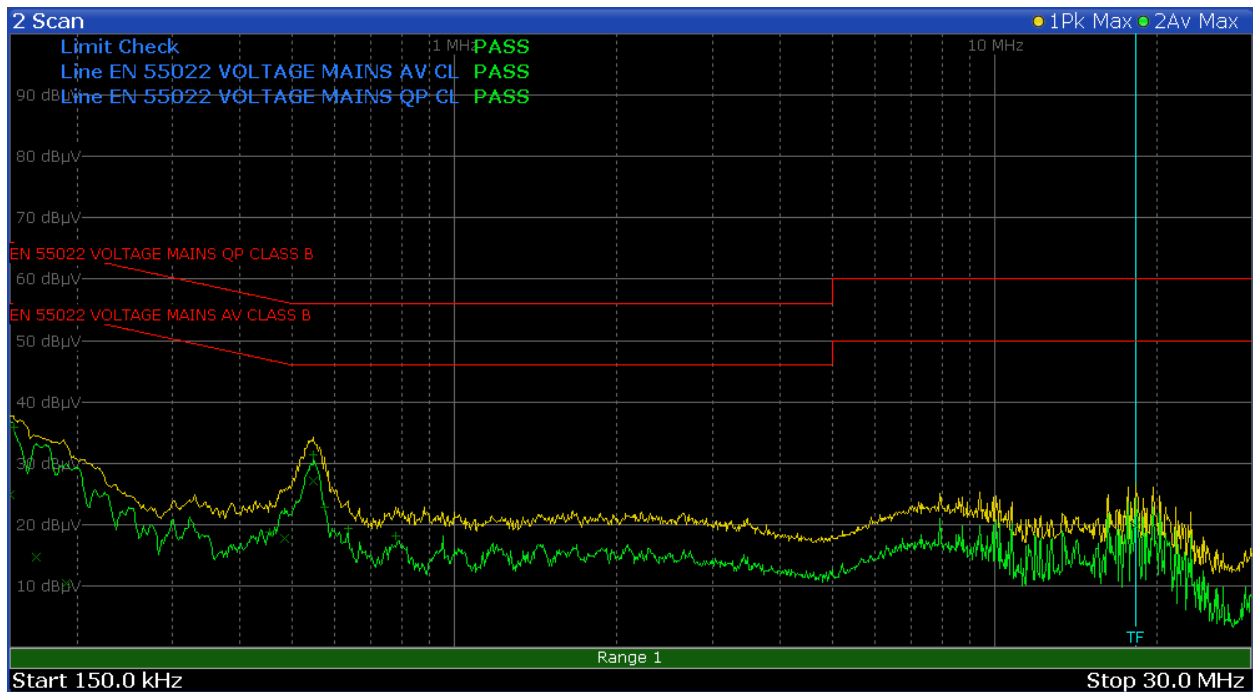
Figure 2 AC Line Conducted Emissions Line 2
