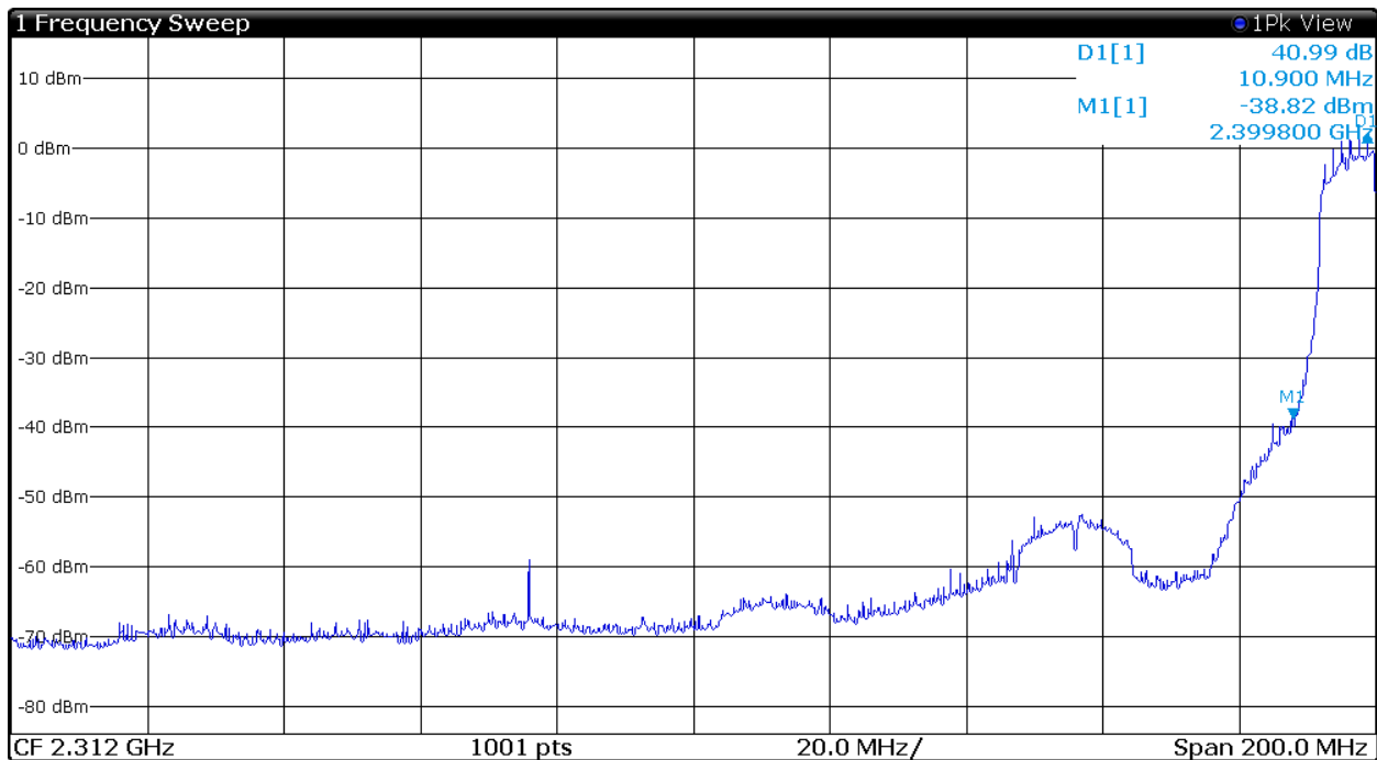
Figure 13 Plot of Transmitter Low Band Edge (802.11g, Chain 0)
