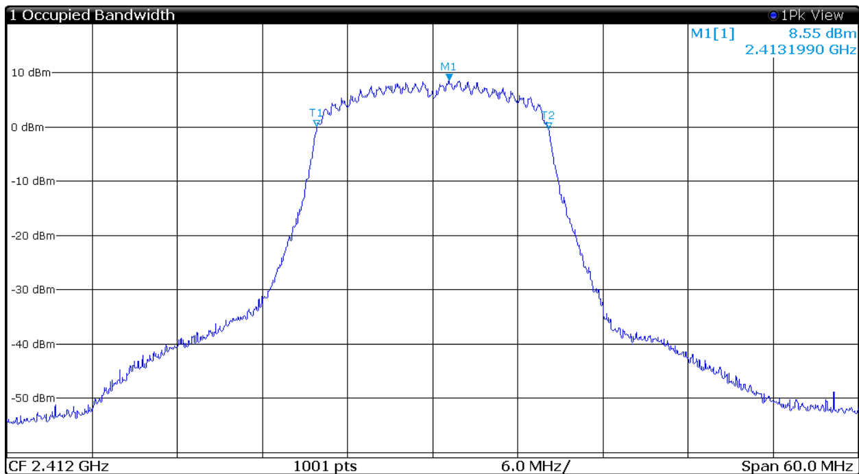
Figure 40 Plot of Transmitter 99% Occupied Band Width (802.11n (20), Chain 1)
