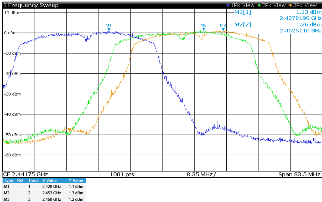
Figure 10 Plot of Transmitter Emissions (Across Operational Band, 802.11n (40), Chain 1)
