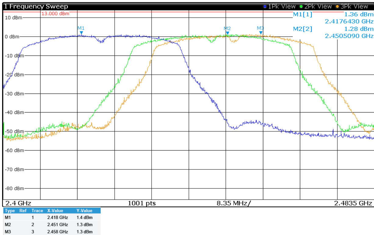
Figure 9 Plot of Transmitter Emissions (Across Operational Band, 802.11n (40), Chain 0)
