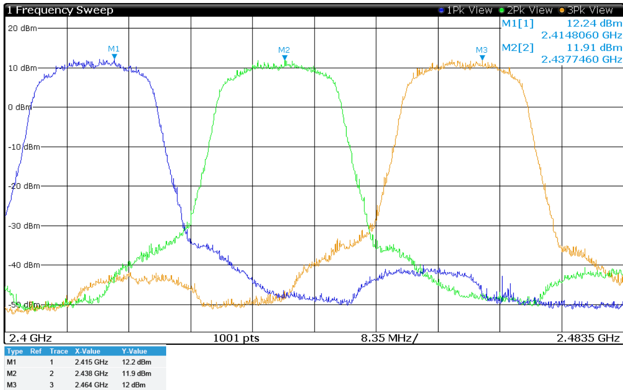
Figure 8 Plot of Transmitter Emissions (Across Operational Band, 802.11n (20), Chain 1)
