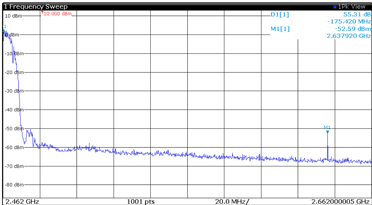
Figure 20 Plot of Transmitter High Band Edge (802.11b, Chain 1)
