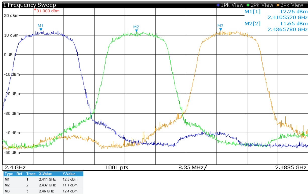
Figure 6 Plot of Transmitter Emissions (Across Operational Band, 802.11g, Chain 1)
