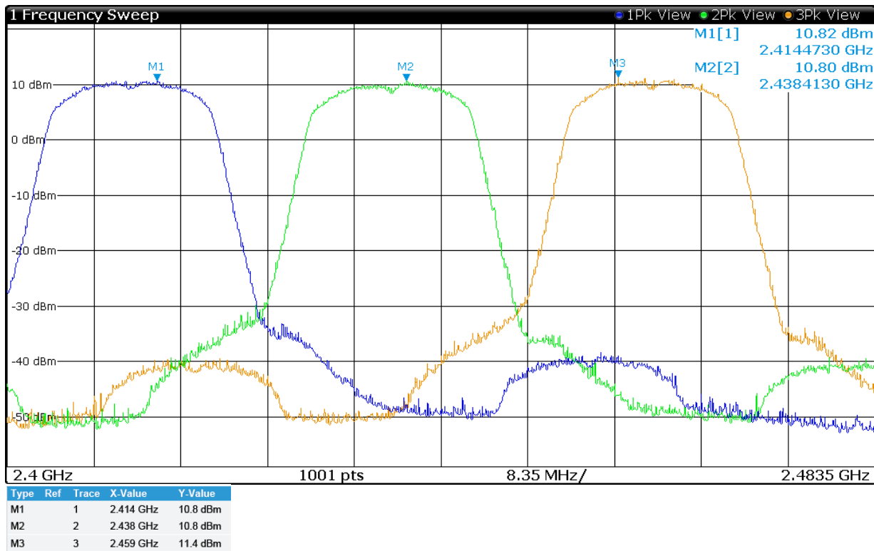
Figure 5 Plot of Transmitter Emissions (Across Operational Band, 802.11g, Chain 0)
