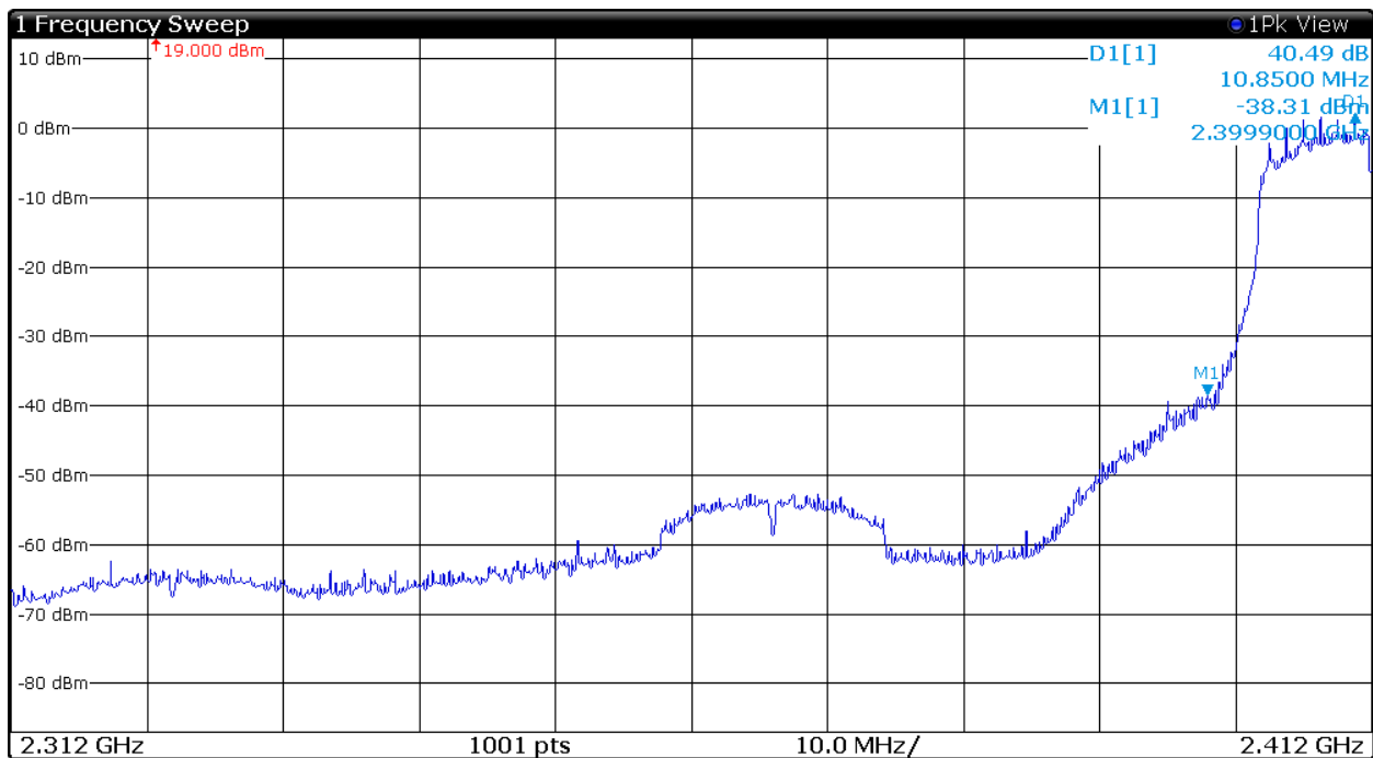
Figure 14 Plot of Transmitter Low Band Edge (802.11g, Chain 1)
