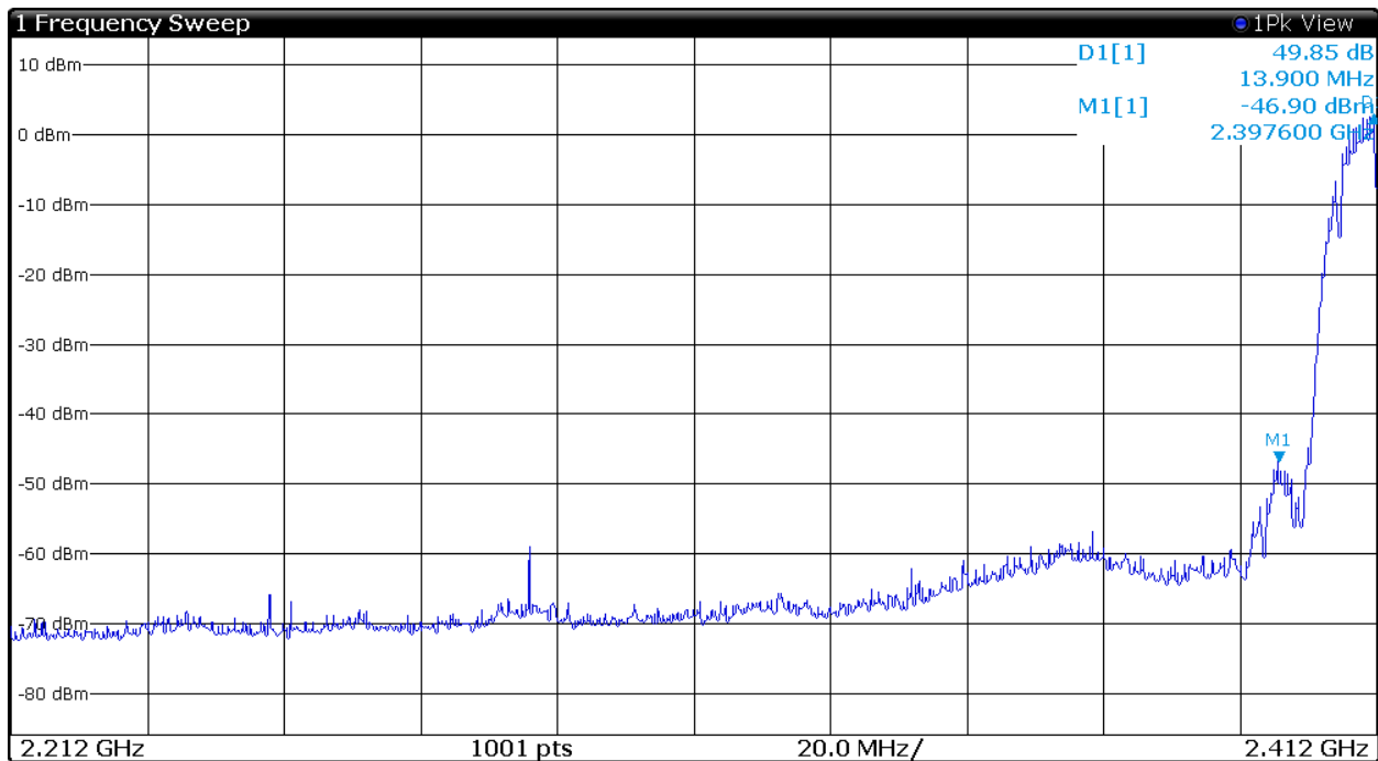
Figure 11 Plot of Transmitter Low Band Edge (802.11b, Chain 0)
