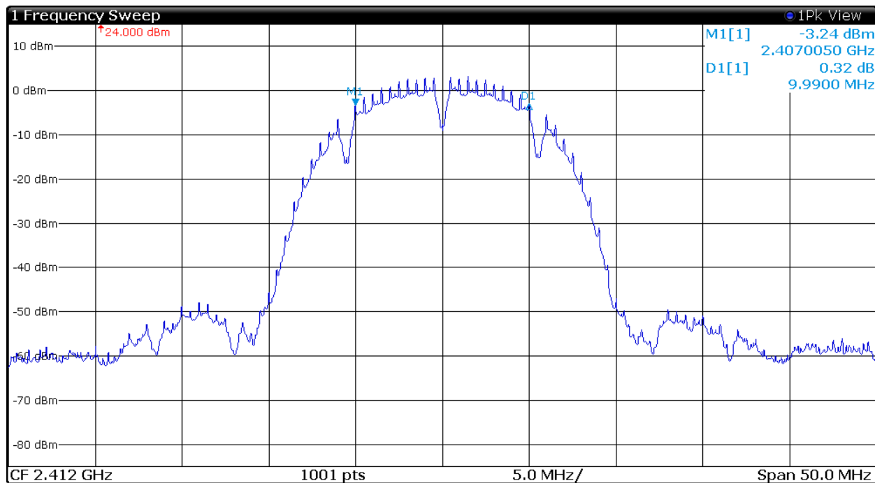
Figure 28 Plot of Transmitter 6-dB Occupied Band Width (802.11b, Chain 1)
