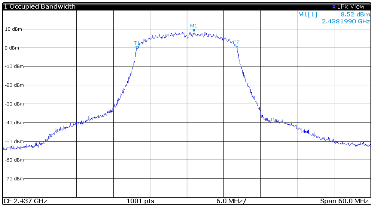
Figure 38 Plot of Transmitter 99% Occupied Band Width (802.11g, Chain 1)
