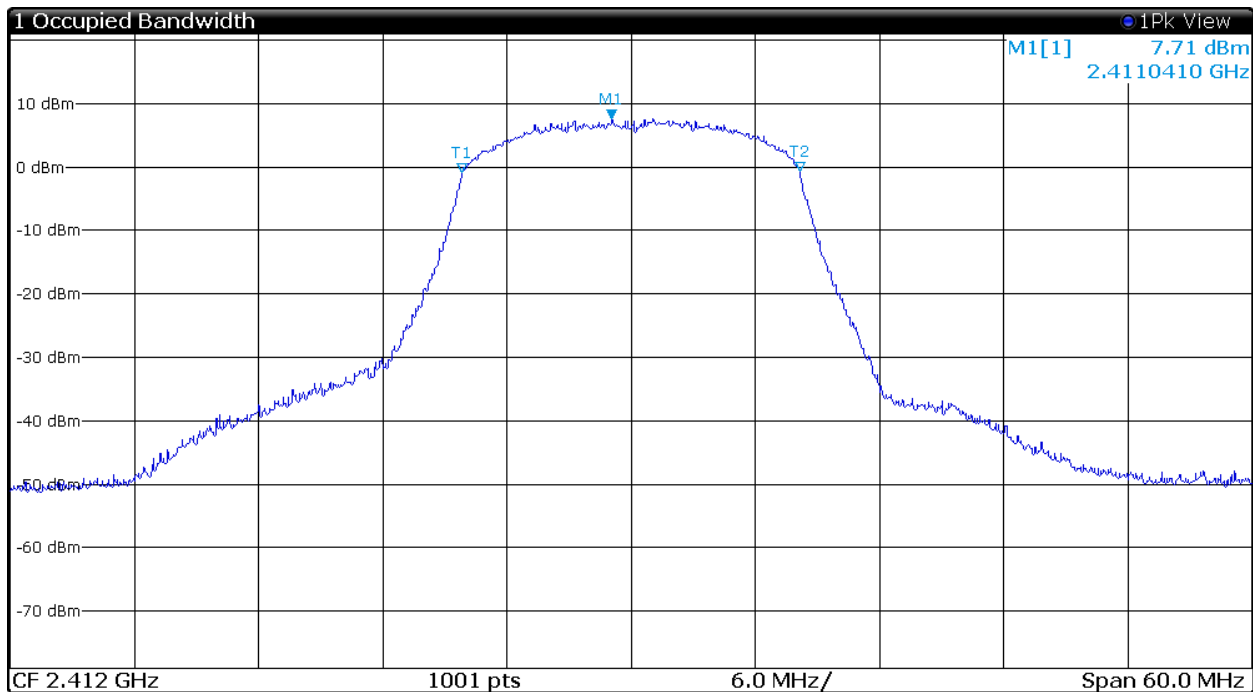
Figure 39 Plot of Transmitter 99% Occupied Band Width (802.11n (20), Chain 0)
