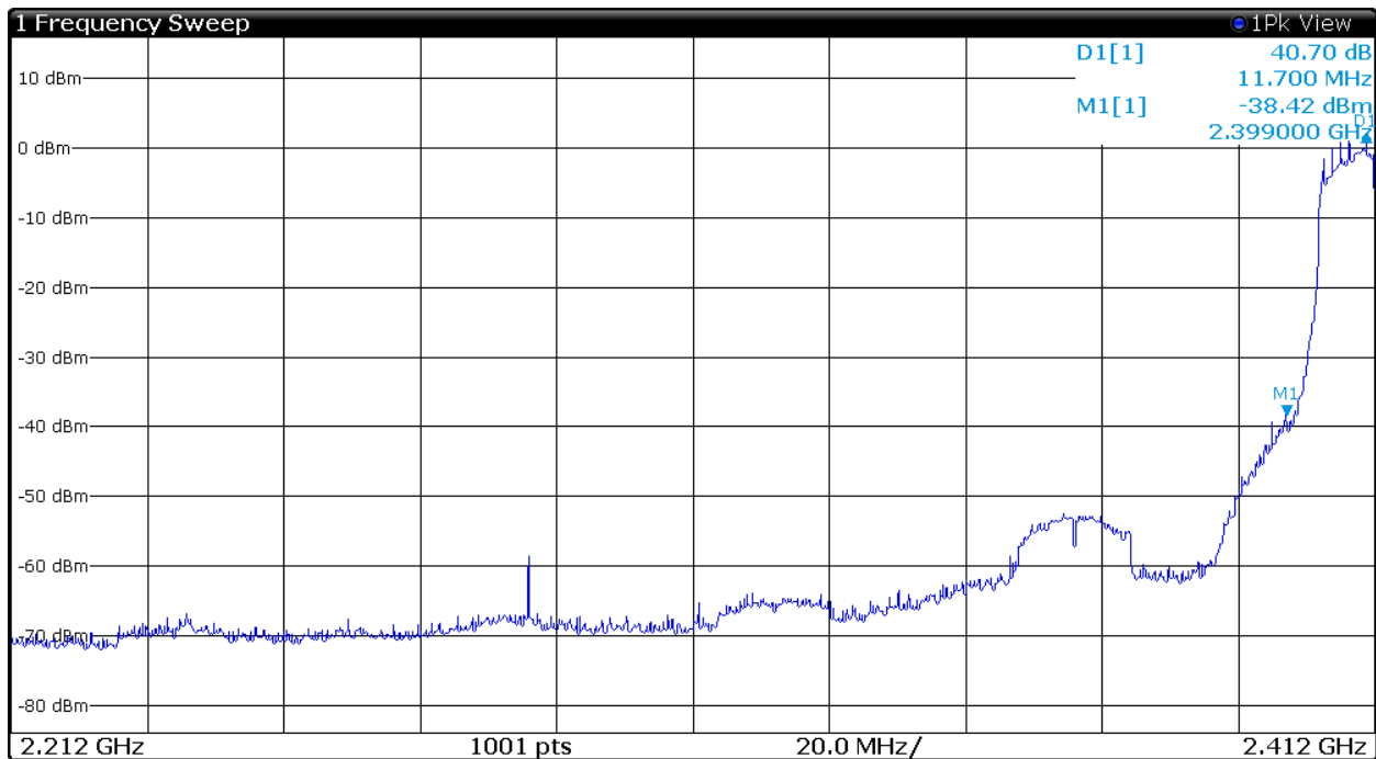
Figure 15 Plot of Transmitter Low Band Edge (802.11n (20), Chain 0)
