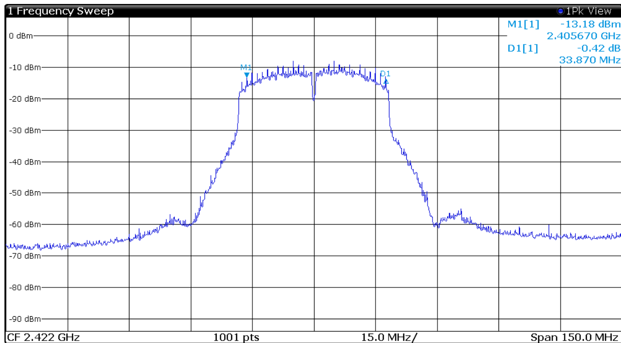
Figure 34 Plot of Transmitter 6-dB Occupied Band Width (802.11n (40), Chain 1)
