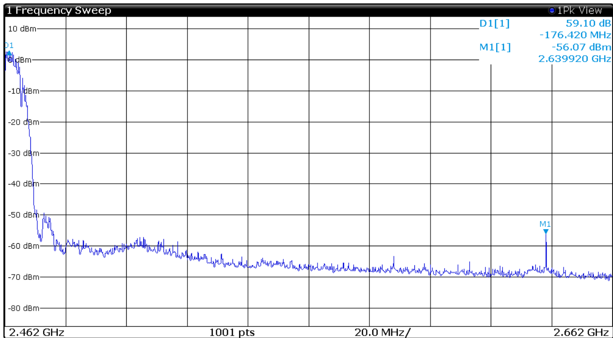
Figure 19 Plot of Transmitter High Band Edge (802.11b, Chain 0)
