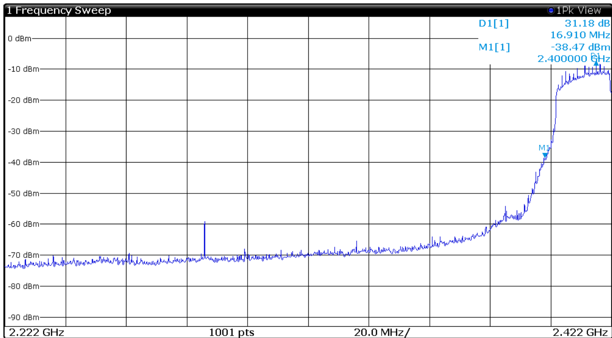
Figure 17 Plot of Transmitter Low Band Edge (802.11n (40), Chain 0)
