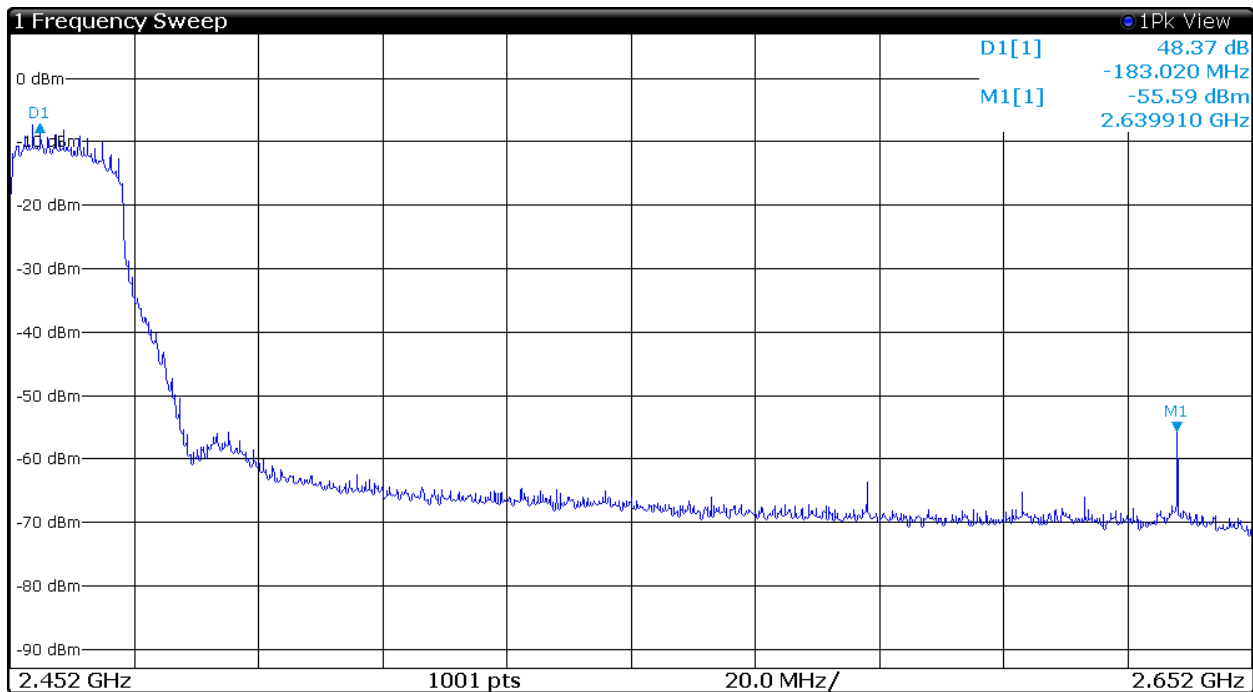
Figure 25 Plot of Transmitter High Band Edge (802.11n (40), Chain 0)
