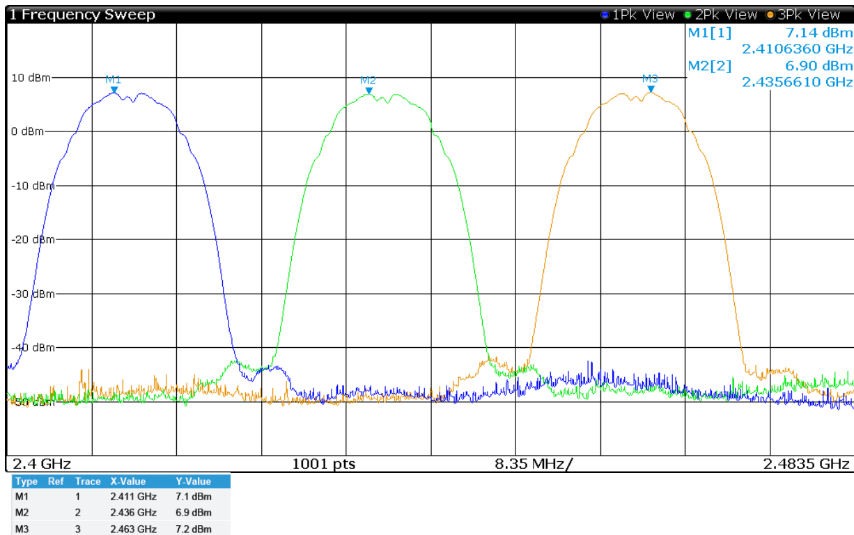
Figure 3 Plot of Transmitter Emissions (Across Operational Band 802.11b, Chain 0)
