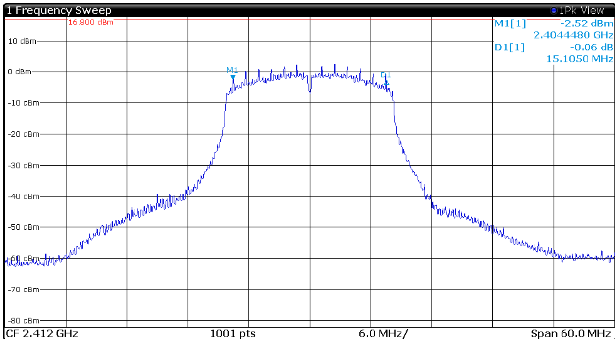
Figure 29 Plot of Transmitter 6-dB Occupied Band Width (802.11g, Chain 0)
