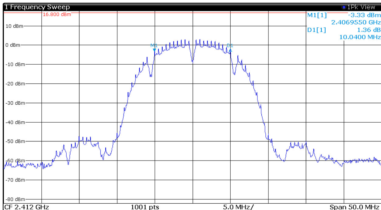
Figure 27 Plot of Transmitter 6-dB Occupied Band Width (802.11b, Chain 0)
