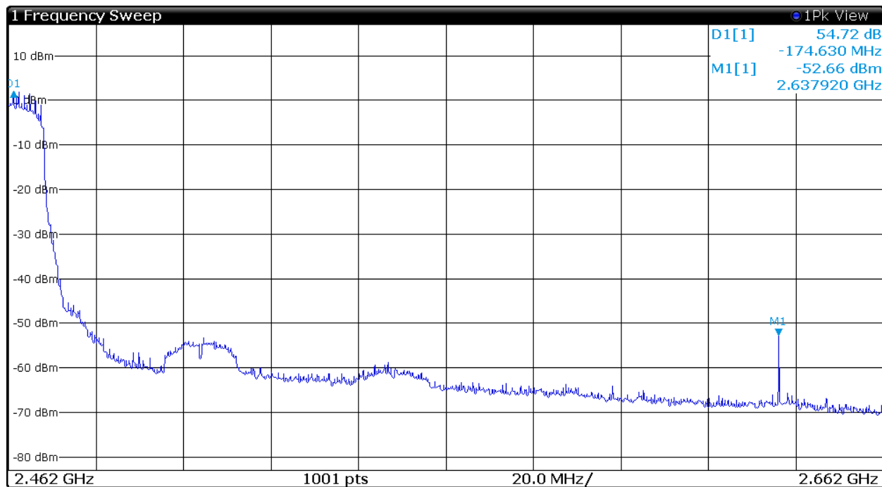
Figure 24 Plot of Transmitter High Band Edge (802.11n (20), Chain 1)
