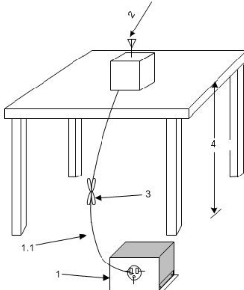
Diagram 1 Test arrangement for Conducted emissions
