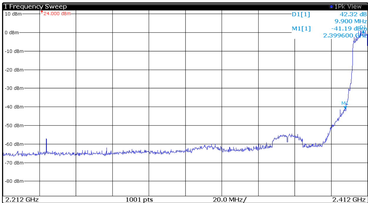
Figure 12 Plot of Transmitter Low Band Edge (802.11b, Chain 1)
