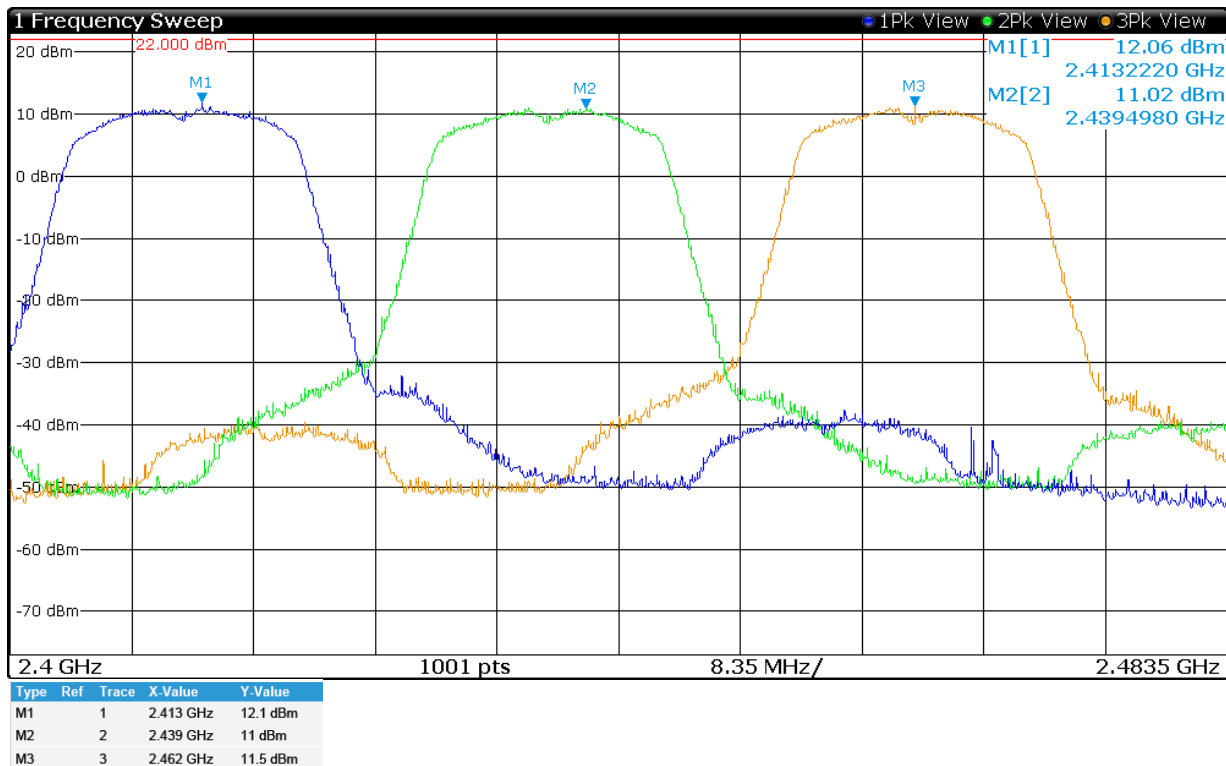
Figure 7 Plot of Transmitter Emissions (Across Operational Band, 802.11n (20), Chain 0)
