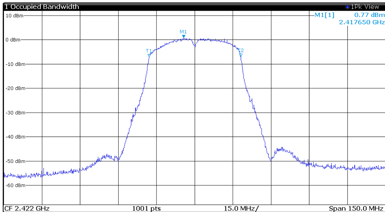
Figure 42 Plot of Transmitter 99% Occupied Band Width (802.11n (40), Chain 1)
