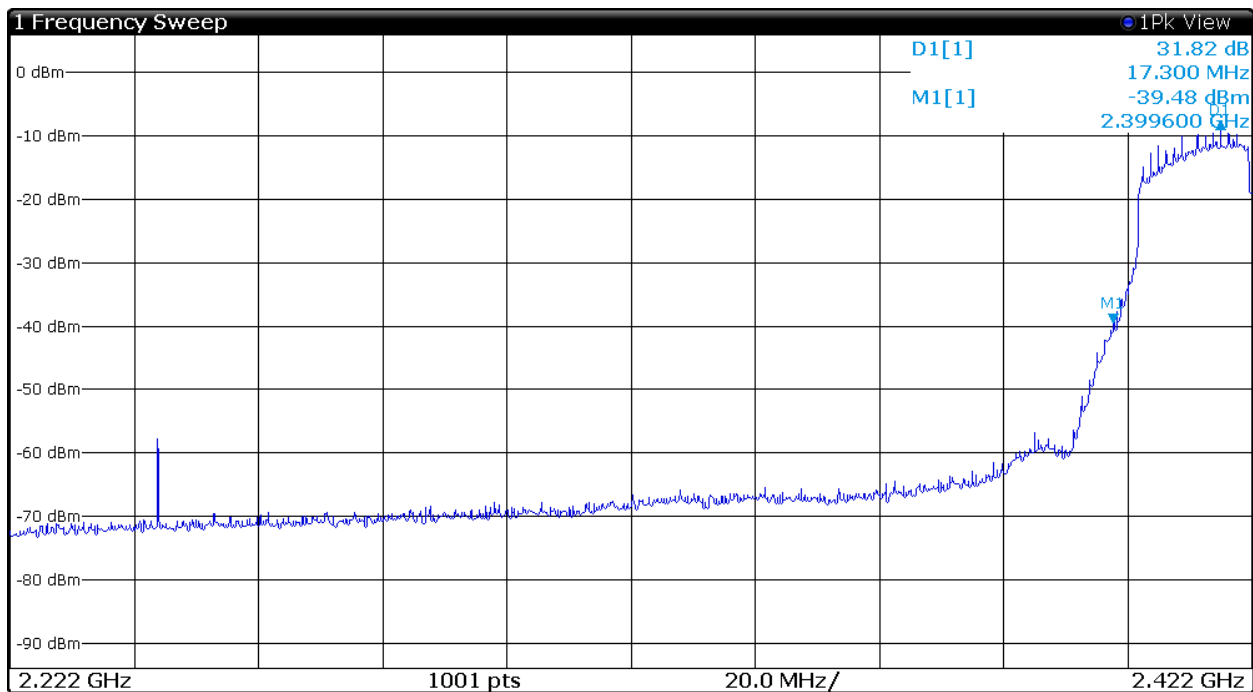
Figure 18 Plot of Transmitter Low Band Edge (802.11n (40), Chain 1)
