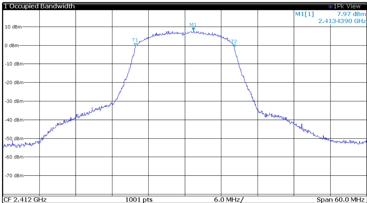
Figure 37 Plot of Transmitter 99% Occupied Band Width (802.11g, Chain 0)
