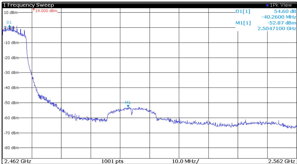
Figure 21 Plot of Transmitter High Band Edge (802.11g, Chain 0)
