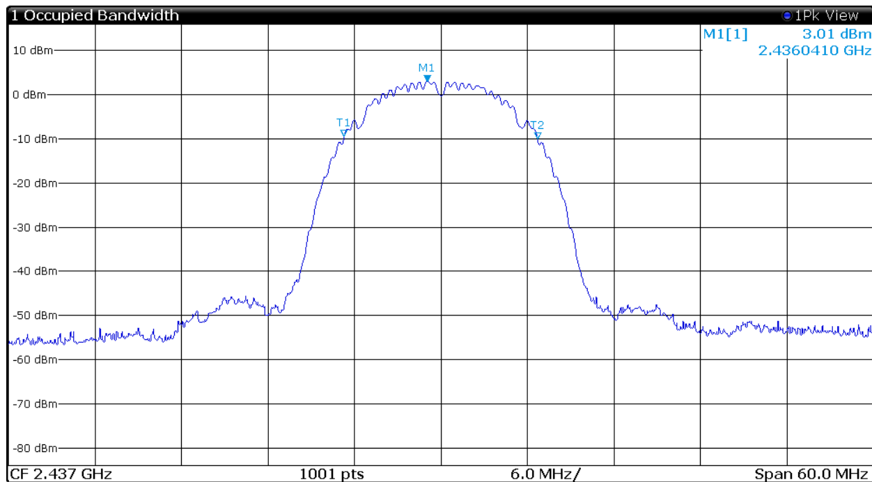
Figure 36 Plot of Transmitter 99% Occupied Band Width (802.11b, Chain 1)
