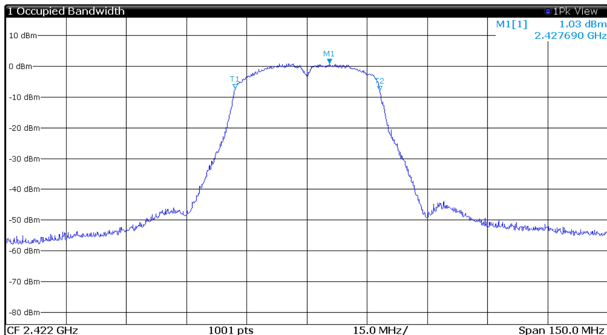
Figure 41 Plot of Transmitter 99% Occupied Band Width (802.11n (40), Chain 0)
