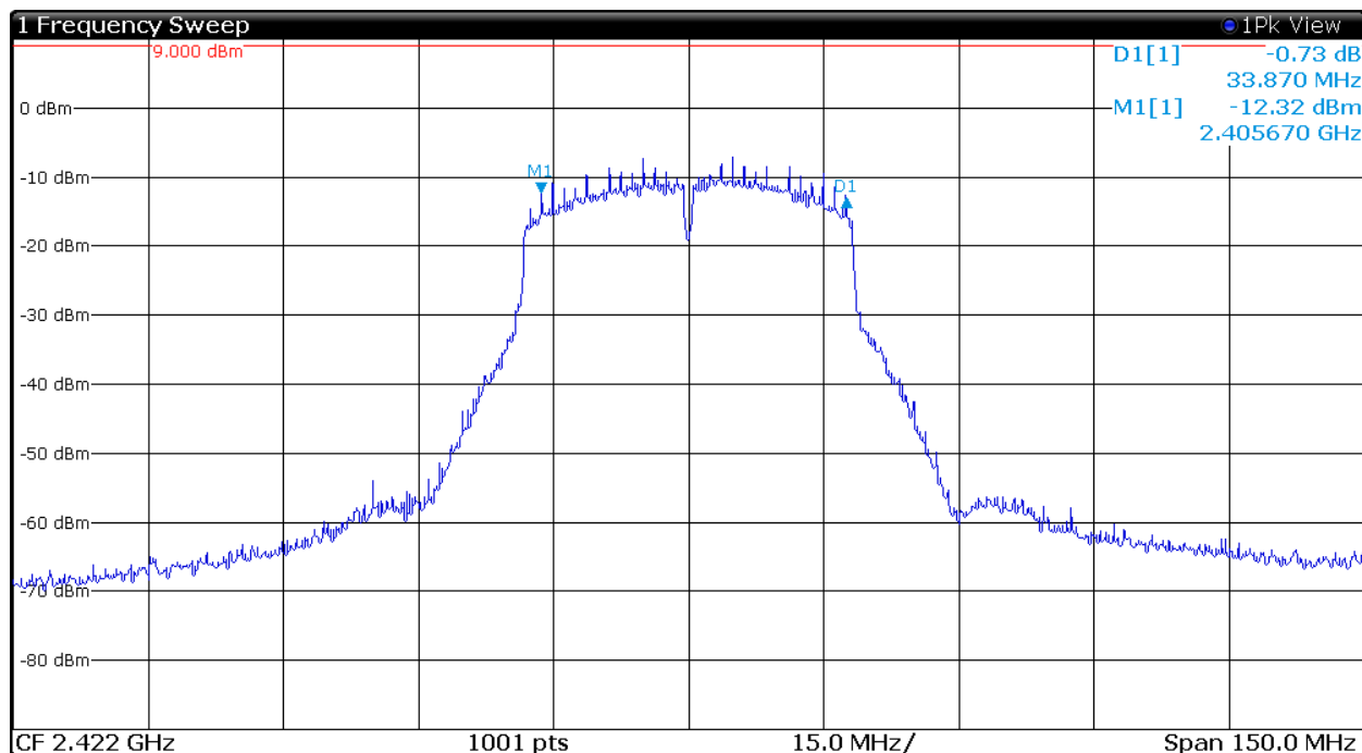
Figure 33 Plot of Transmitter 6-dB Occupied Band Width (802.11n (40), Chain 0)
