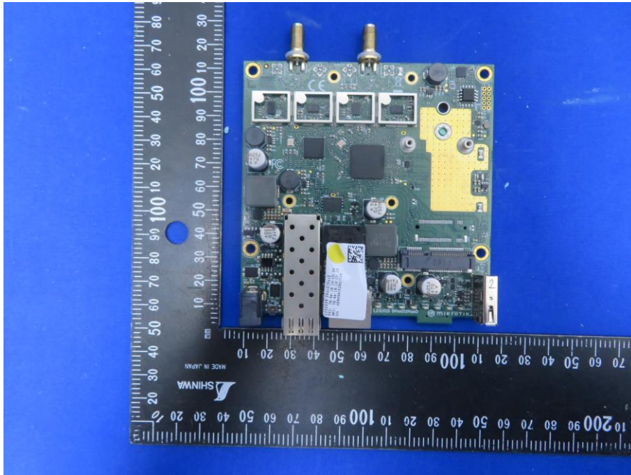
(7) EUT Photo
