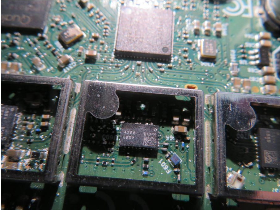
(7) EUT Photo
