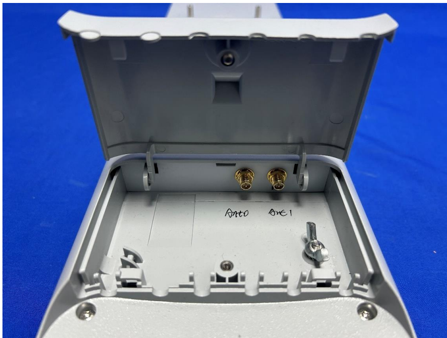
(8) Sector Antenna (MTAS-5G-19D120)
