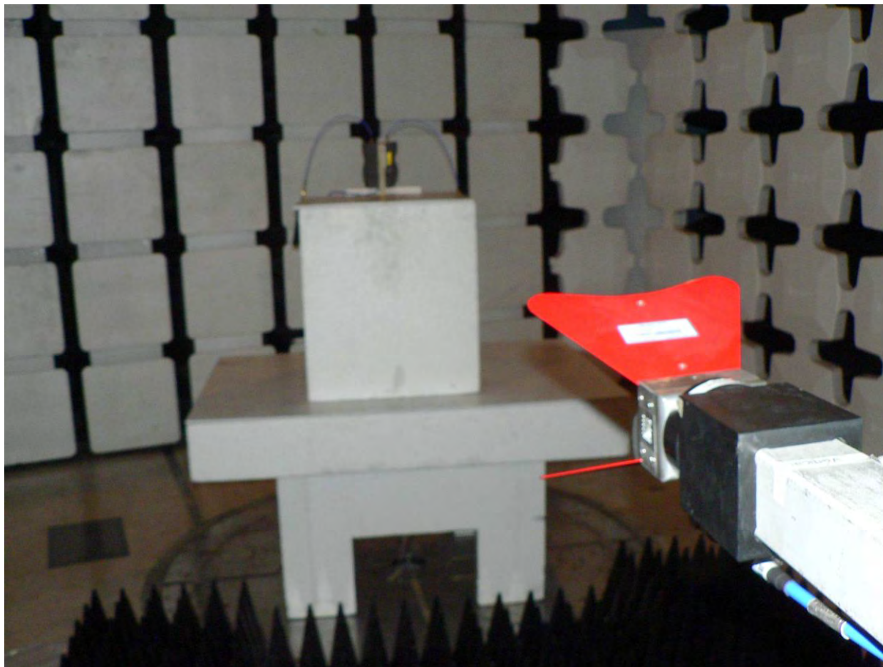
HGO-Antenna-OUT
