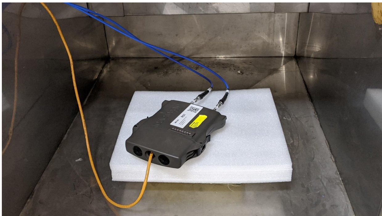
Conducted RF
