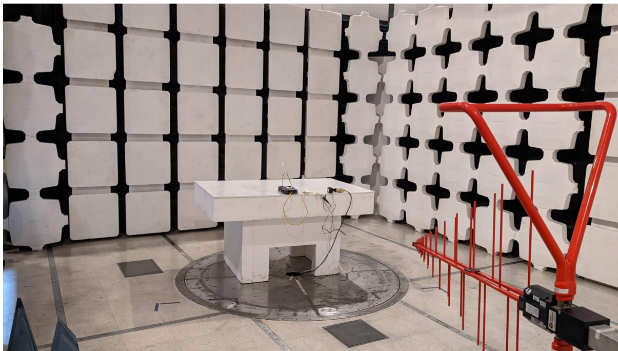
Digital Emissions with POE
