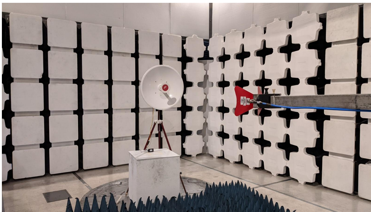
MTAD-5G-30D3 Spurious Emissions
