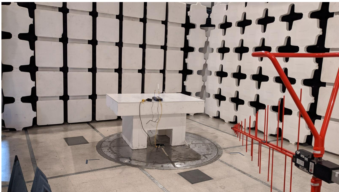
Digital Emissions with ACDC Adapter
