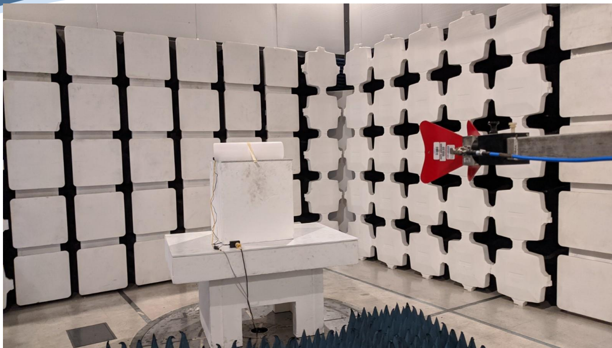
MTAS-5G-19D120 Spurious Emissions
