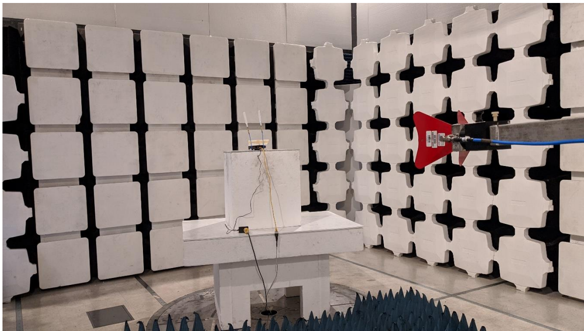
DA-2450-05RP-SMA-01 Spurious Emissions
