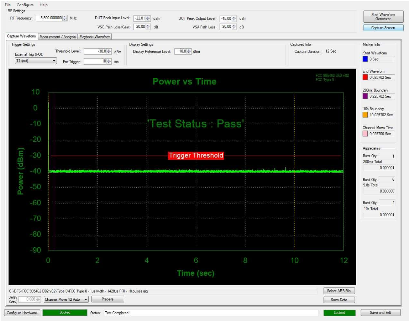
Figure 8.6-1: Channel closing transmission and move time
