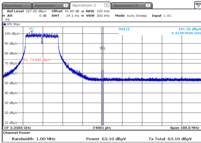
Figure 8.8-1: Peak spurious emissions within restricted bands at high channel, 802.11a cho
