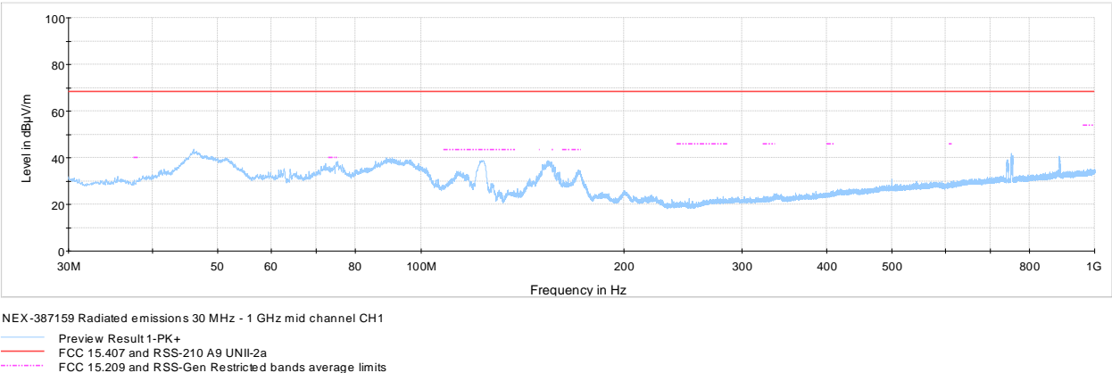
Figure 8.8-17: Radiated spurious emissions 30 MHz – 1 GHz mid channel ch1
