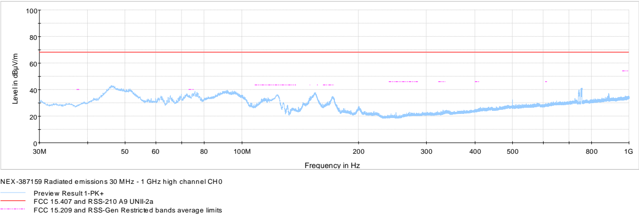
Figure 8-15: Radiated spurious emissions 30 MHz – 1 GHz high channel cho
