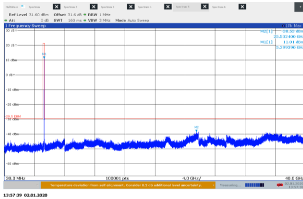
Figure 8.8-45: Conducted spurious emissions 30 MHz – 40 GHz mid channel, 802.11a ch 0
