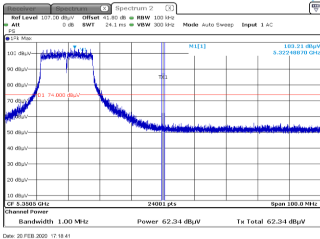
Figure 8.8-3: Peak spurious emissions within restricted bands at high channel, 802.11a ch1
