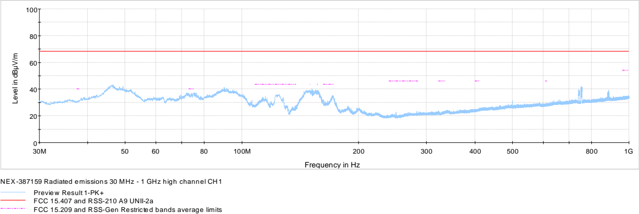
Figure 8.8-18: Radiated spurious emissions 30 MHz – 1 GHz high channel ch1
