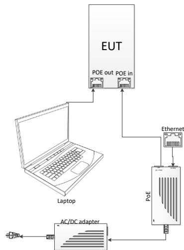
Figure 3.6-1: Setup diagram
