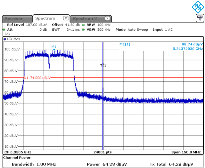
Figure 8.8-5: Peak spurious emissions within restricted bands at high channel, 802.11n cho
