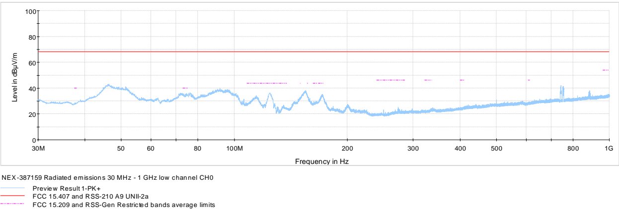
Figure 8-13: Radiated spurious emissions 30 MHz – 1 GHz low channel cho
