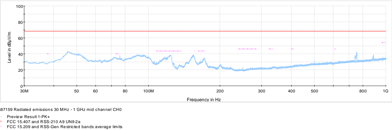
Figure 8-14: Radiated spurious emissions 30 MHz – 1 GHz mid channel cho
