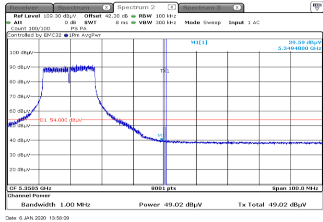
Figure 8.8-2: Average spurious emissions within restricted bands at high channel, 802.11a cho
