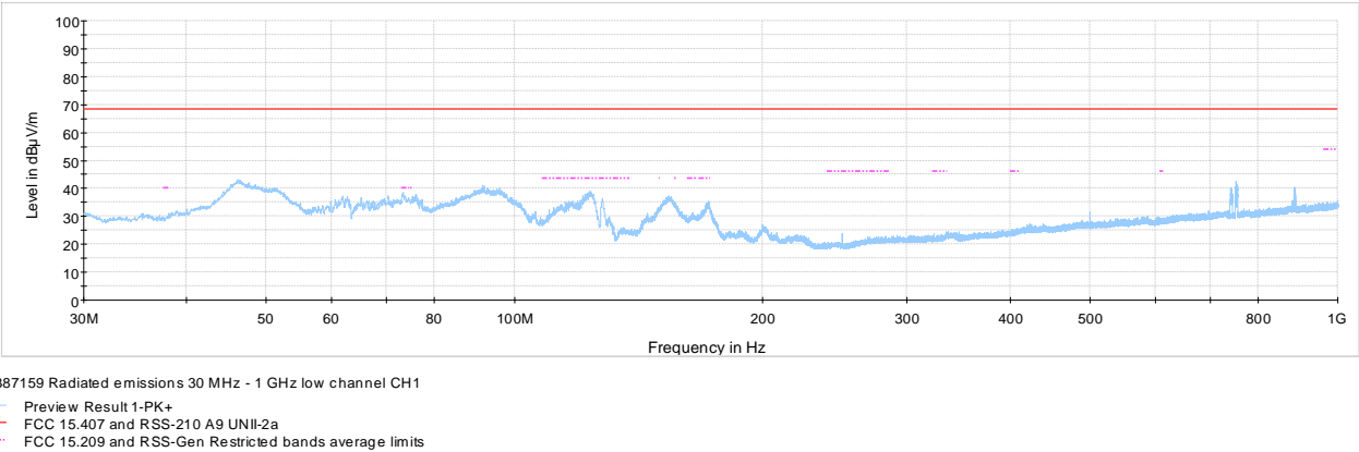
Figure 8.8-16: Radiated spurious emissions 30 MHz – 1 GHz low channel ch1
