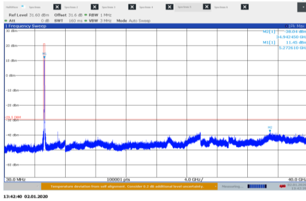
Figure 8.8-43: Conducted spurious emissions 30 MHz – 40 GHz low channel, 802.11a ch 0
