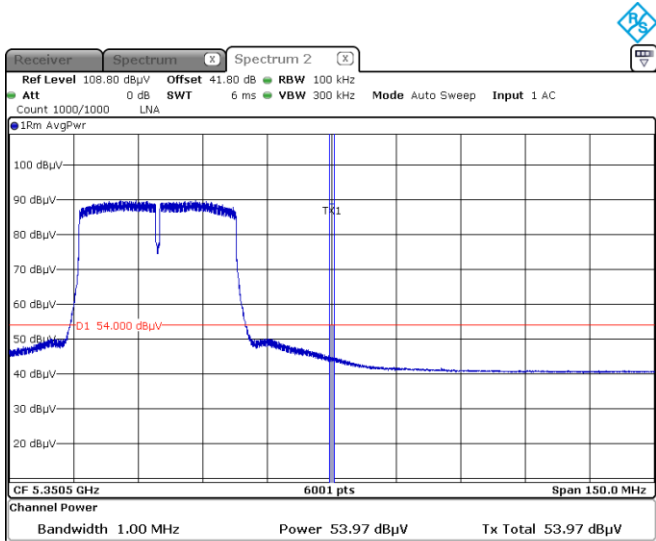
Figure 8.8-6: Average spurious emissions within restricted bands at high channel, 802.11n cho
