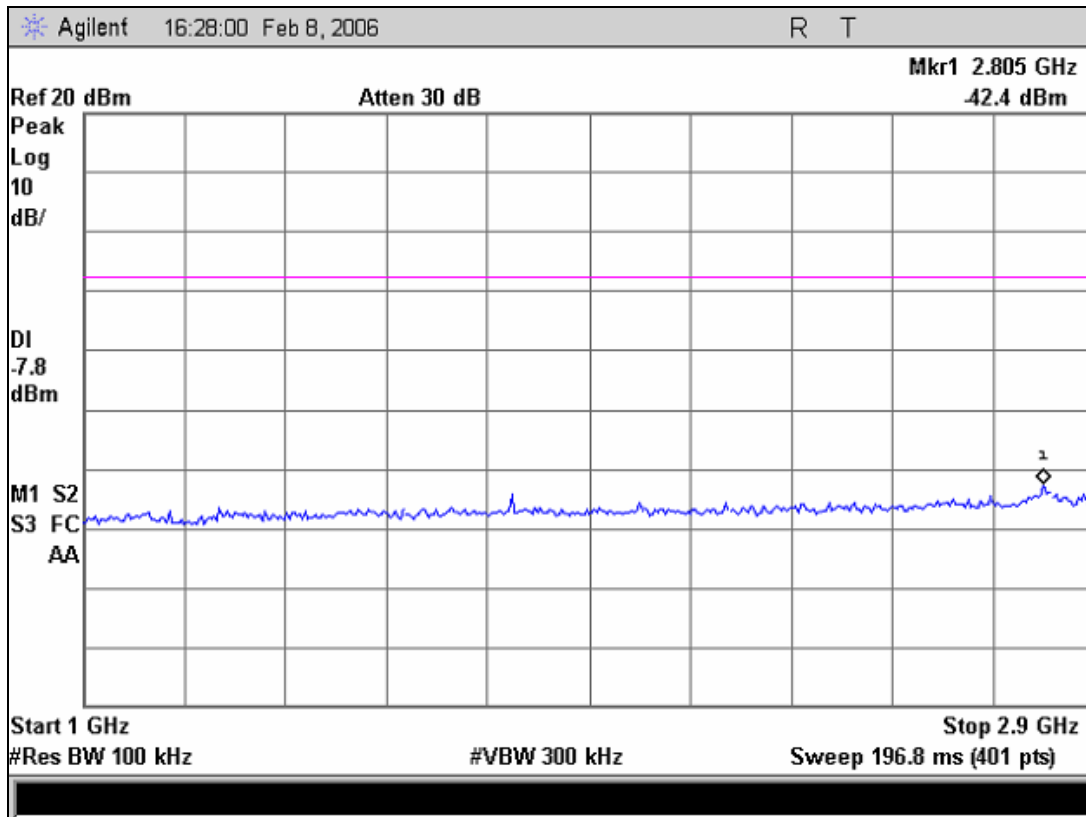
Plot 17. Spurious Conducted Emissions – 2
