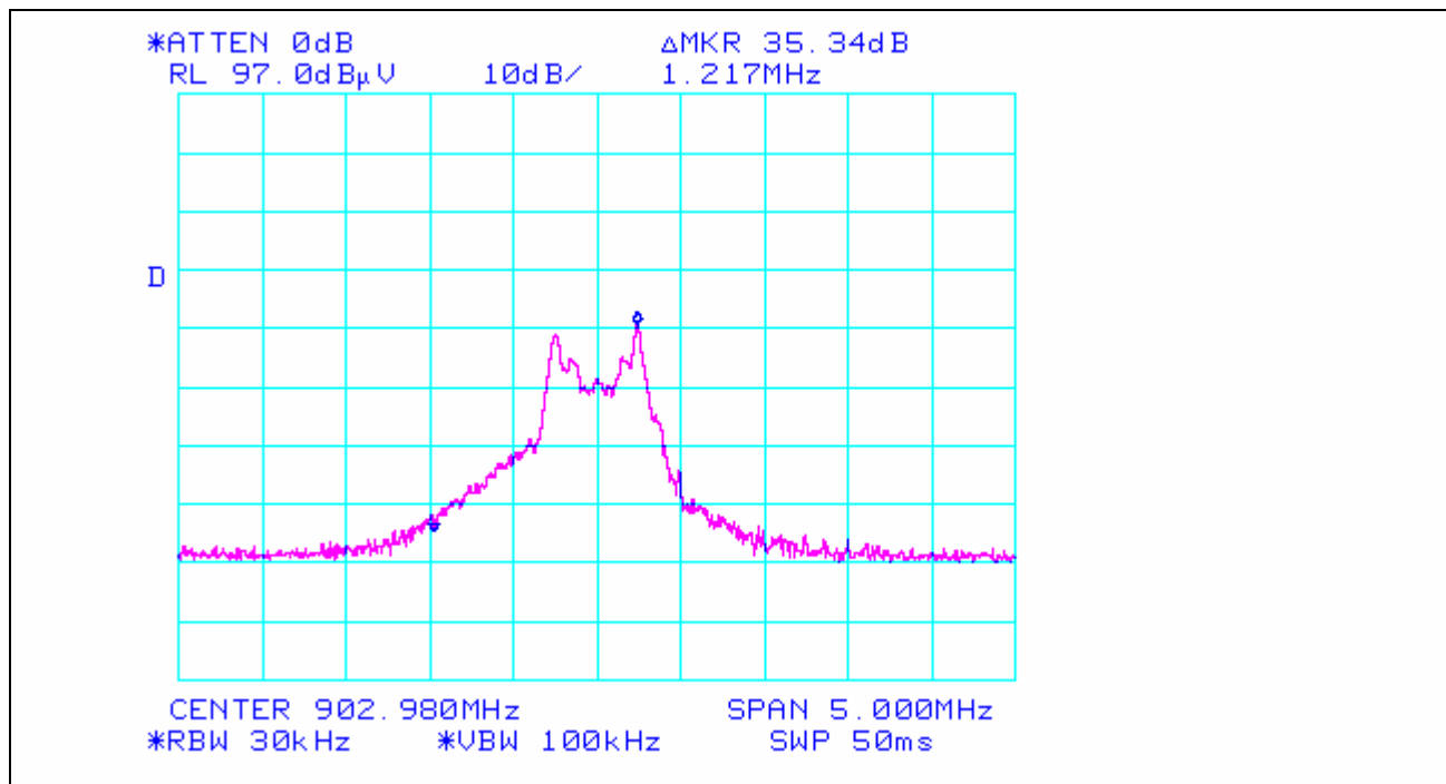
Plot 10. Band Edge Emissions – Lower Delta
