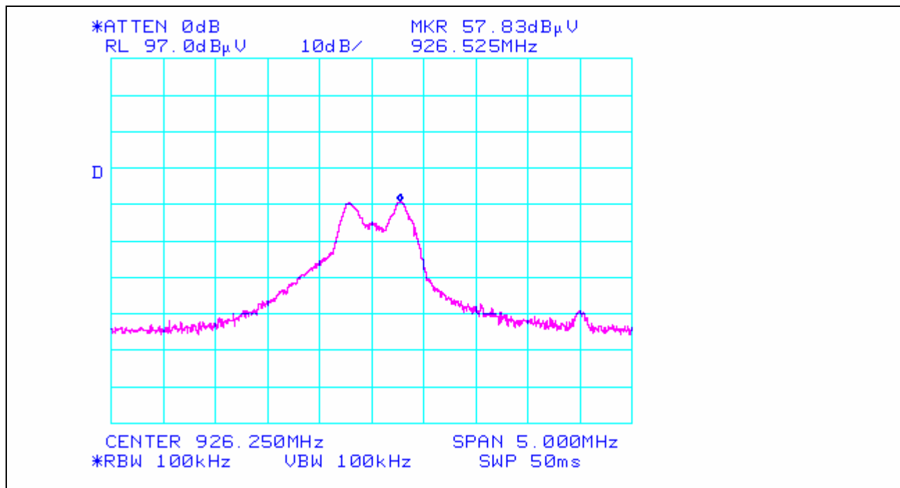
Plot 11. Band Edge Emissions – Upper Peak
