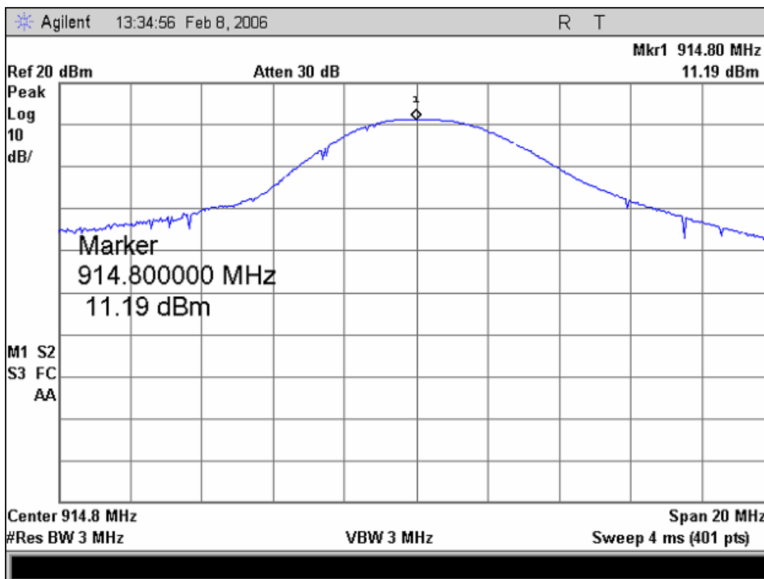
Plot 7. Output Power – Channel 17
