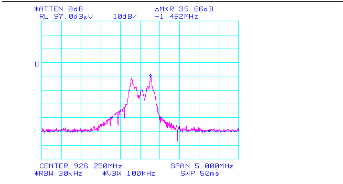
Plot 12. Band Edge Emissions – Upper Delta
