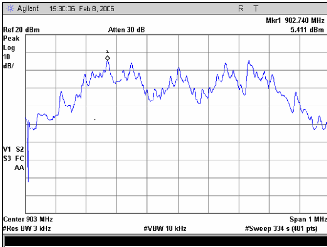
Plot 13. Spectral Power Density – Channel 1
