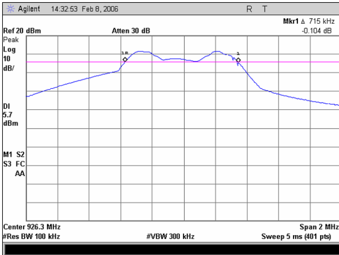
Plot 5. Occupied Bandwidth, 6 dB – Channel 32
