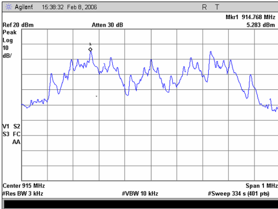
Plot 14. Spectral Power Density – Channel 17
