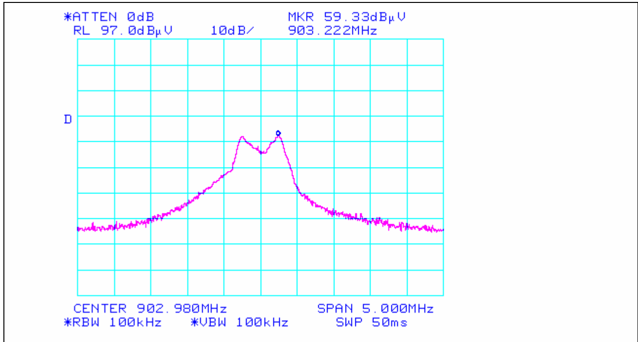
Plot 9. Band Edge Emissions – Lower Peak
