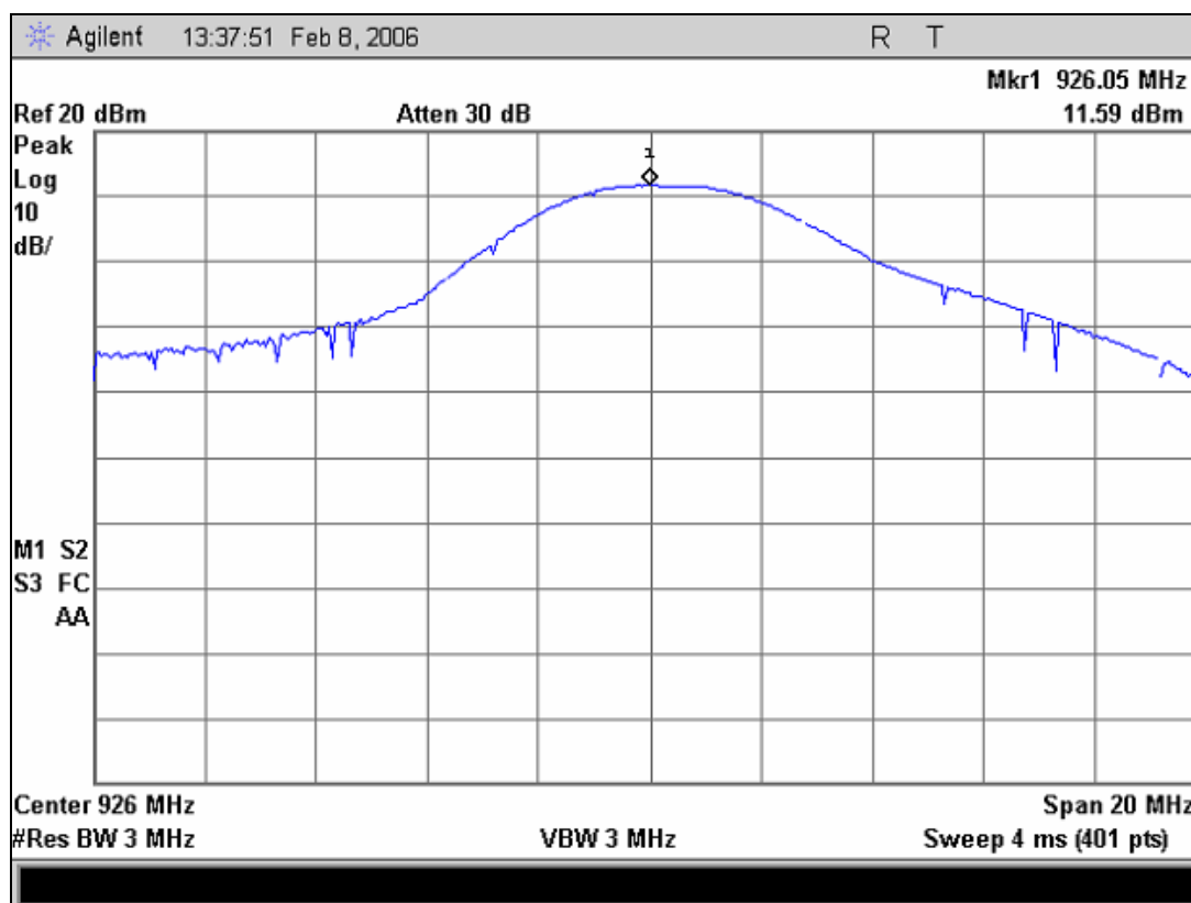
Plot 8. Output Power – Channel 32
