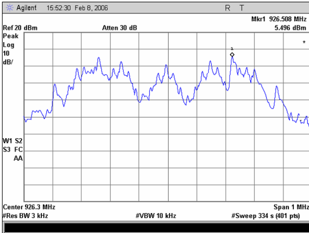
Plot 15. Spectral Power Density – Channel 32
