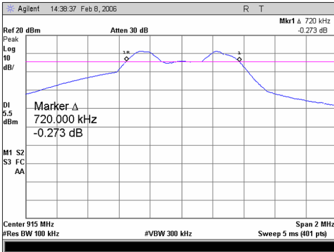
Plot 4. Occupied Bandwidth, 6 dB – Channel 17
