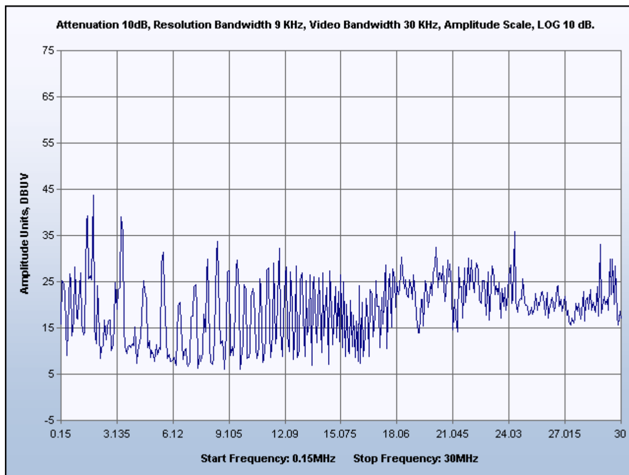
Plot 1. Conducted Emissions – Test Results, 0.15 MHz – 30 MHz – Phase Line
