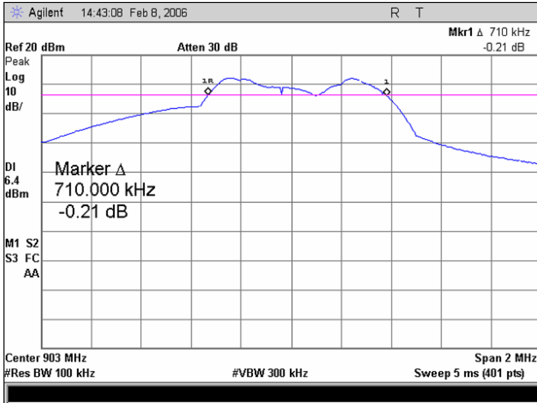
Plot 3. Occupied Bandwidth, 6 dB – Channel 1
