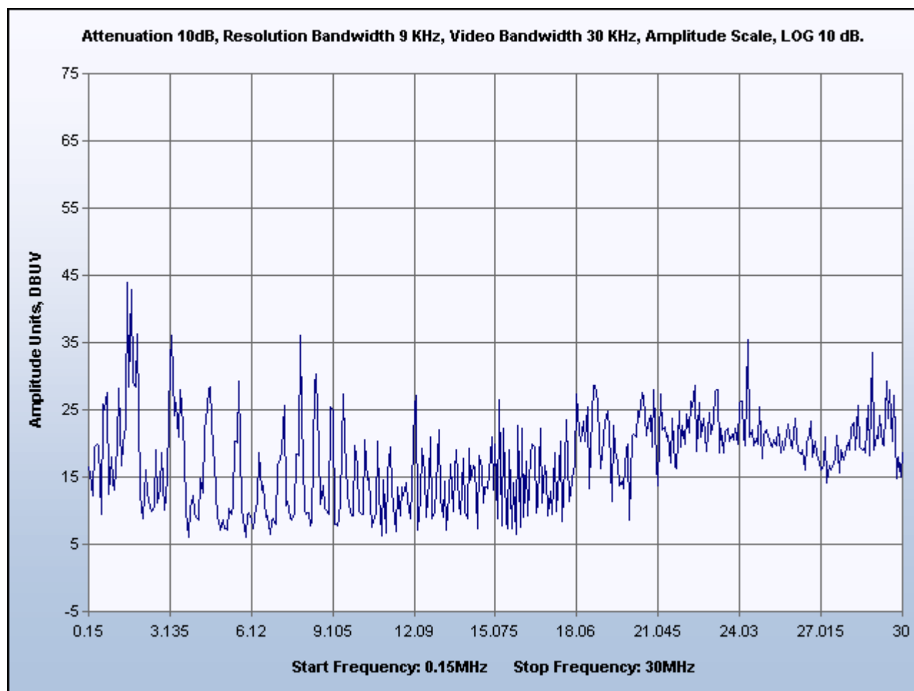
Plot 2. Conducted Emissions – Test Results, 0.15 MHz – 30 MHz – Neutral Line
