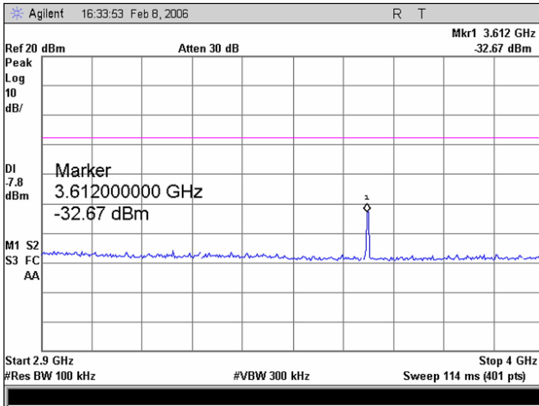
Plot 18. Spurious Conducted Emissions – 3
