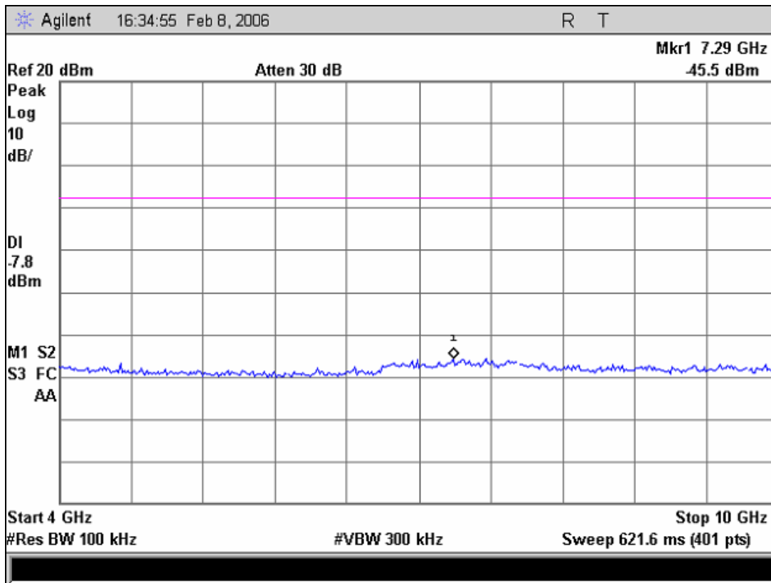
Plot 19. Spurious Conducted Emissions – 4
