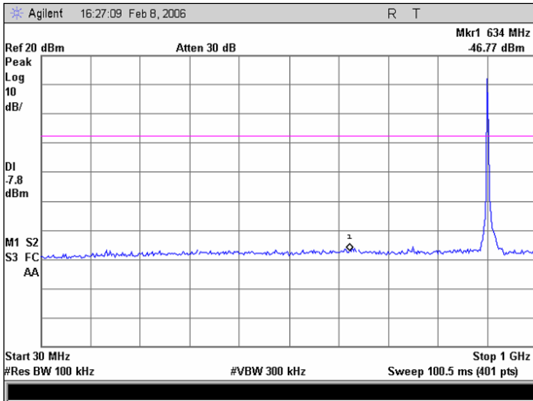
Plot 16. Spurious Conducted Emission – 1
