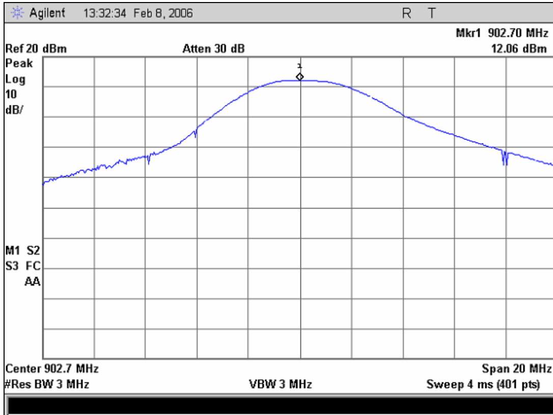
Plot 6. Output Power – Channel 1
