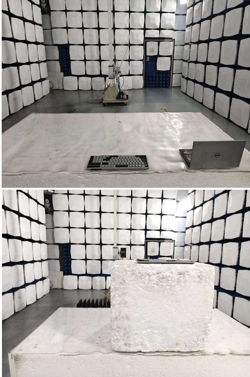
Radiated emission test view- Model: BK-7114WG
