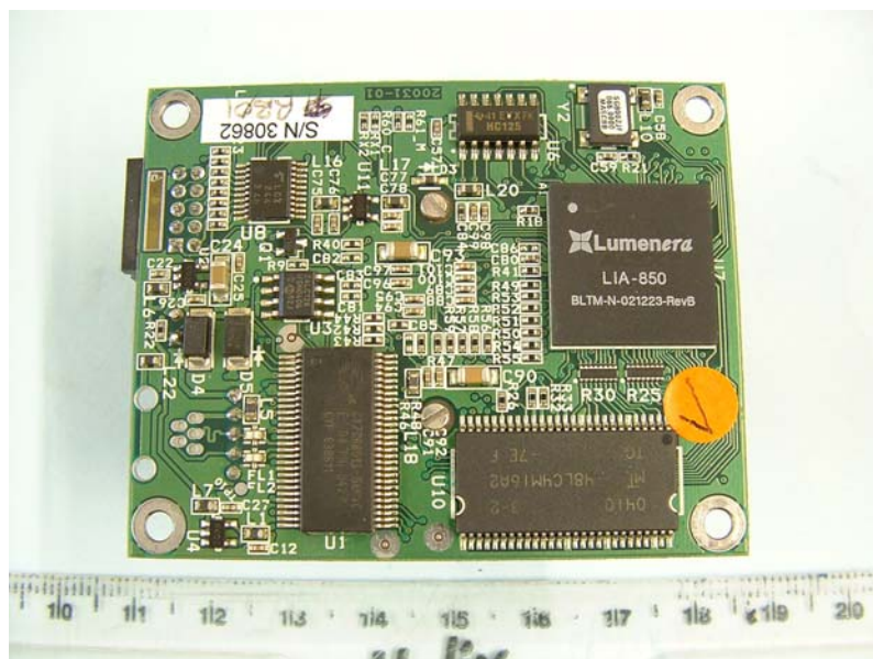
Camera PCB Bottom Side
