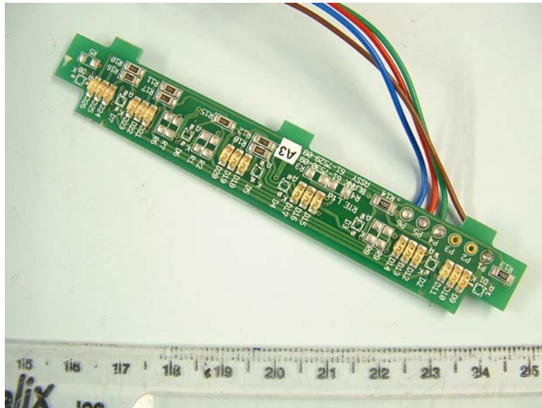
Short Illumination Board Component Side
