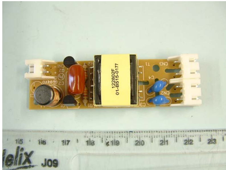
PSU PCB Component Side
