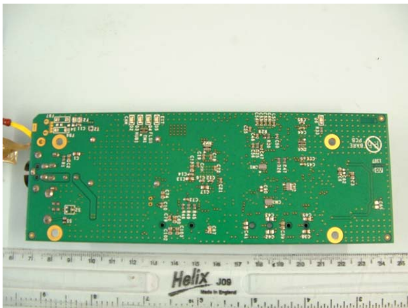
Hub Board Track Side
