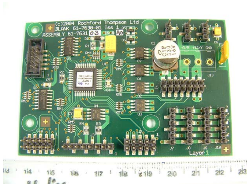
Lighting Control PCB Component Side
