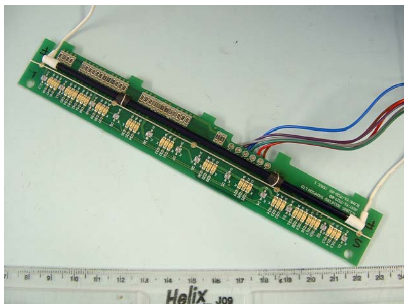
Long Illumination Board Component Side
