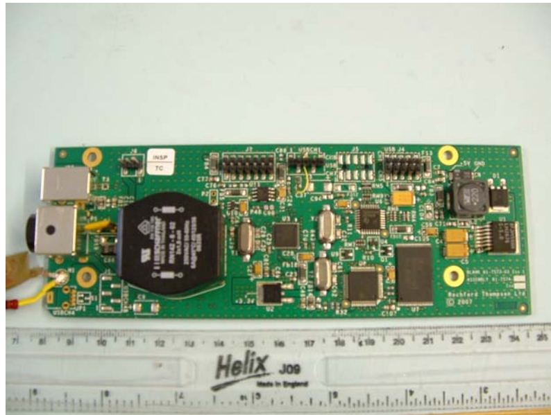
Hub Board Component Side
