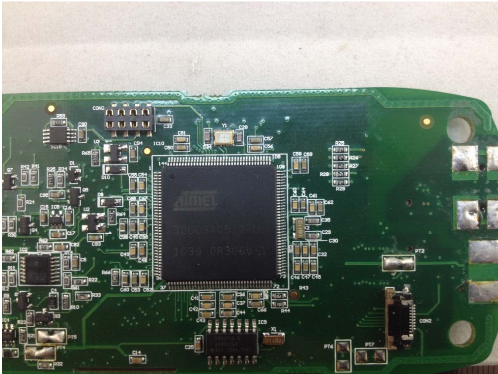
MAIN BOARD VIEW 2
