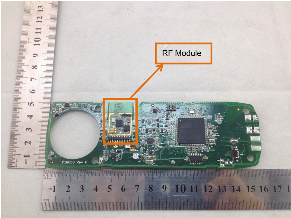
MAIN BOARD VIEW 1
