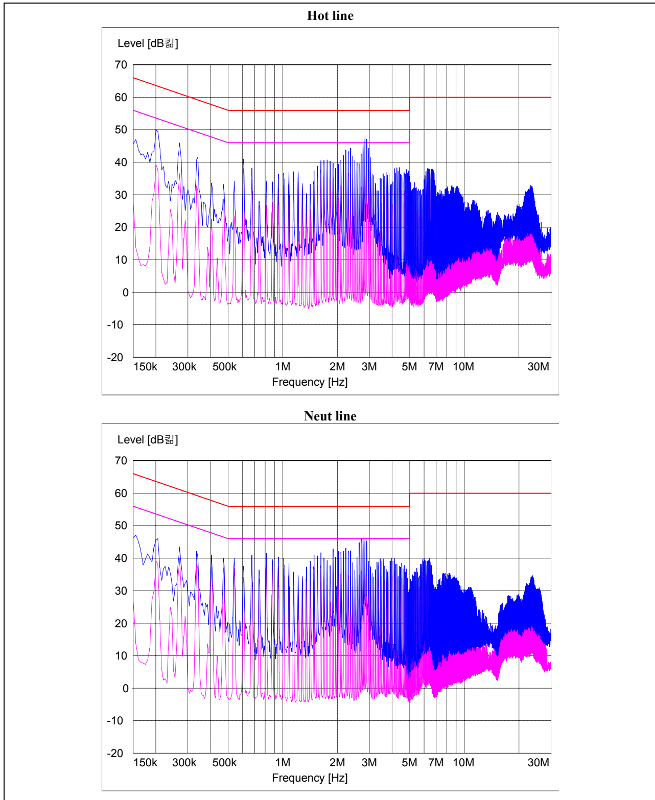
Figure 1. Operating condition : Graphical representation of conducted emissions Hot line
