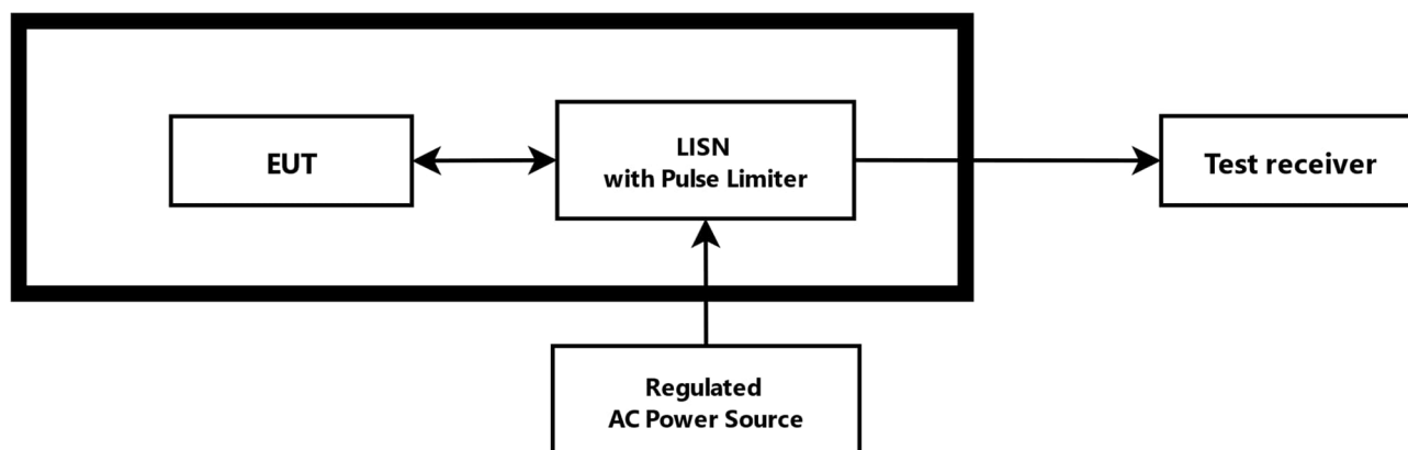
Test Set-Up 4
