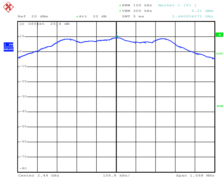
PSD 100kHz Plot on Channel 19 for 1Mbps
