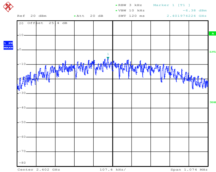
PSD 3kHz Plot on Channel 00 for 1Mbps
