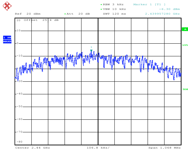
PSD 3kHz Plot on Channel 19 for 1Mbps
