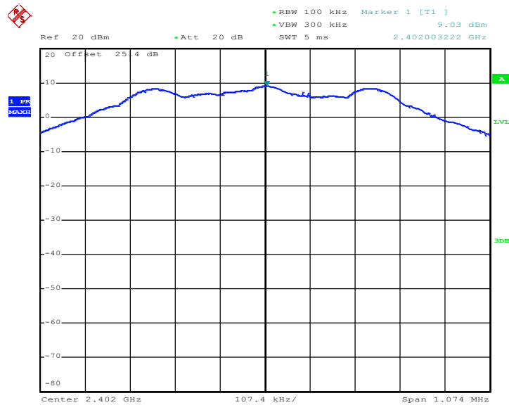
PSD 100kHz Plot on Channel 00 for 1Mbps
