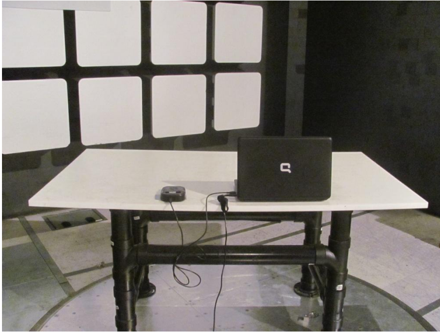
Photo 1.1-1: Radiated emissions setup
