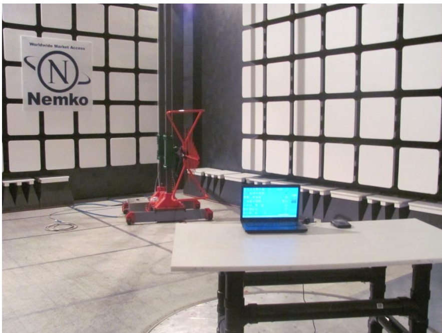
Photo 1.1-2: Radiated emissions setup
