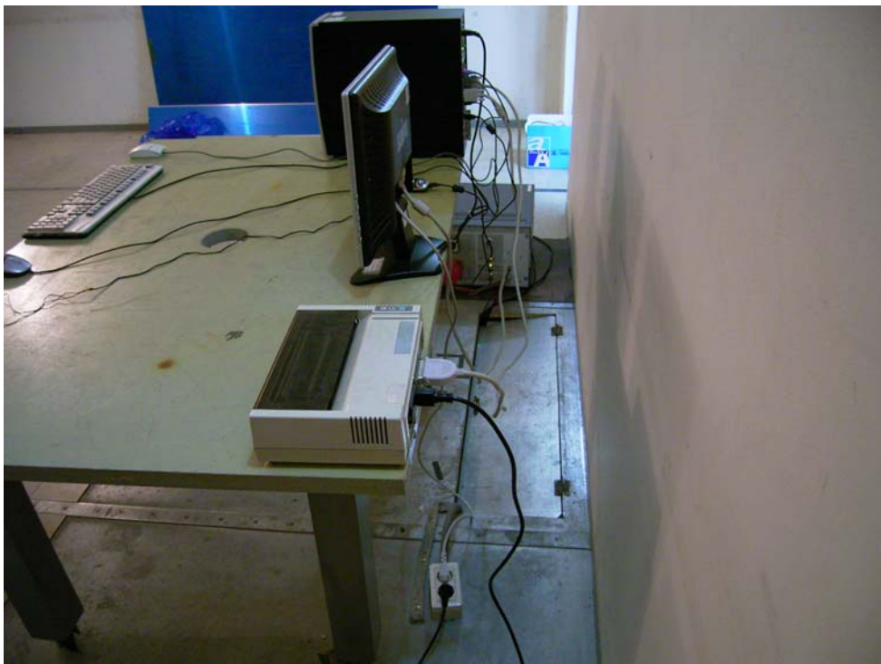
Conducted Emissions(PC power line) - Rear View
