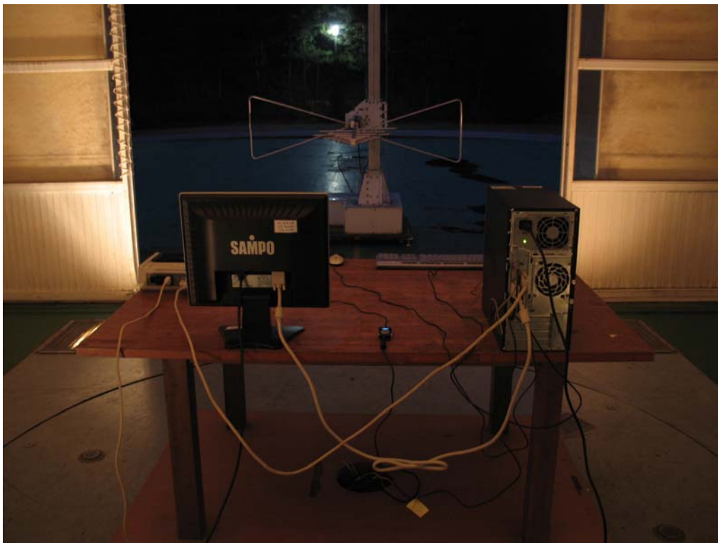
Radiated Emissions(30MHz-1GHz)-Rear View(Files read/write mode)
