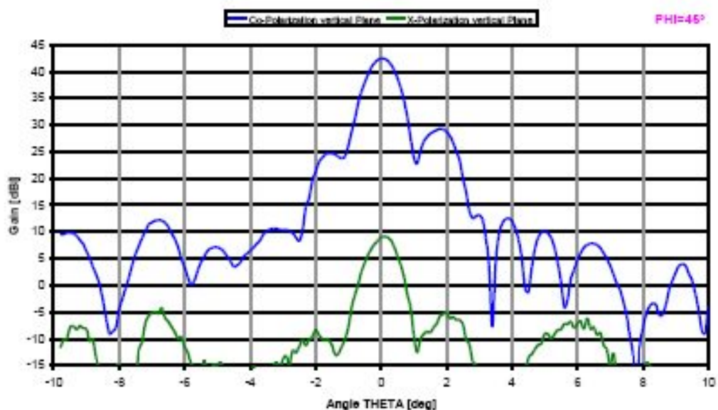
SL80-HGA Gain-Pattern CO-/X-Polarization vertical Plane @ 82.5GHz, Peak Gain = 42.5dBi
