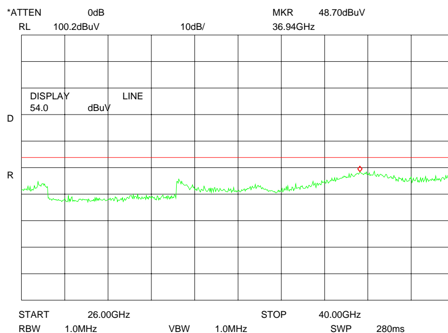
Plot 9: 26 - 40 GHz (Terminal A)
