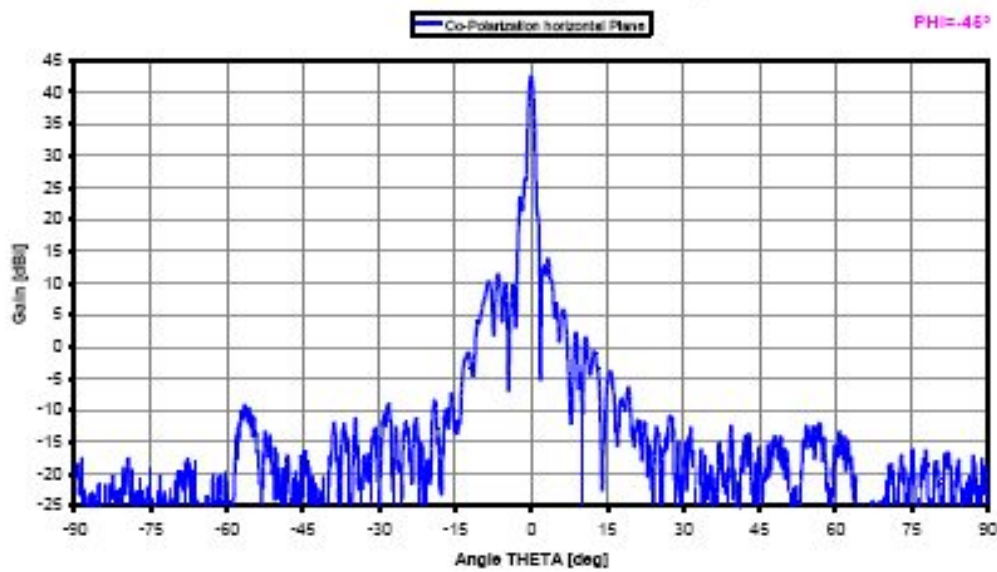
8L80-HGA Gain-Pattern Co-Polarization horizontal Plane @ 82.6GHz, Peak Gain = 42.6dBi
