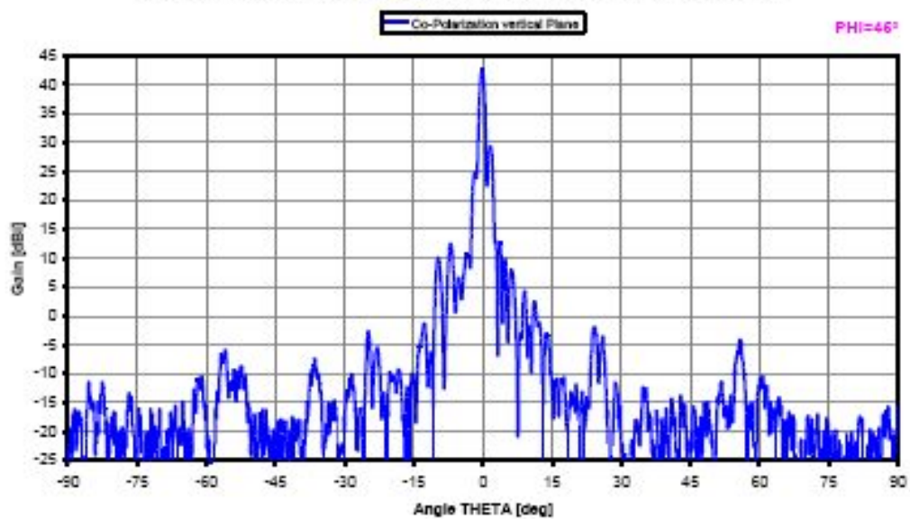
SL80-HGA Gain-Pattern Co-Polarization vertical Plane @ 82.5GHz, Peak Gain = 42.5dBi
