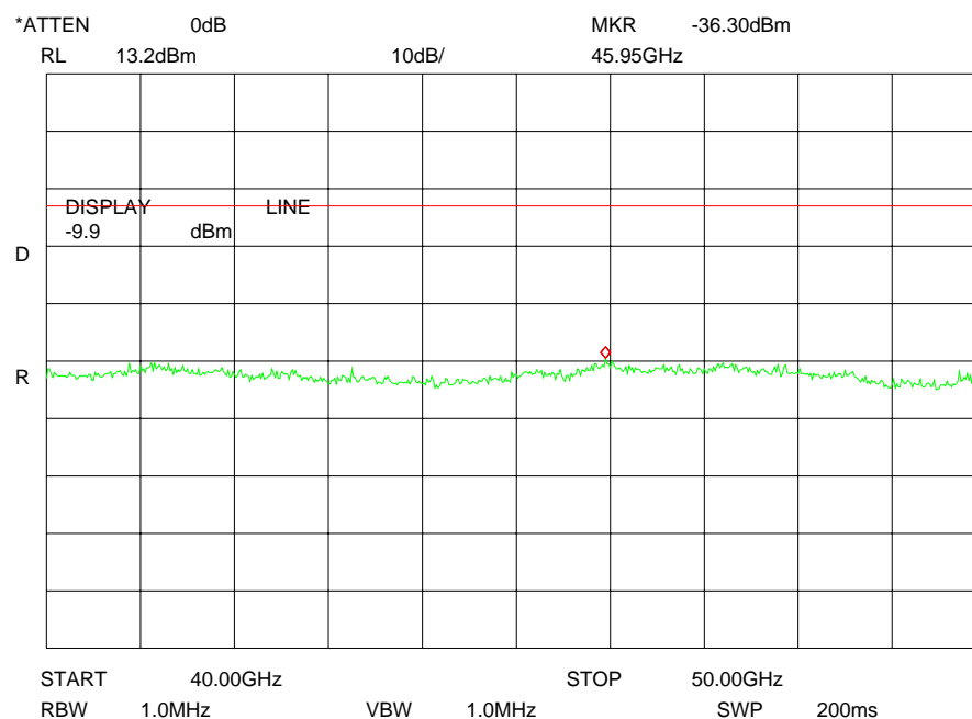
Plot 10: 40 - 50 GHz (Terminal A)
