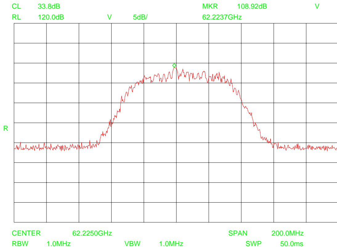
Plot 2e (Terminal B) Field strength at 3m test distance
