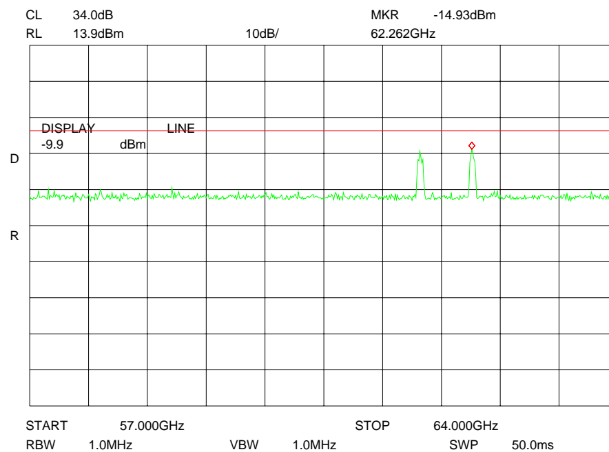
Plot 26: 57 - 64 GHz (Terminal B)
