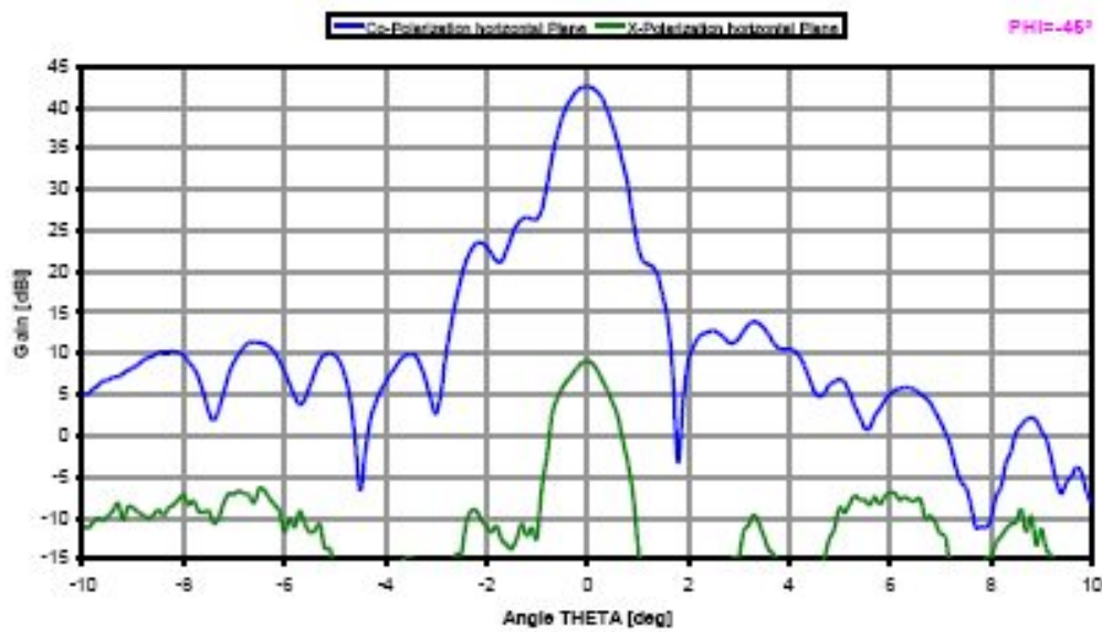
8L80-HGA Gain-Pattern Co/X-Polarization horizontal Plane @ 82.6GHz, Peak Gain = 42.6dBi
