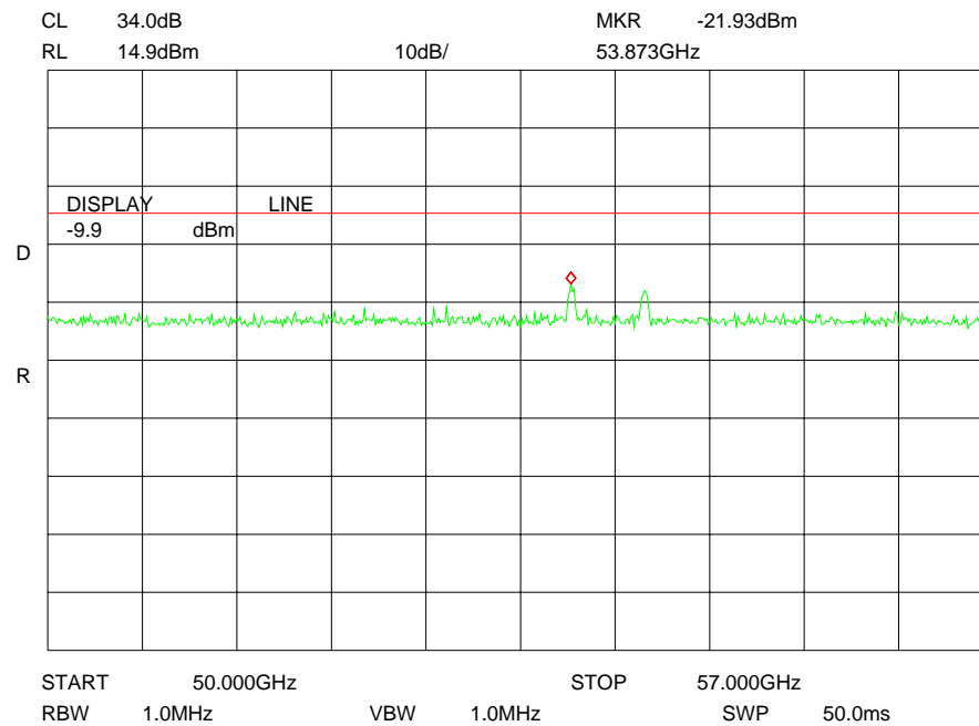
Plot 25: 50 - 57 GHz (Terminal B)
