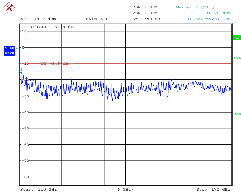
Plot 15: 110 - 170 GHz (Terminal A)
