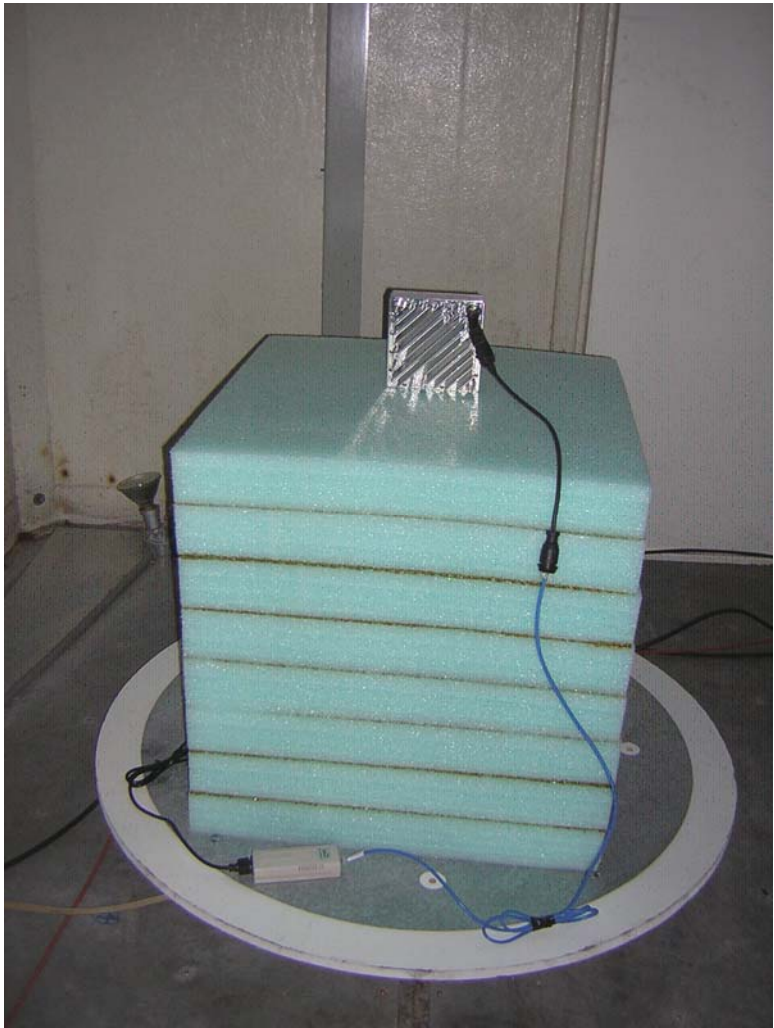
Radiated EMI
