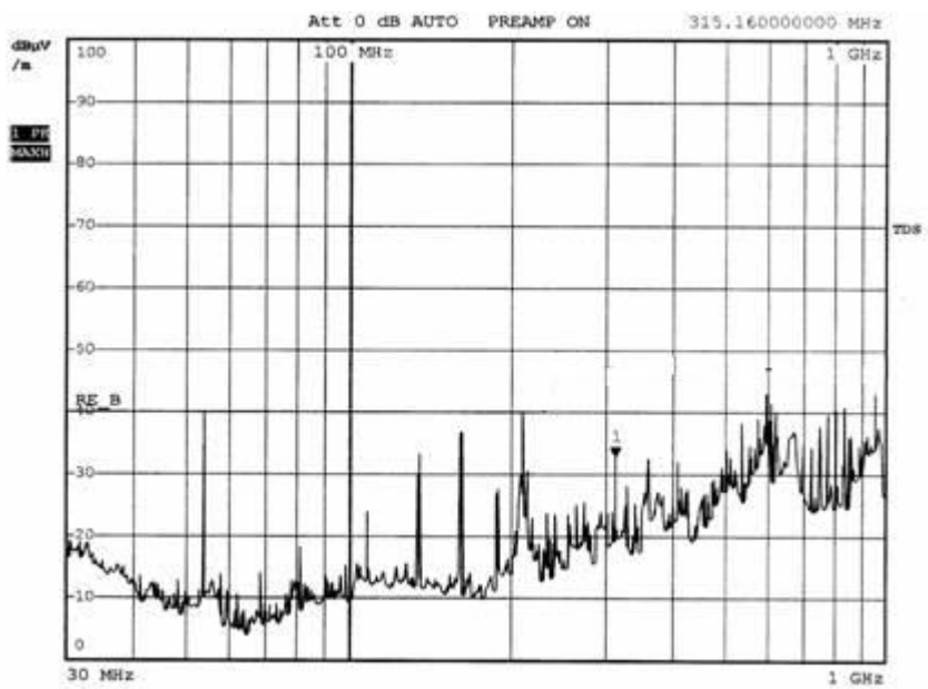
Vertical Radiated Emission Plot (Receiver)
