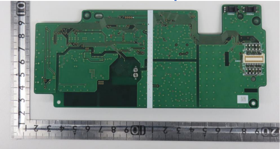
Sensor Board(back side)
