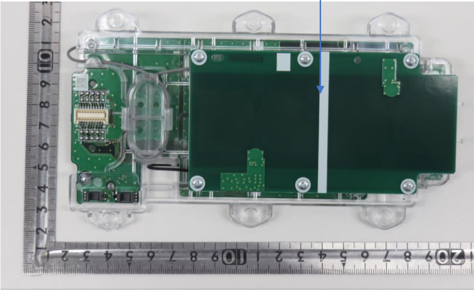
Antenna Board(back side)
