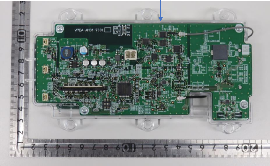
Sensor Board(back side)
