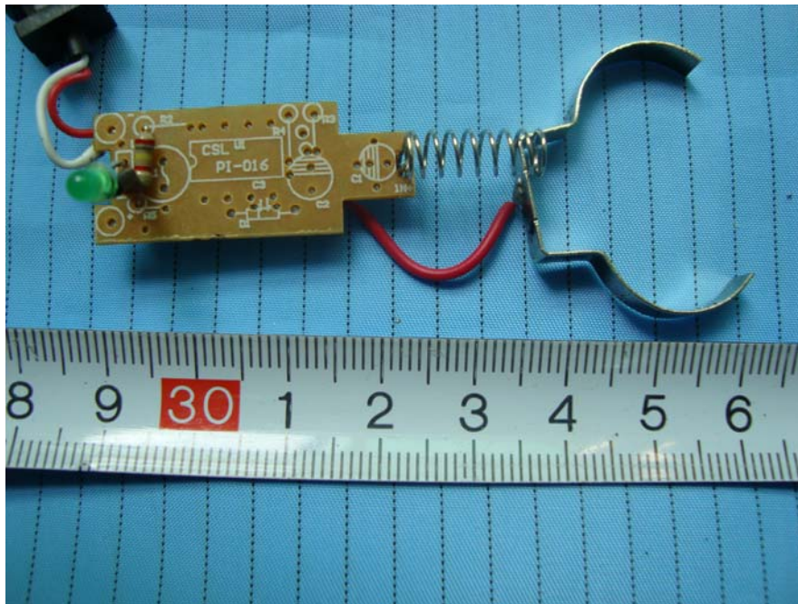
EUT – Power Socket Board Bottom View
