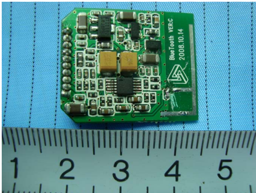
EUT – Bluetooth Board Top View
