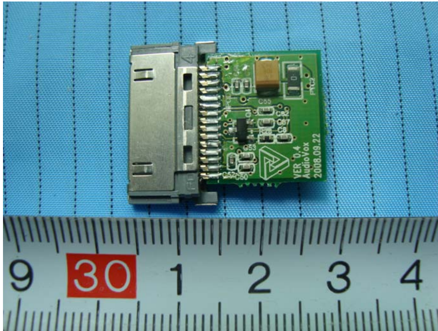
EUT – iPod Socket Board Bottom View
