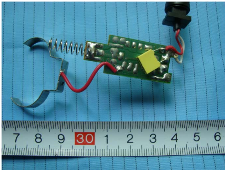
EUT – Power Socket Board Top View
