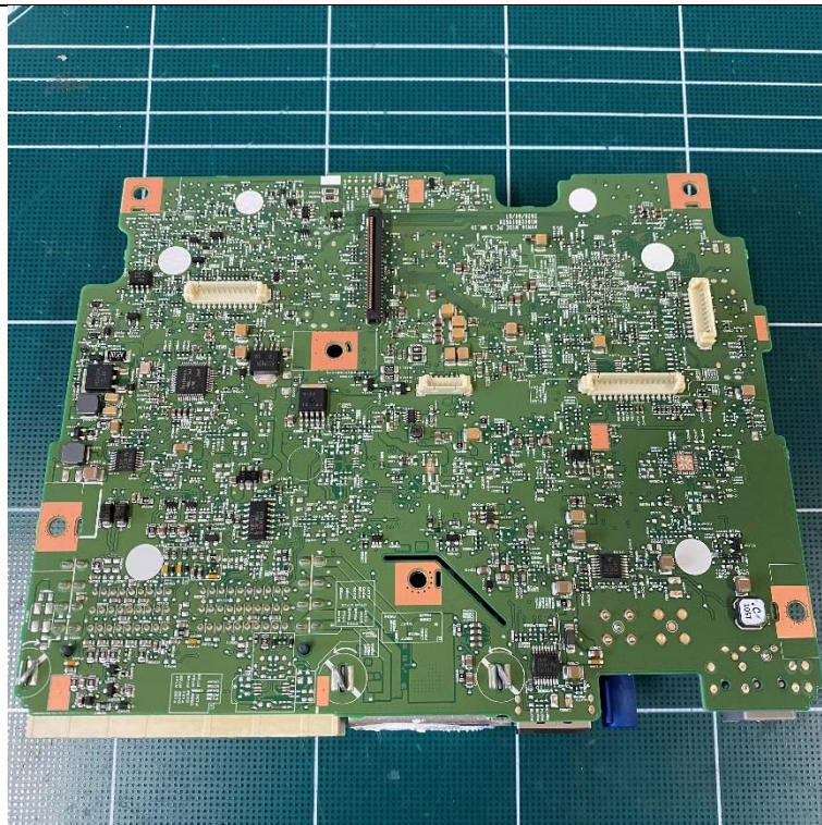
Bottom View of Main PCB
