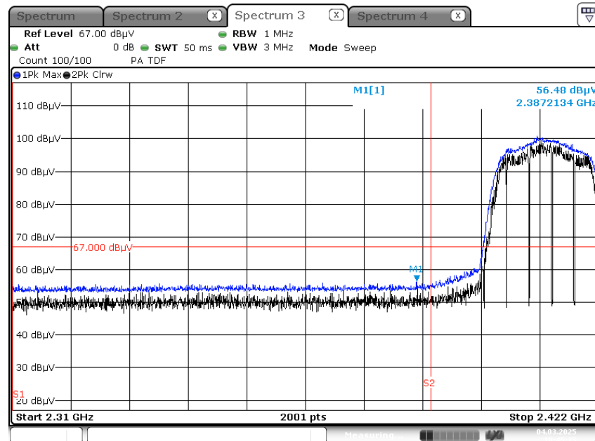
Radiated Restricted Band Edges plot – Peak Result (802.11n (HT20)_MCS0, Ch.1, X-V)
