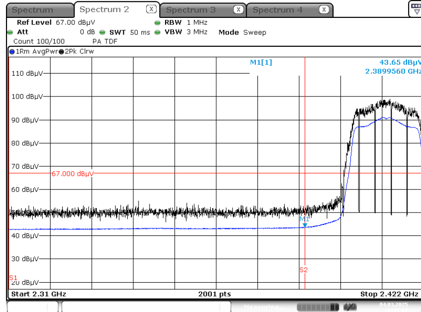
Radiated Restricted Band Edges plot – Average Result (802.11n (HT20)_MCS0, Ch.1, X-V)
