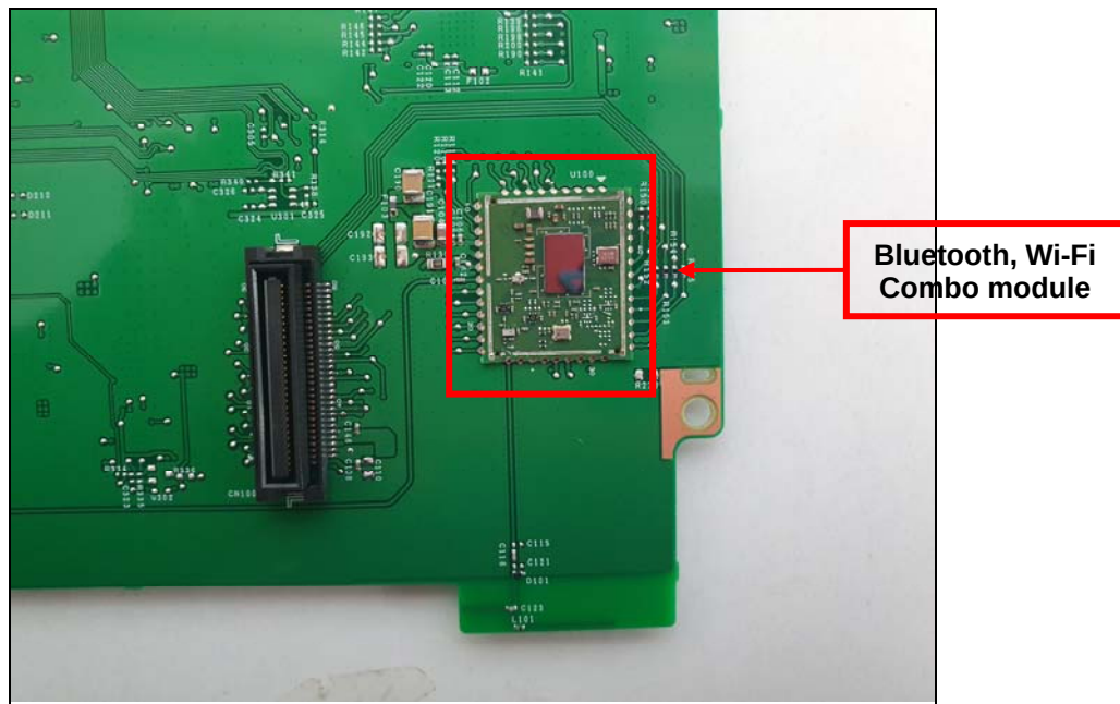
View of Bluetooth, Wi-Fi Combo module
