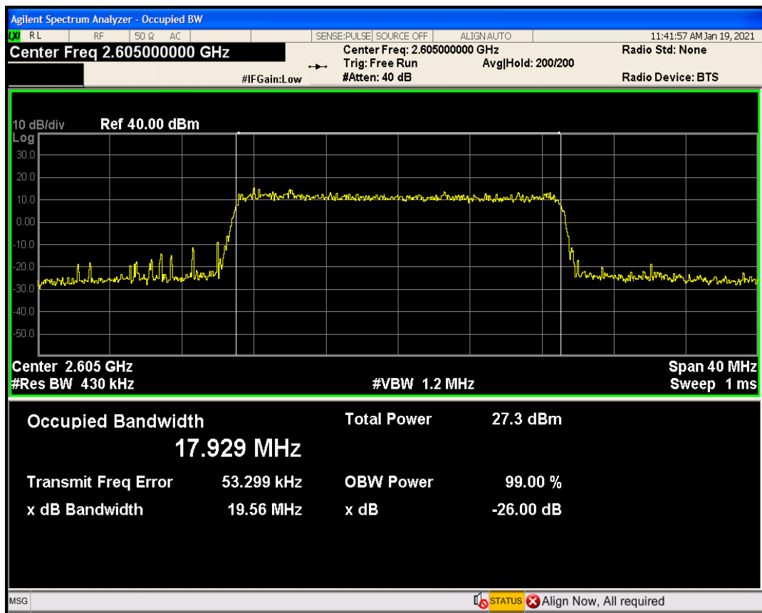
Band41a QAM16 BW=20MHz Channel=40740 RB Size=100 Position=#0
