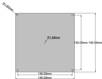
XC-AF620 Type antenna appearance dimension drawing
