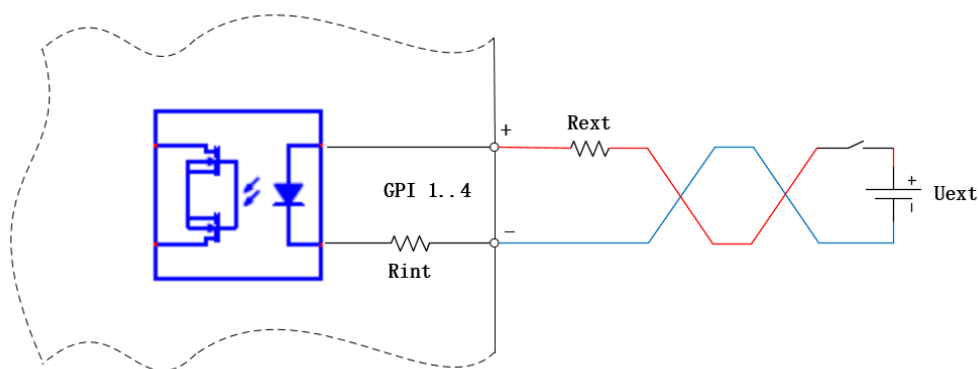
Fig.4-3: Internal and possible external wiring of the optocoupler inputs
