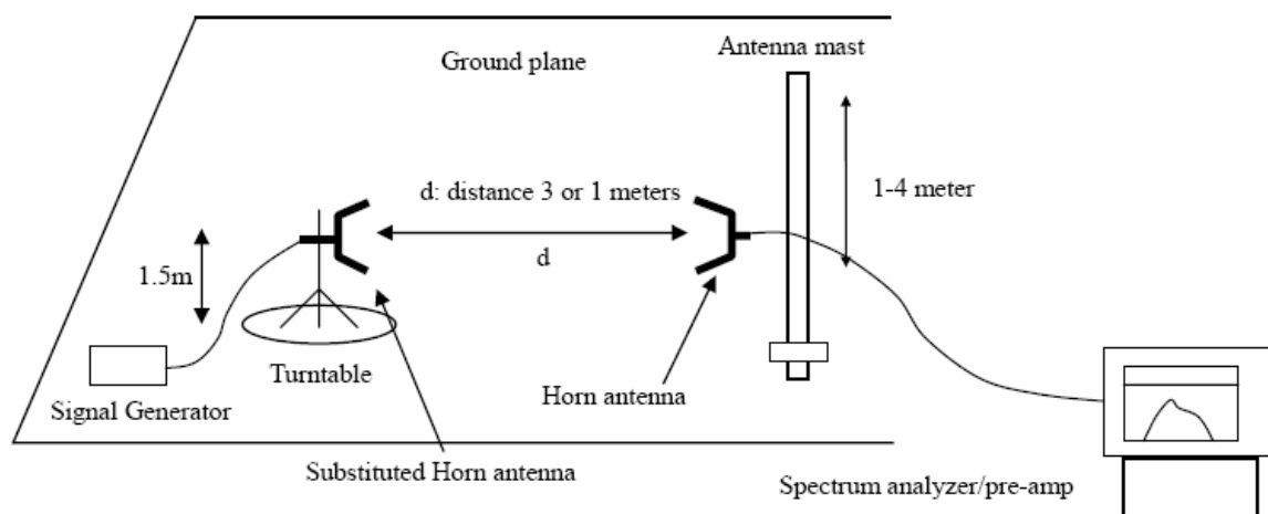
Radiation above 1GHz
