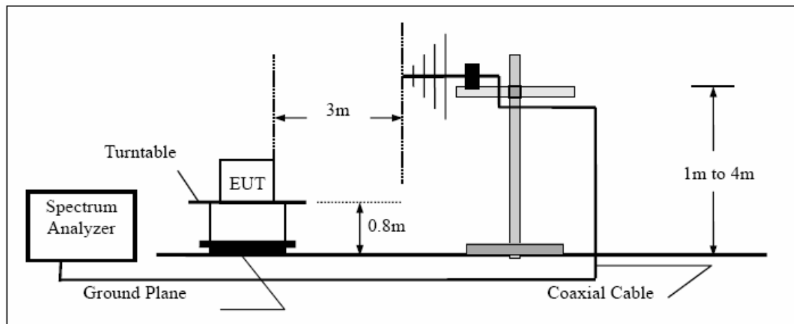
Radiation below 1GHz
