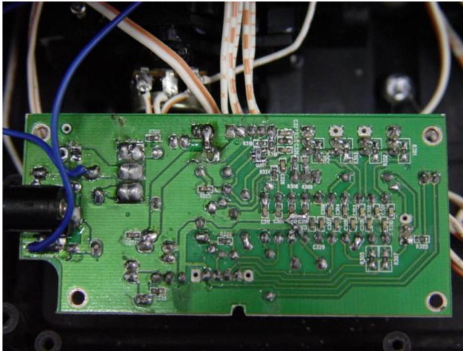
Photo 5 PCB photo
