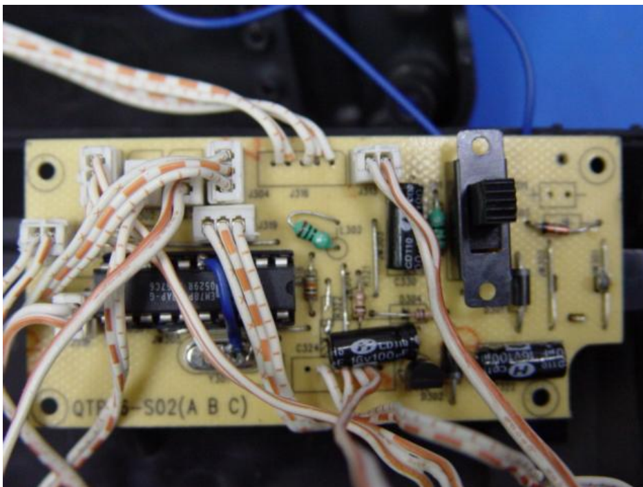
Photo 4 PCB photo
