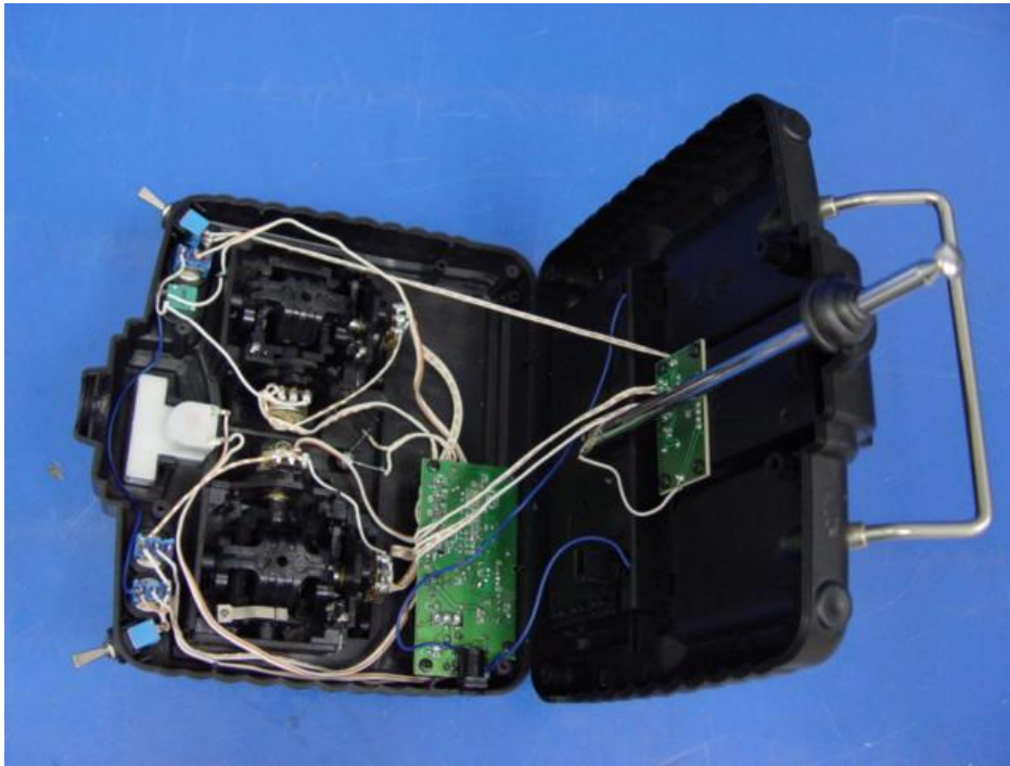
Photo 4 PCB photo
