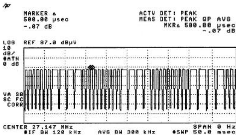
Figure C [Short Pulse]
