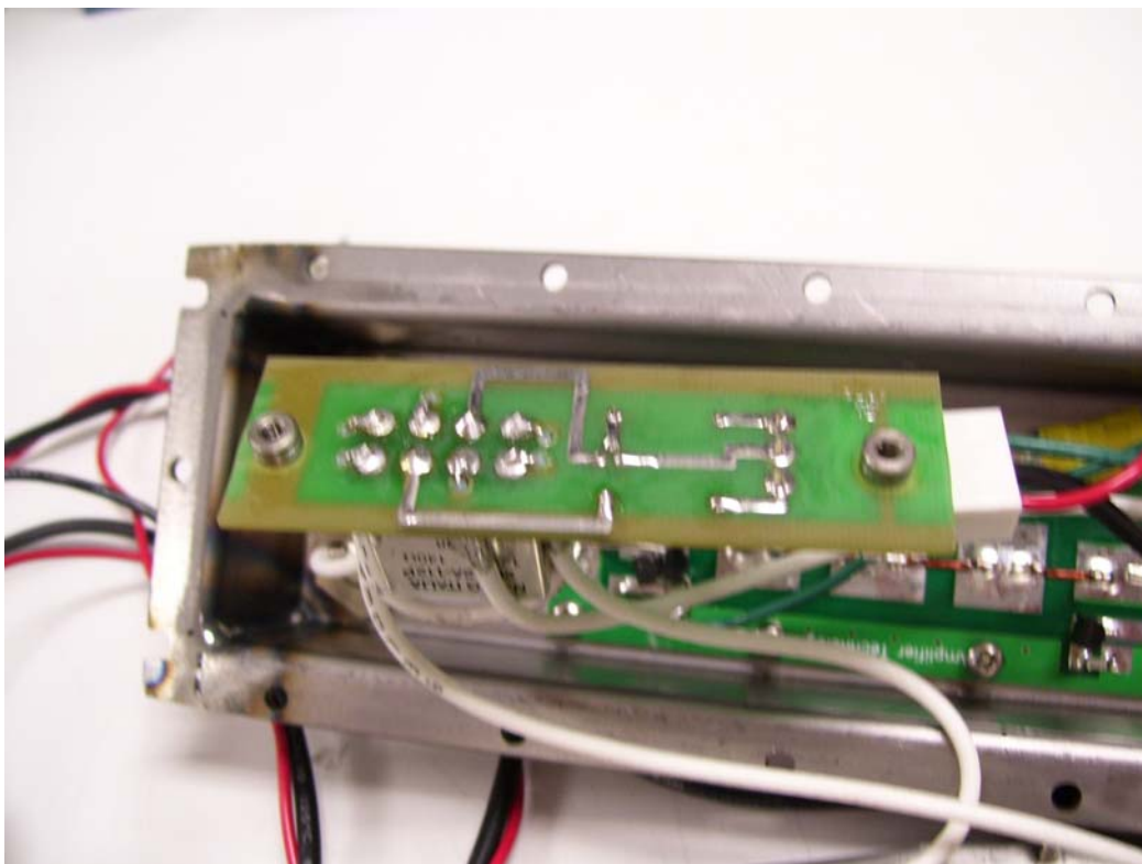
Figure 2 - Underside of PCB
