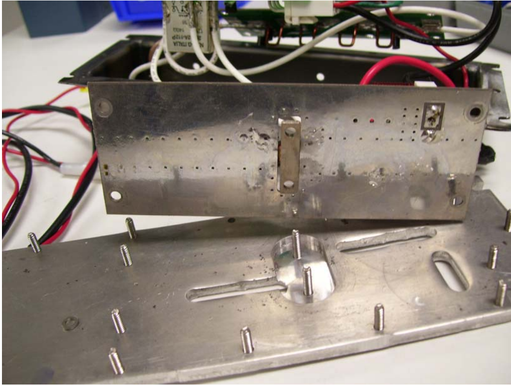
Figure 3 - Underside of PCB
