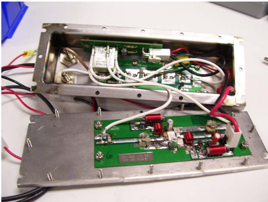
Figure 1 - Internal Photo
