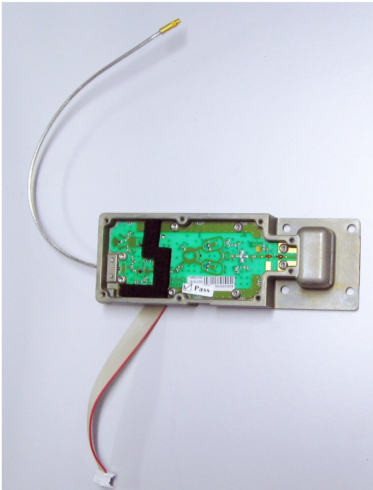
Figure 12 FE unit 3482 side 1
