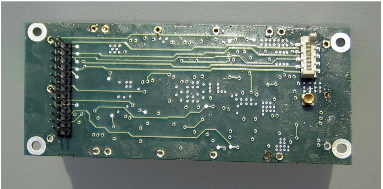
Figure 11 IF Board 3476 solder side
