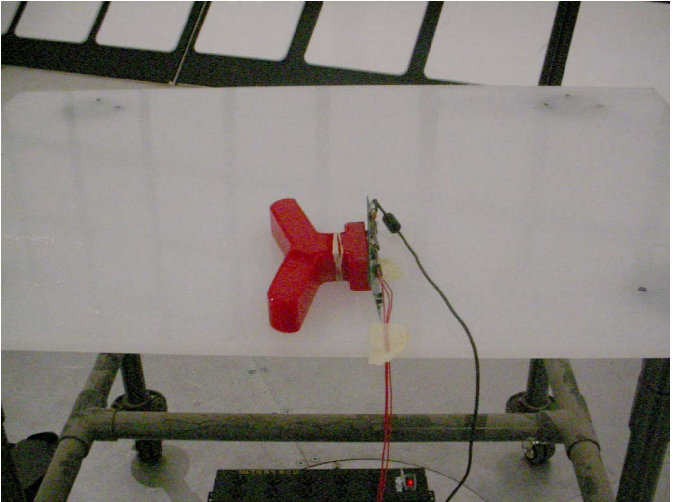
Radiated Emissions at 3 Meters EUT with Rigid Wire Antenna on Remote Control PCB
