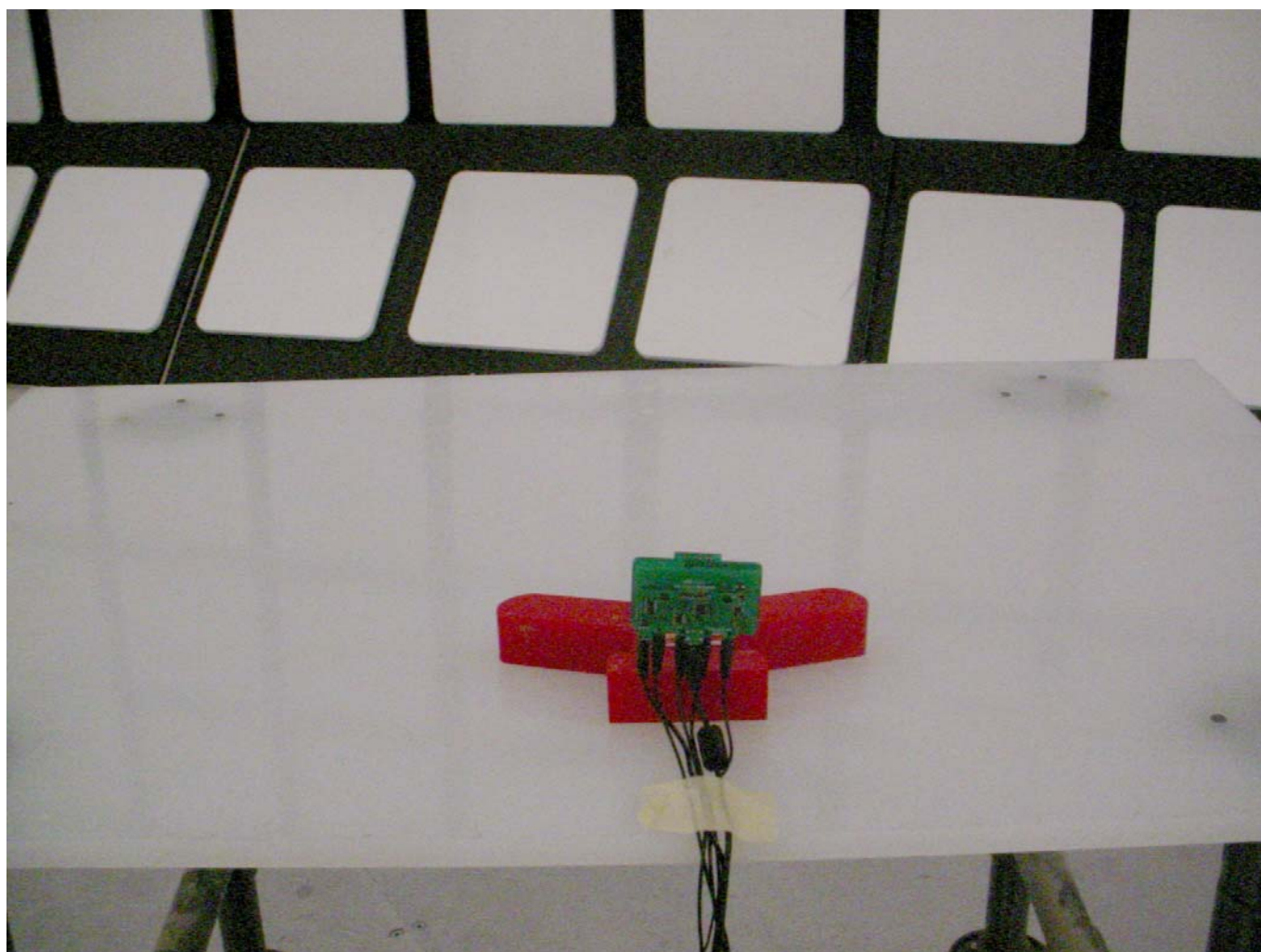
Radiated Emissions at 3 Meters EUT with Inverted F Antenna on Omnilink PCB
