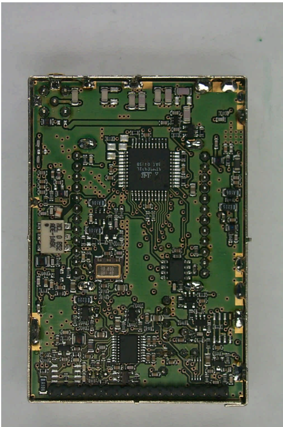
40893eut6.jpg: PCB, rear view
