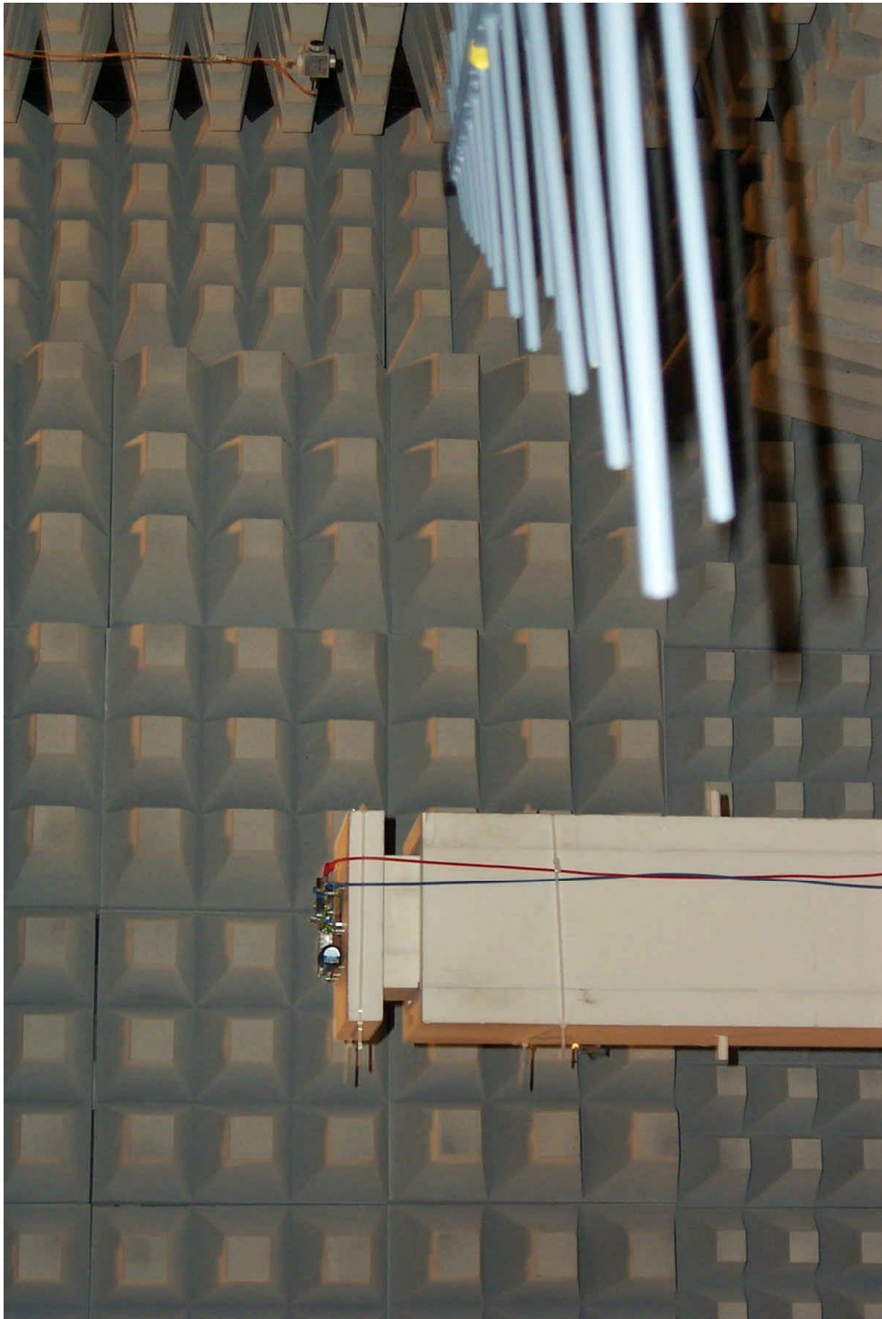
40893emi3.jpg: Test set-up radiated spurious emissions
