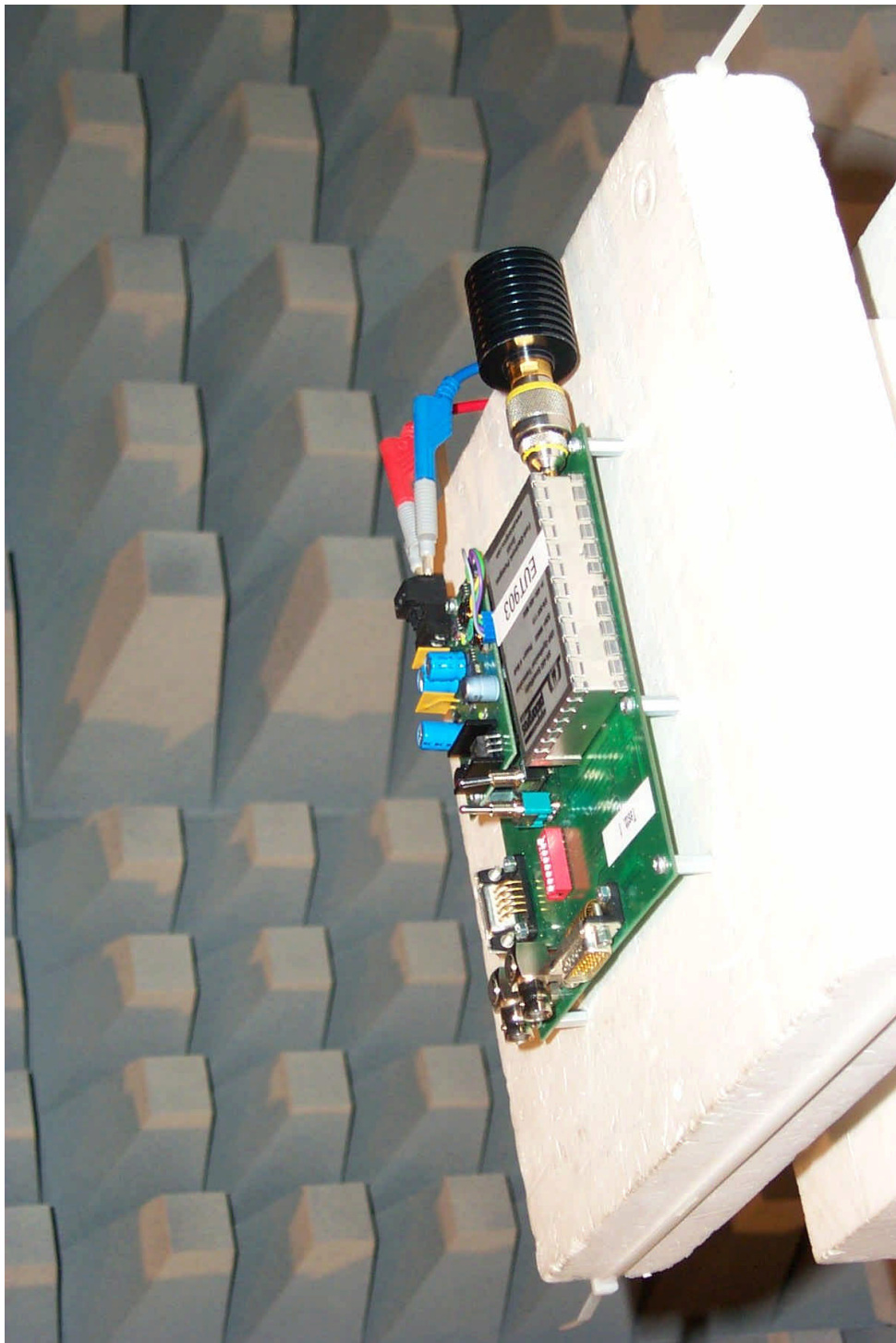
40893emi2.jpg: Test set-up radiated spurious emissions
