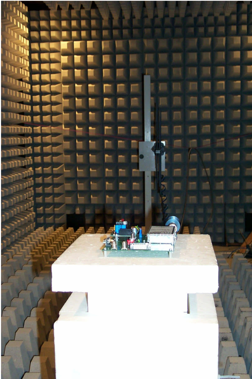
40893emi8.jpg: Test set-up radiated spurious emissions
