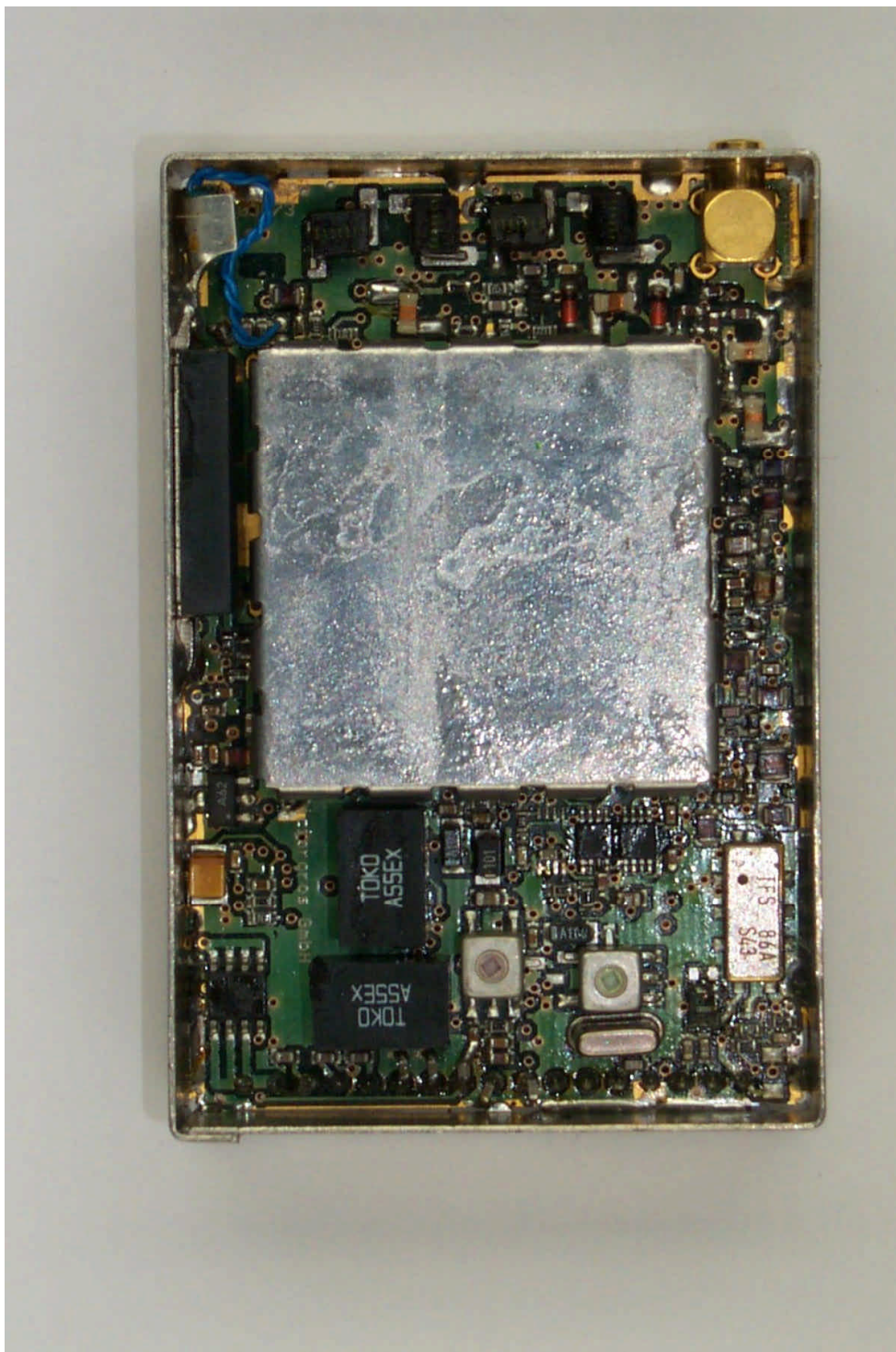
40893eut23.jpg: Main-PCB, front view
