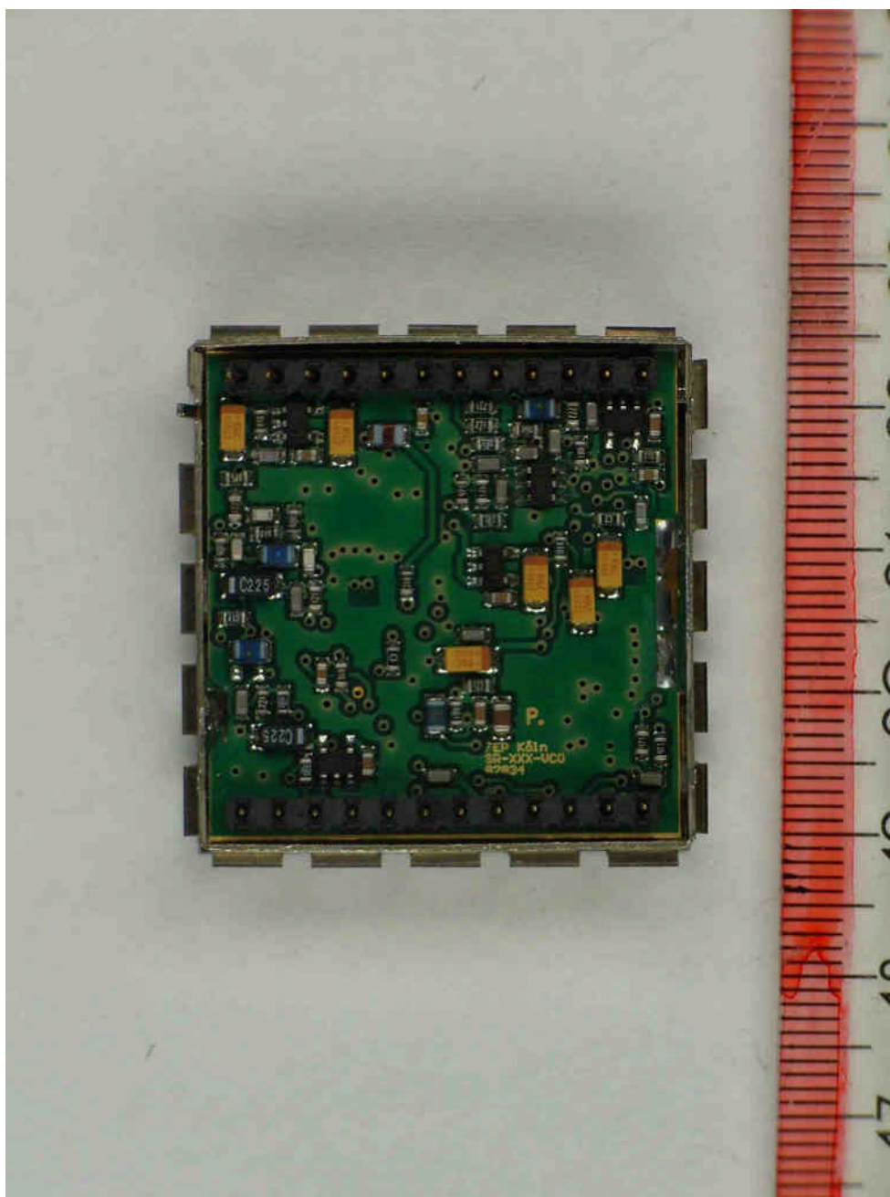
40893VCO3.jpg: VCO-PCB, front view
