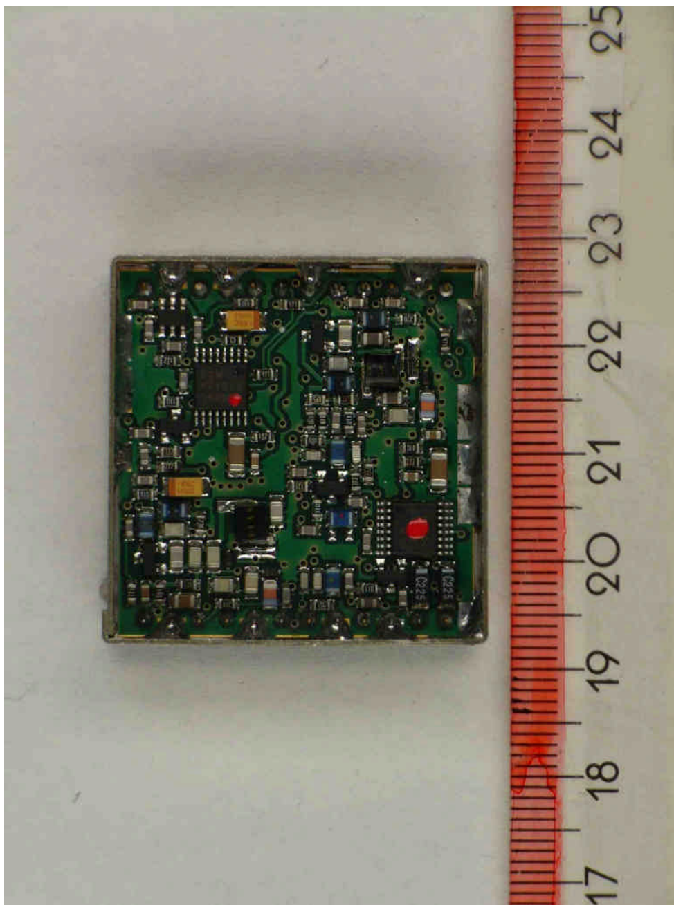
40893VCO1.jpg: VCO-PCB, rear view
