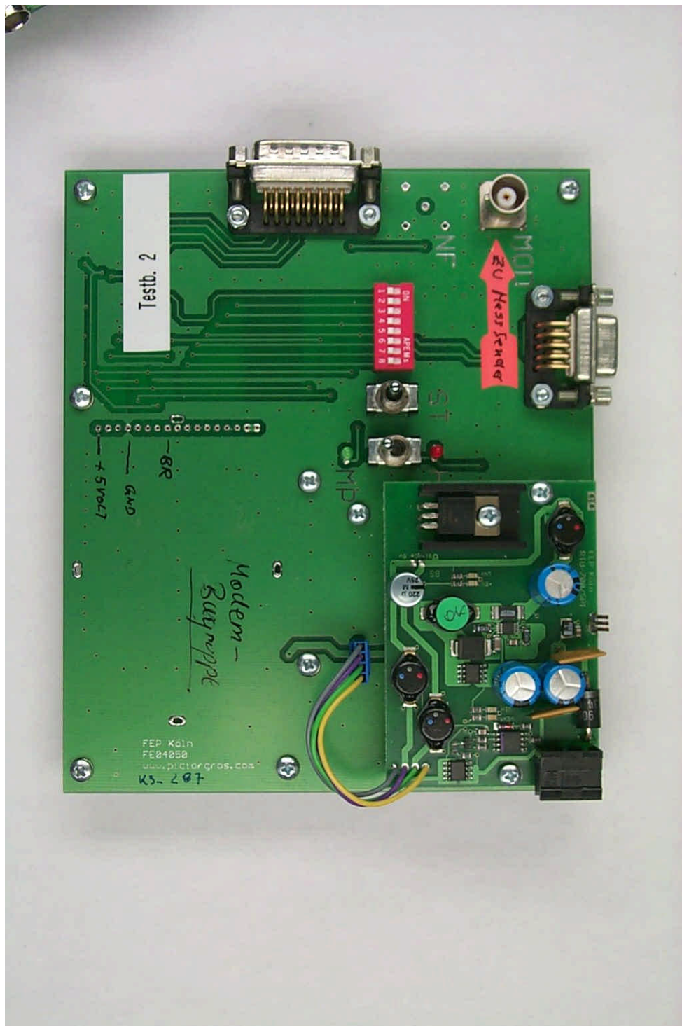
40893TB2.jpg: Test board 2
