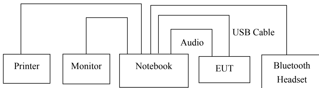
Fig. 2-1 Configuration of Tested System (AC Power Line Conducted Emission mode)
