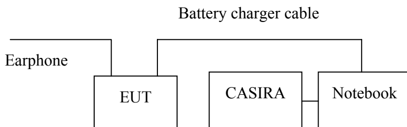
Fig. 2-1 Configuration of Tested System (Fixed channel)
