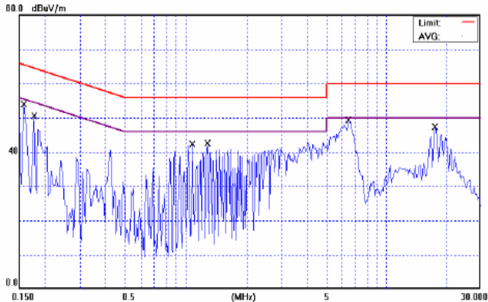
Conducted Emission Measurement
