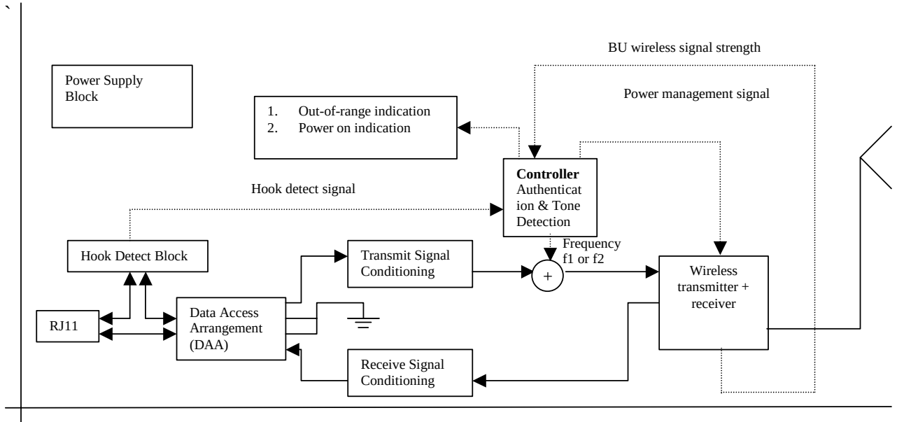
Figure 1: MU system block diagram
