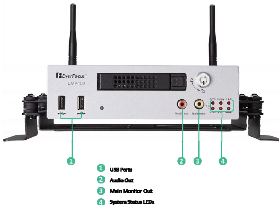
Figure 1-1 Front Panel
