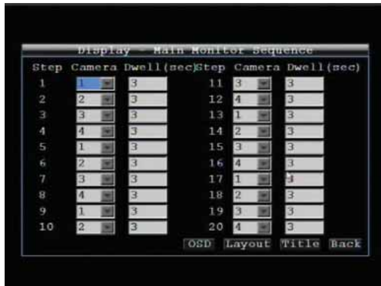
Figure 4-29 Display-Sequence
