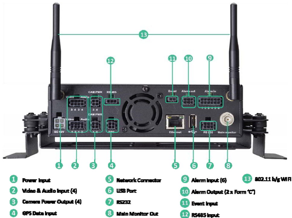
Figure 1-2 Rear Panel
