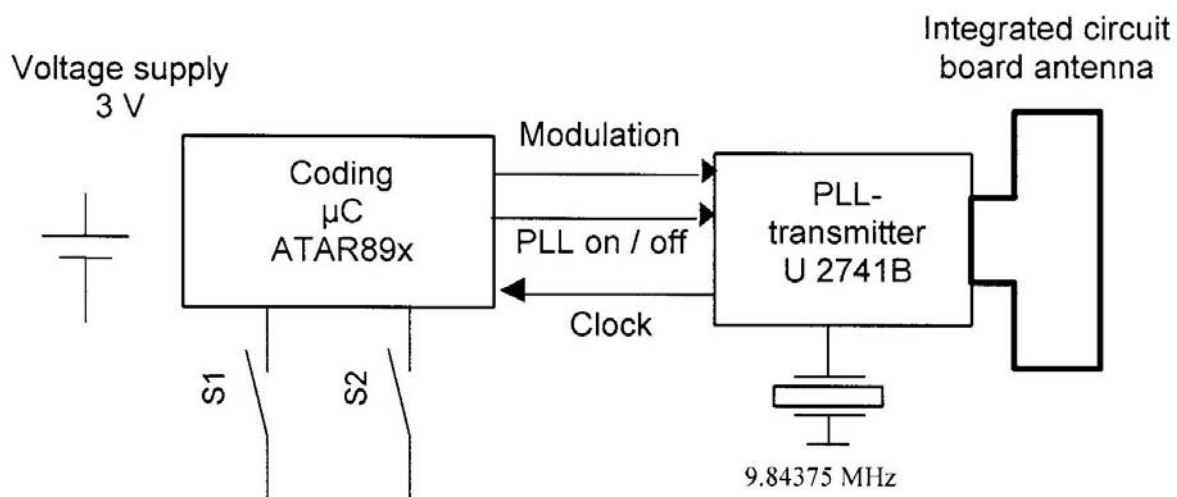
Figure 1: Block diagram of the transmitter
