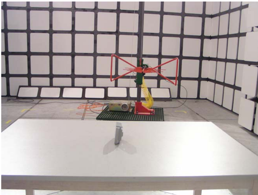
Radiated Emissions-Side View (2)
