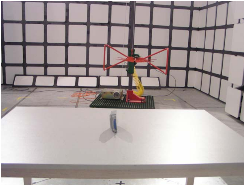
Radiated Emissions-Side View (1)
