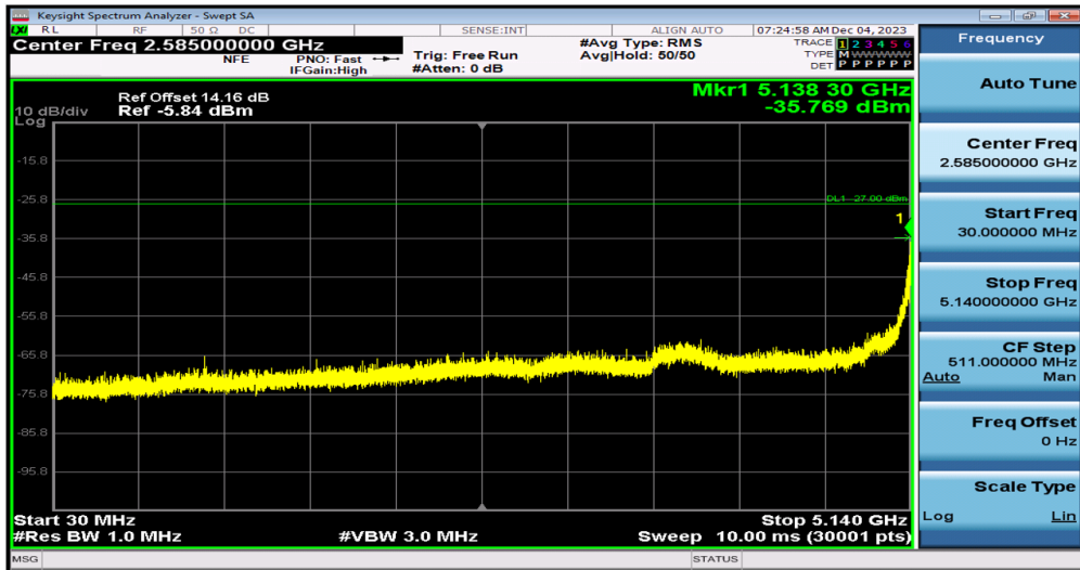
11N20MIMO-Ant0-5180-30~5140
