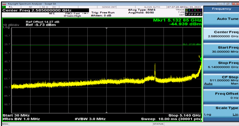
11N20MIMO-Ant1-5180-30~5140
