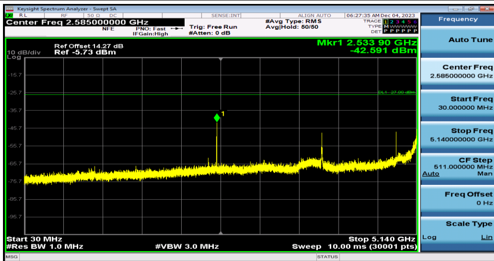
11A-Ant1-5200-30~5140
