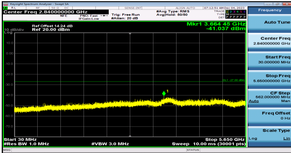
11A-Ant1-5825-30~5650
