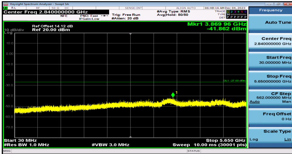
11A-Ant1-5745-30~5650
