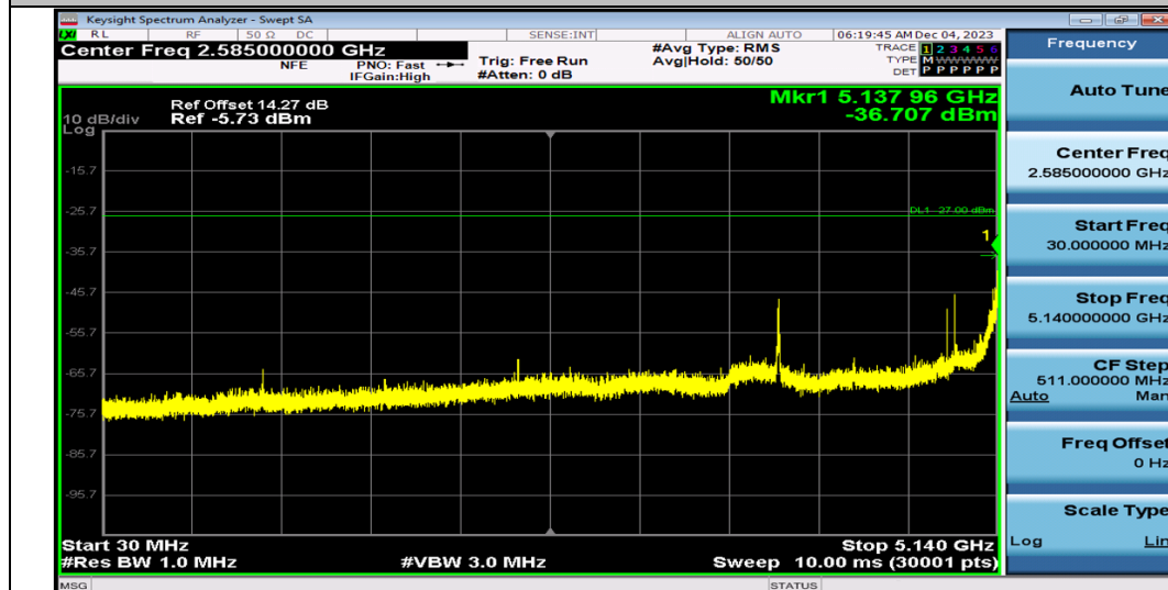
11A-Ant1-5180-30~5140
