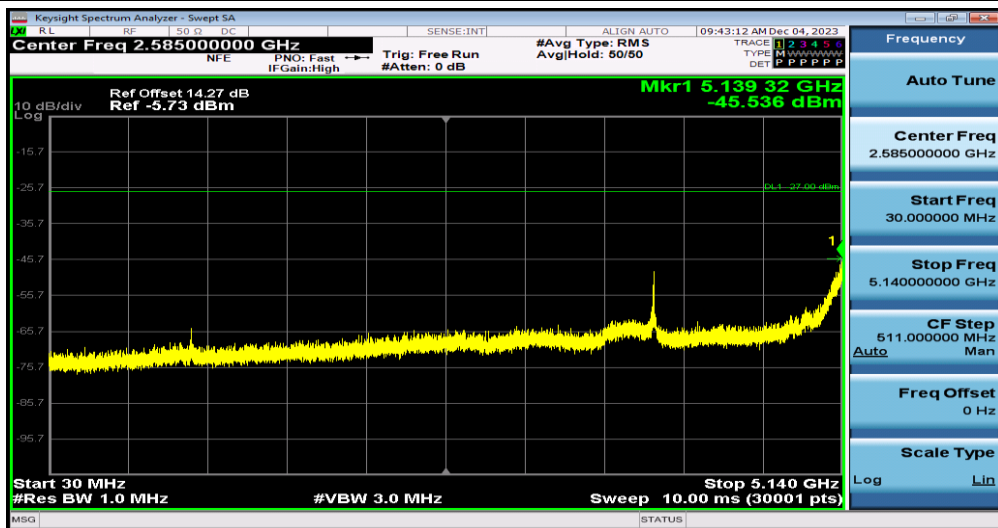
11N40MIMO-Ant1-5230-30~5140
