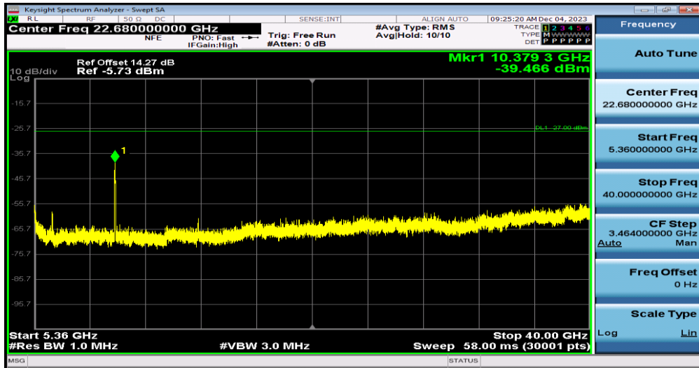
11N40MIMO-Ant1-5190-5360~40000
