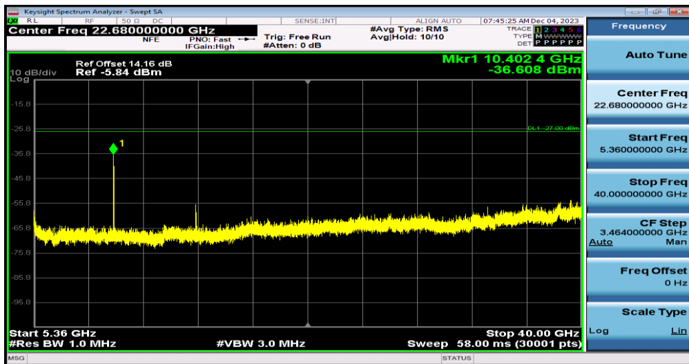
11N20MIMO-Ant0-5200-5360~40000
