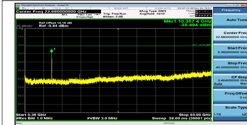
11A-Ant0-5180-5360~40000
