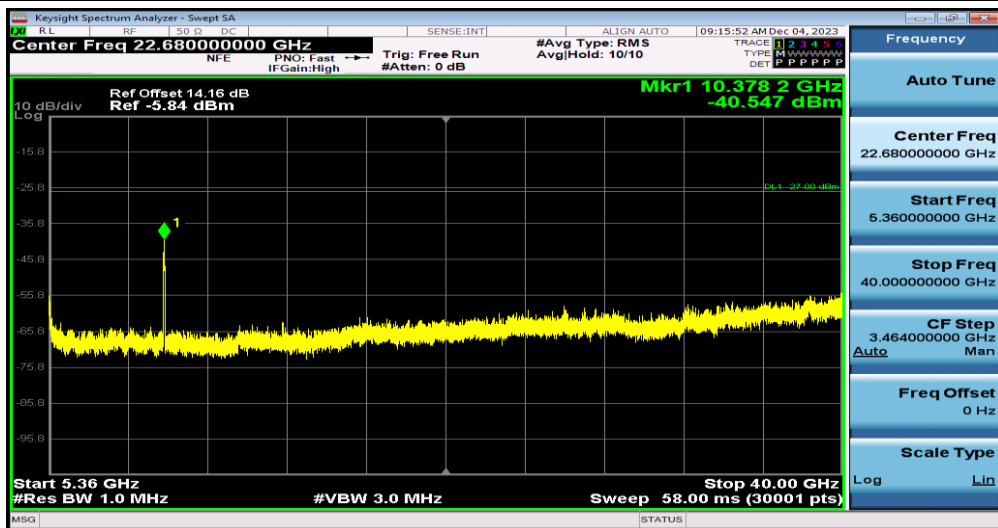
11N40MIMO-Ant0-5190-5360~40000
