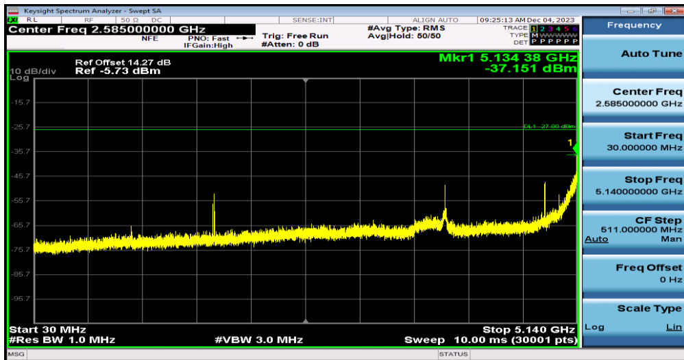
11N40MIMO-Ant1-5190-30~5140
