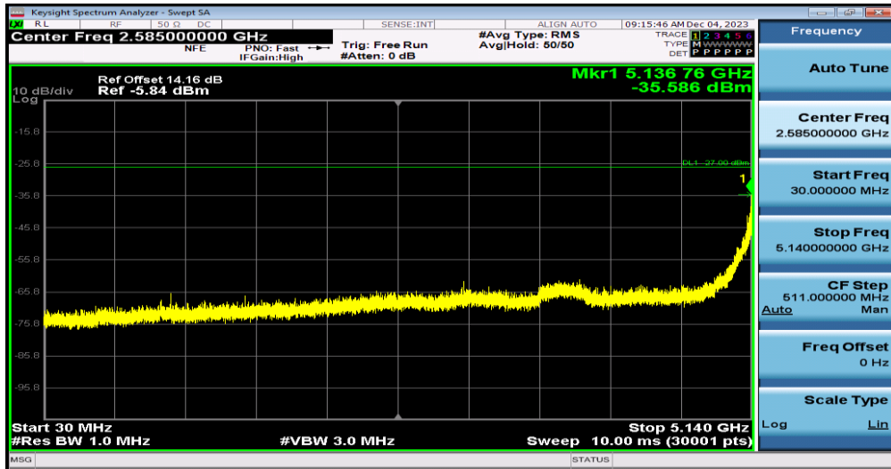
11N40MIMO-Ant0-5190-30~5140
