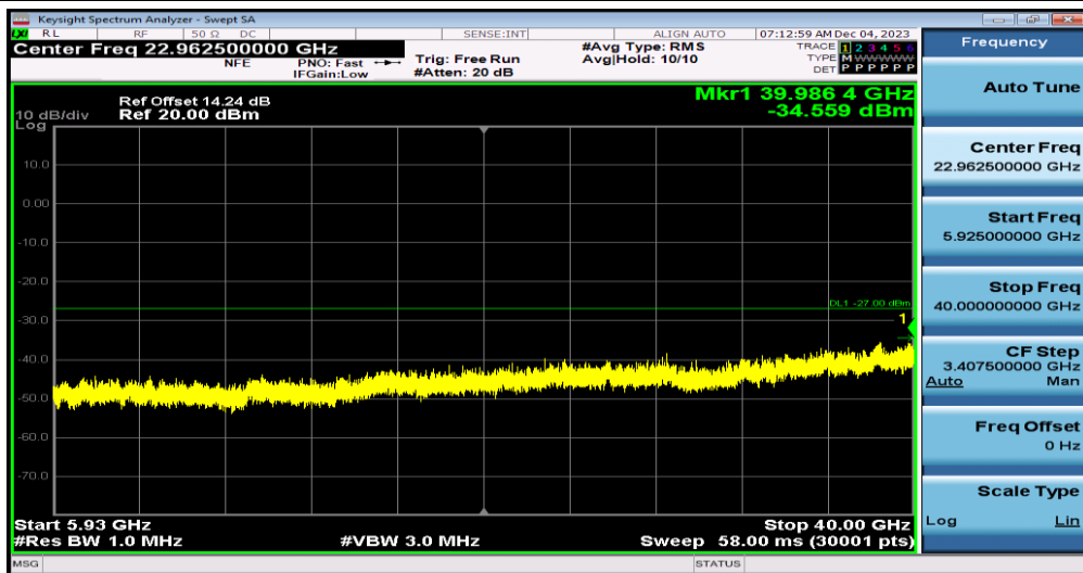
11A-Ant1-5825-5925~40000
