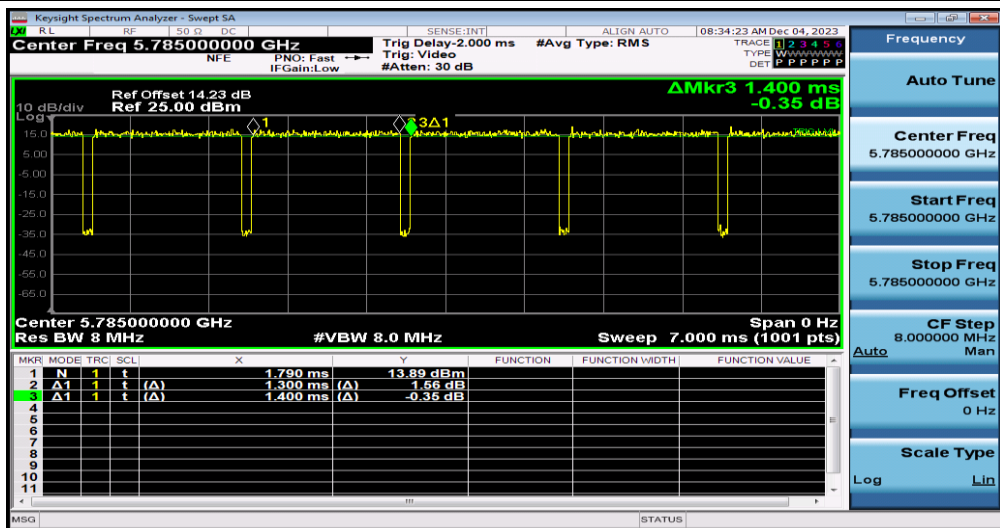
NTNV-11N20MIMO-Ant0-5785
