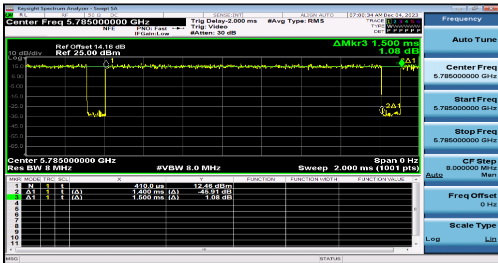
NTNV-11A-Ant1-5785
