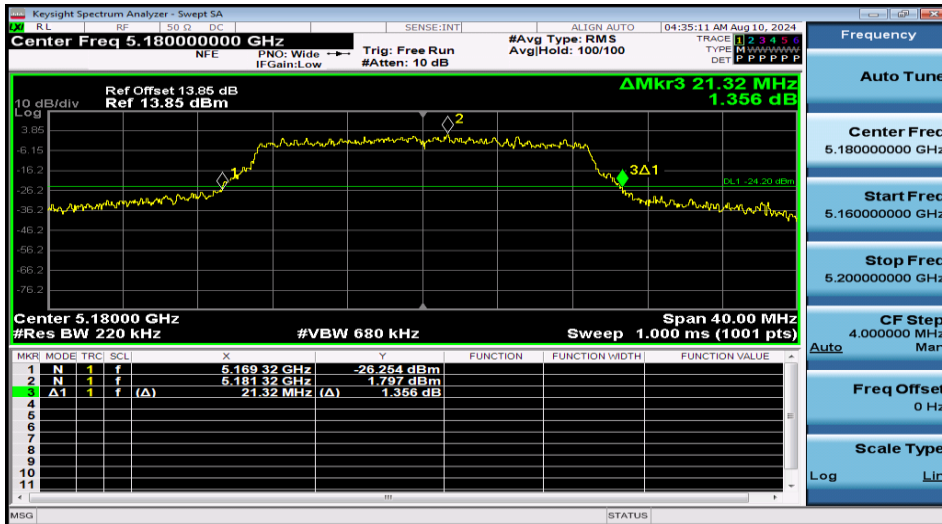
11N20MIMO-Ant2-5180
