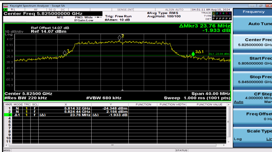
11N20MIMO-Ant2-5825
