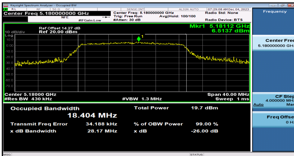
11N20MIMO-Ant1-5180
