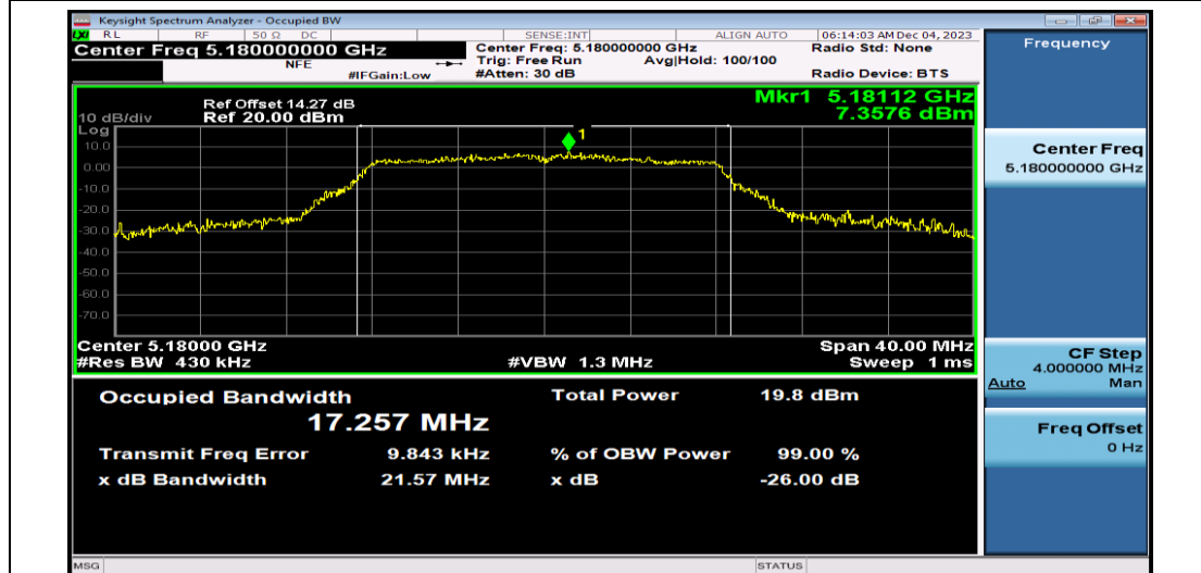
11A-Ant1-5180
