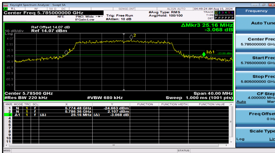
11N20MIMO-Ant2-5785
