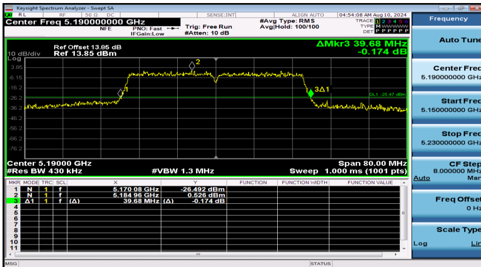
11N40MIMO-Ant2-5190
