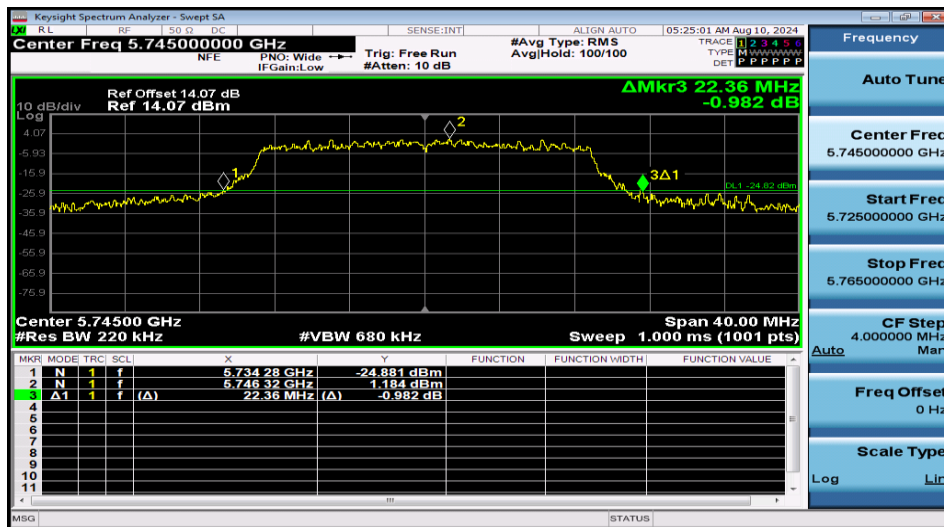
11N20MIMO-Ant2-5745
