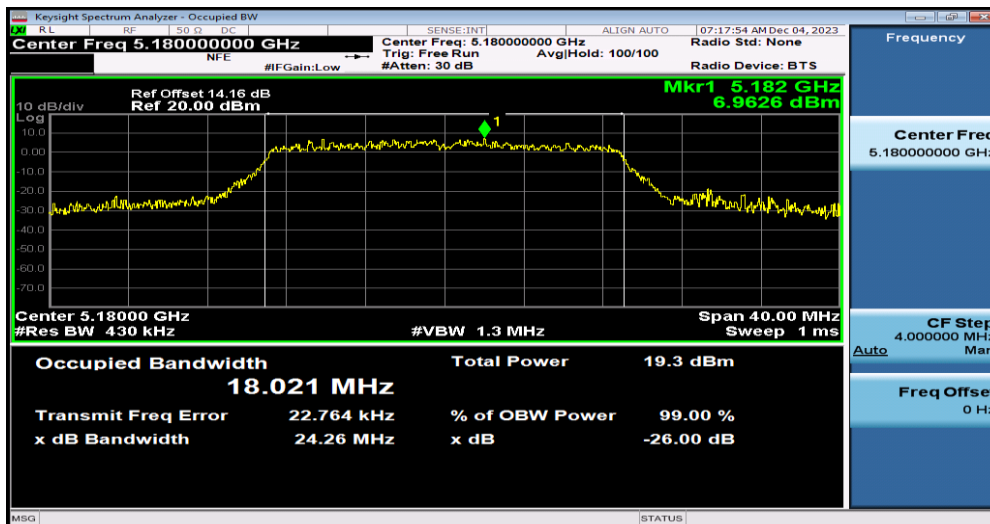
11N20MIMO-Ant0-5180
