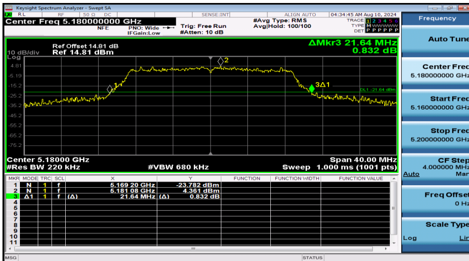
11N20MIMO-Ant1-5180
